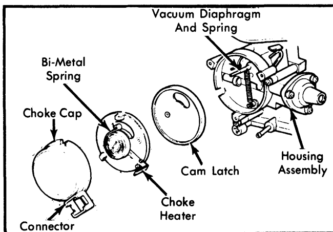
Fig. 2 Constant Operating Type Electric Assist Choke
