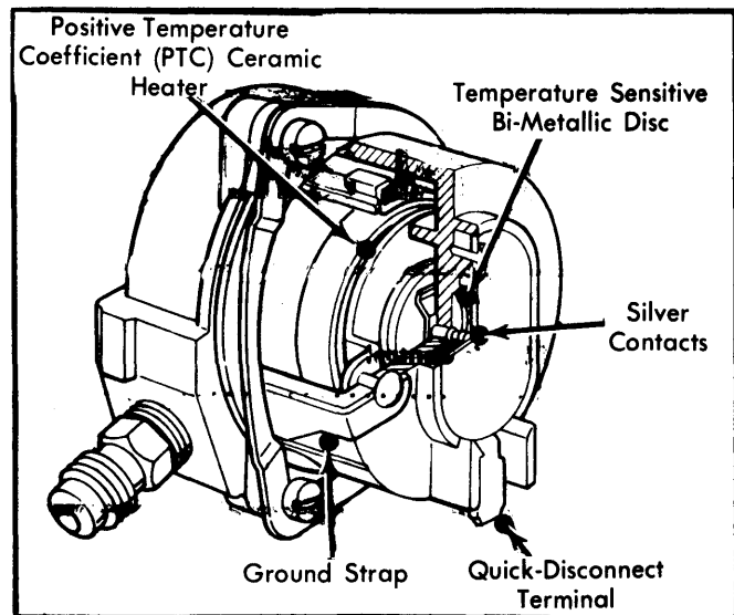
Fig. 1 Temperature Sensitive Type Electric Assist Choke
