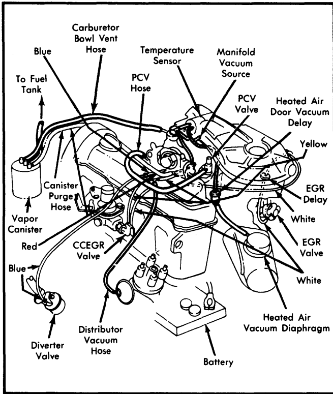
Fig. 1 1.7 Liter; Federal
