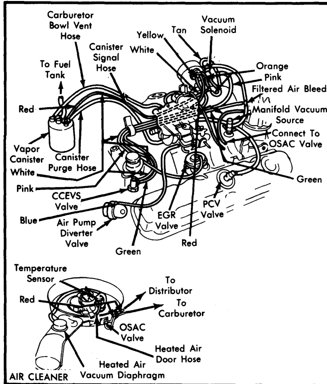
Fig. 5 318" 2-Bbl; Federal
