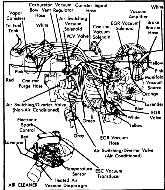
Fig. 4 225" 1-Bbl.; California
