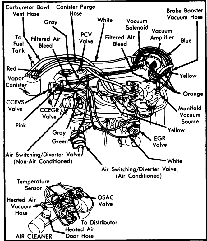
Fig. 3 225" 1-Bbl.; Federal
