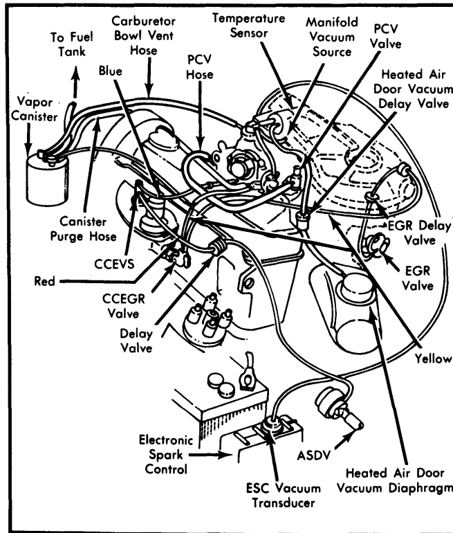
Fig. 2 1.7 Liter; California
