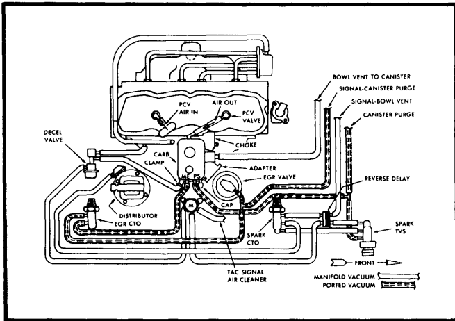
Fig. 1 151" 4-Cyl. Federal Man. Trans. (AMX, Concord and Spirit)
