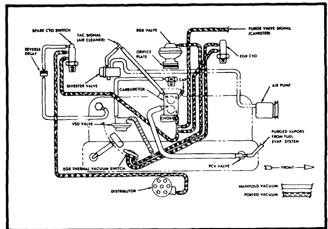
Fig. 11 258" 6-Cyl. Federal with 3.54 Axle (Eagle Models Only)
