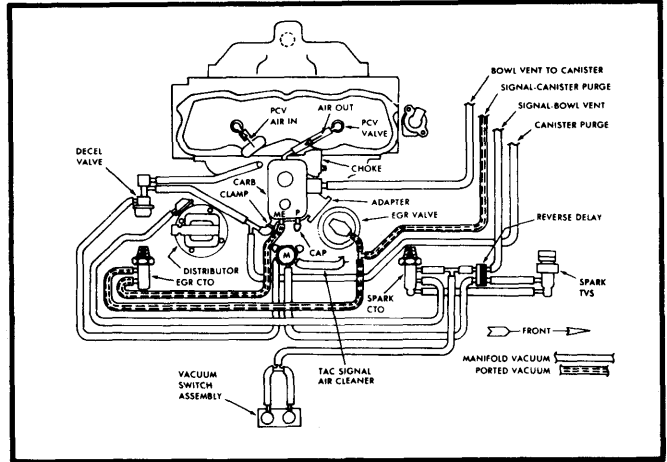
Fig. 4 151" 4-Cyl. Calif. Man. Trans. (AMX, Concord and Spirit)
