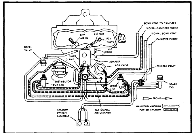
Fig. 5 151" 4-Cyl. Calif. Auto. Trans. (AMX, Concord and Spirit)
