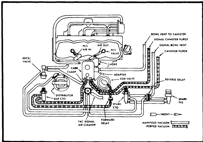
Fig. 2 151" 4-Cyl. Federal Auto. Trans. Without A/C (AMX, Concord and Spirit)
