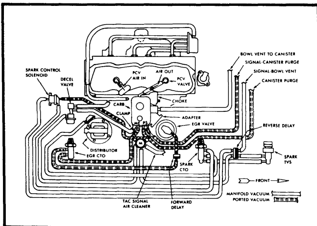
Fig. 3 151" 4-Cyl. Federal Auto. Trans. With A/C (AMX, Concord and Spirit)
