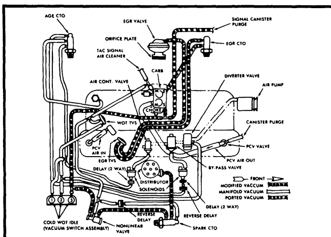
Fig. 9 258" 6-Cyl. Calif. Auto. Trans. (AMX, Concord and Spirit)
