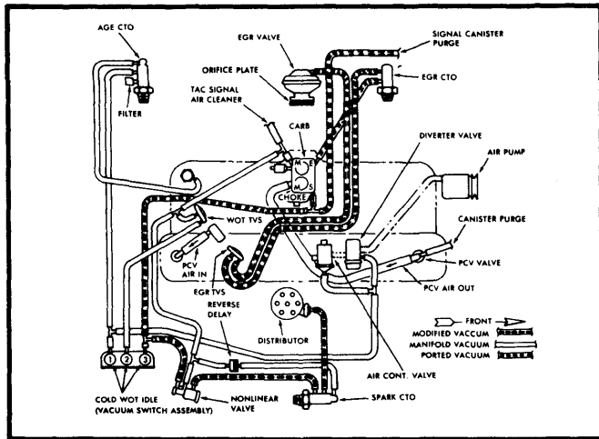
Fig. 7 258" 6-Cyl. Federal Auto. Trans. (AMX, Concord and Spirit)
