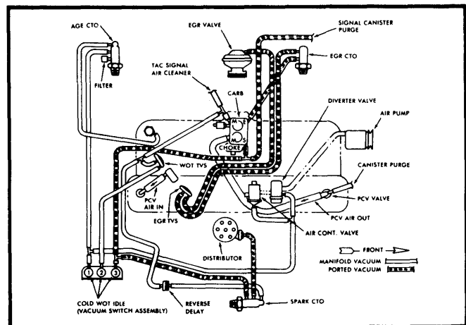
Fig. 6 258" 6-Cyl. Federal Man. Trans. (AMX, Concord and Spirit)
