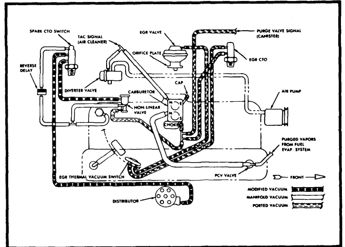
Fig. 10 258" 6-Cyl. Federal with 3.08 Axle (Eagle Models Only)
