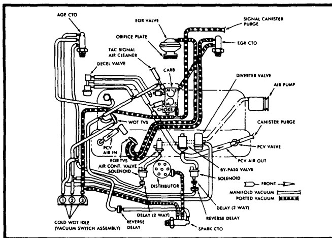
Fig. 8 258" 6-Cyl. Calif. Man. Trans. (AMX, Concord and Spirit)
