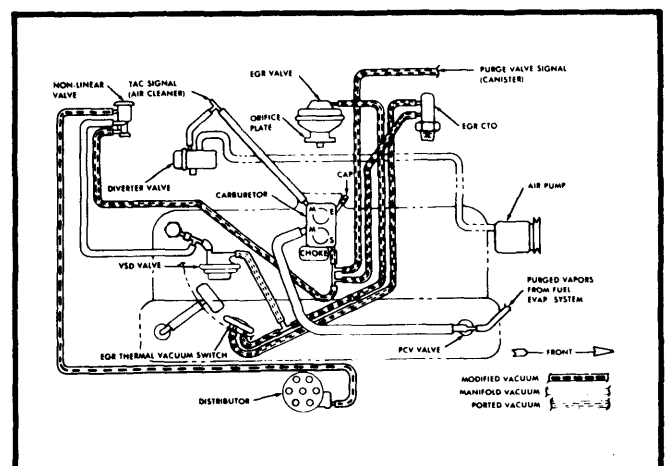
Fig. 12 258" 6-Cyl. Calif. and Hilly Terrain (Eagle Models Only)
