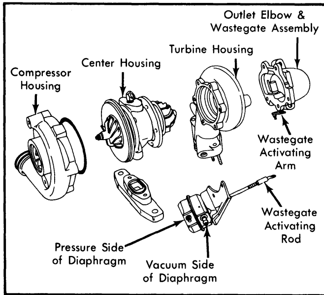
Fig. 2 Turbocharger Components
