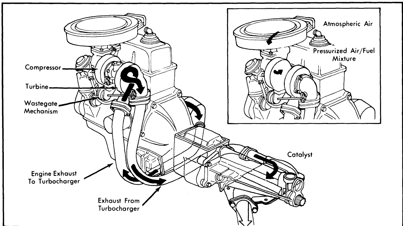
Fig.1 Ford Motor Co. Turbocharging System
