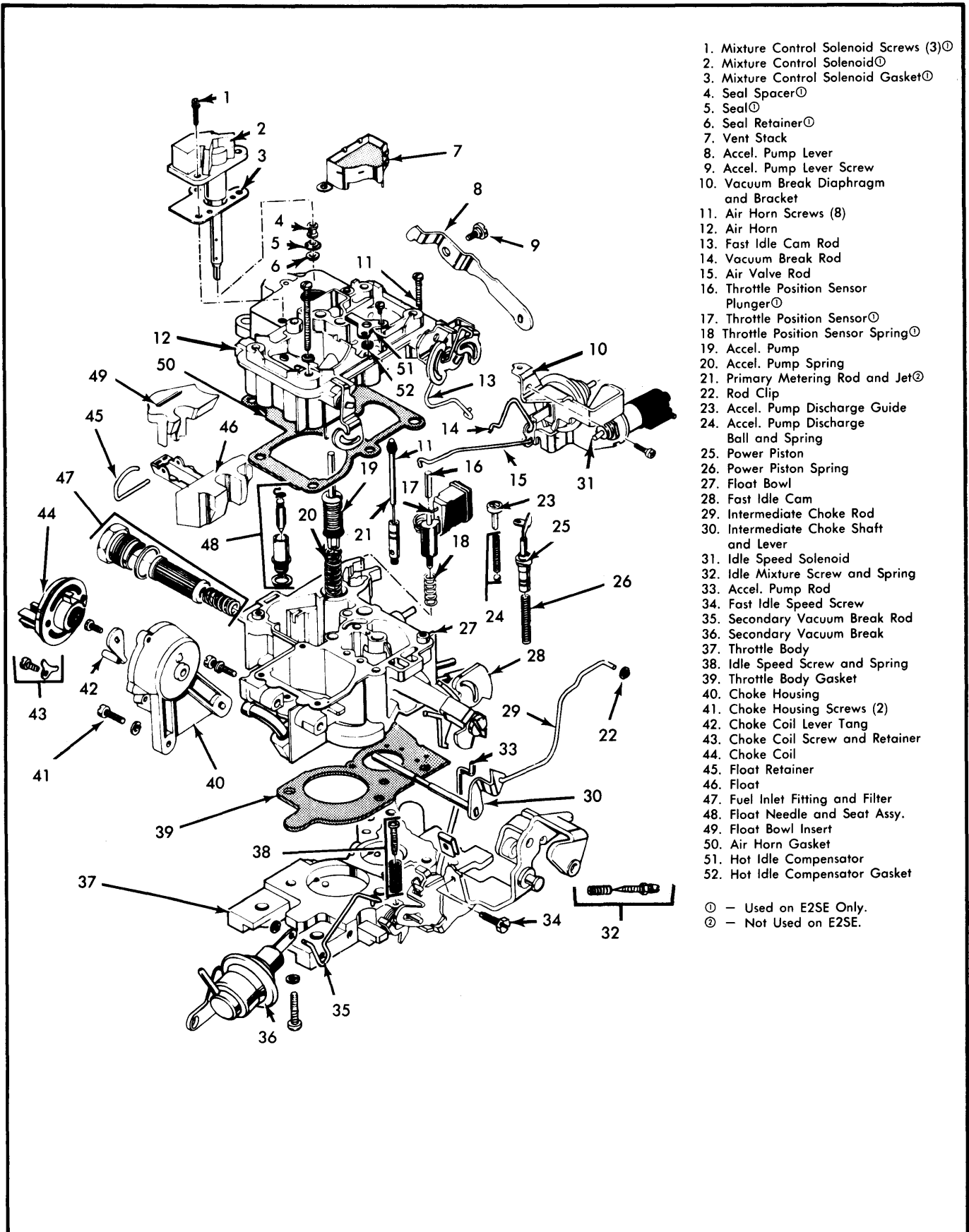
Fig. 12 Exploded View of Rochester Model 2SE and E2SE 2-Barrel Carburetor (6 CYLINDER MODELS)
