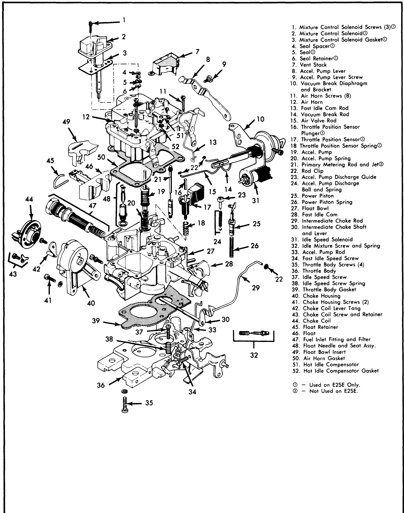
Fig. 11 Exploded View of Rochester Model 2SE and E2SE 2-Barrel Carburetor (4 CYLINDER MODELS)
