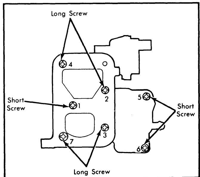
Fig. 10 Air Horn Screw Location and Tightening Sequence
