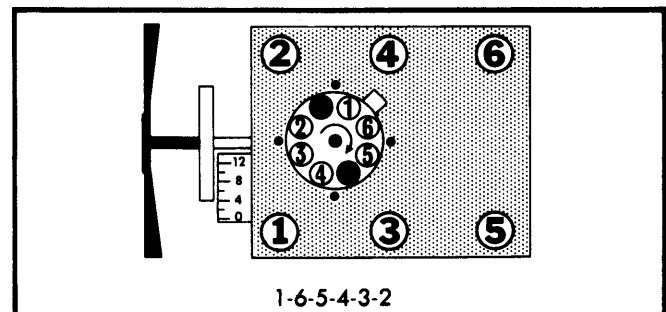
Fig. 2 231" Firing Order and Timing Marks
