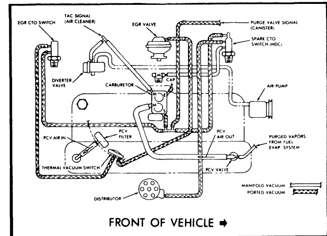
Fig. 6 258" 6 Cyl. California Manual Transmission "CJ" Models With Heavy Duty Cooling
