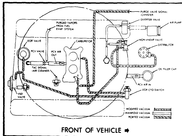
Fig. 17 360" V8 California Manual Transmission "J" Models
