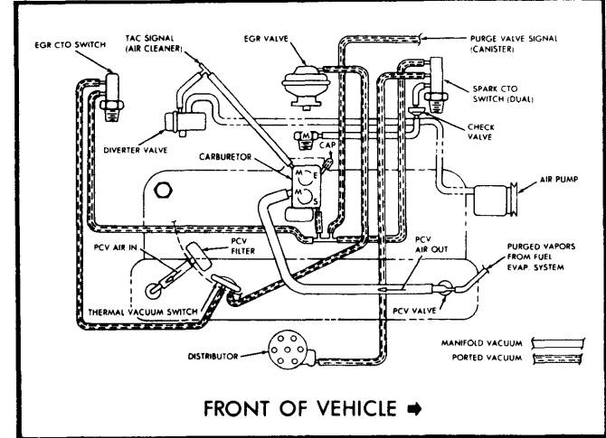
Fig. 4 258" 6 Cyl. Federal Automatic Transmission All Models With Heavy Duty Cooling
