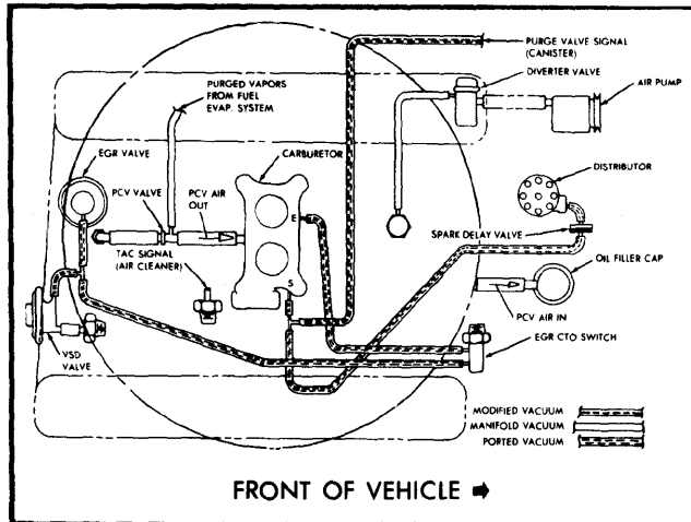
Fig. 15 360" V8 California Manual Transmission Cherokee Models
