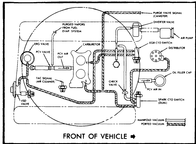
Fig. 22 360" V8 California Automatic Transmission Cherokee, Wagoneer and "J" Models With Heavy Duty Cooling
