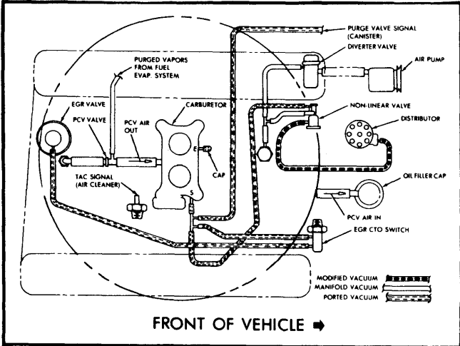
Fig. 9 304" V8 Federal Manual Transmission "CJ" Models
