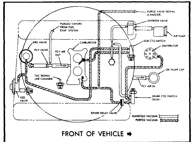
Fig. 16 360" V8 California Manual Transmission Cherokee Models With Heavy Duty Cooling
