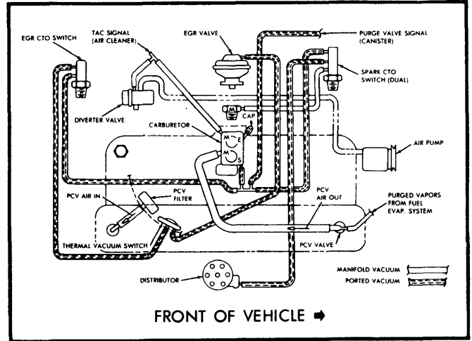
Fig. 2 258" 6 Cyl. Federal Manual Transmission All Models With Heavy Duty Cooling
