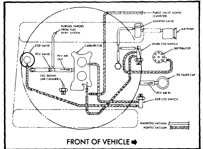
Fig. 14 360" V8 Federal Automatic Transmission Cherokee, Wagoneer and "J" Models
