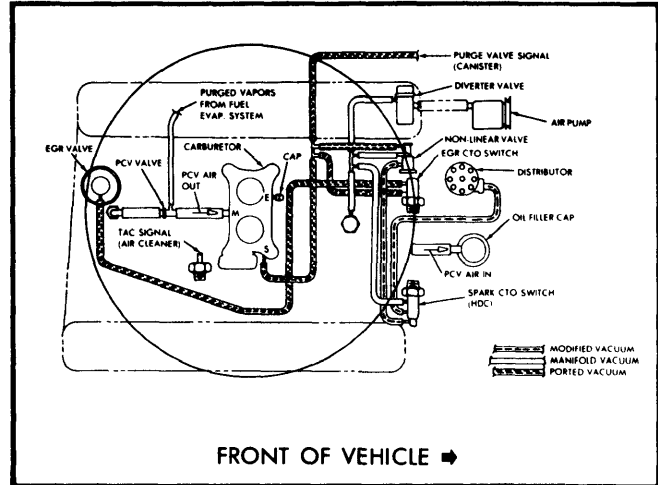
Fig. 10 304" V8 Federal Manual Transmission "CJ" Models With Heavy Duty Cooling
