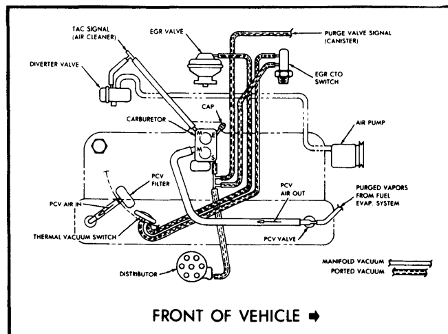
Fig. 5 258" 6 Cyl. California Manual Transmission "CJ" Models
