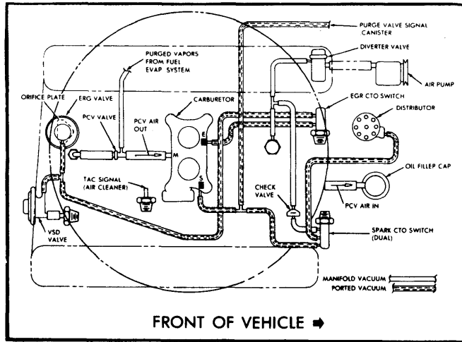
Fig. 21 360" V8 California Automatic Transmission "J" Models With Heavy Duty Cooling
