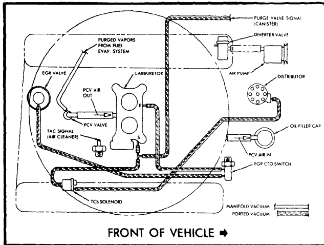
Fig. 13 304" V8 California Manual Transmission "CJ" Models
