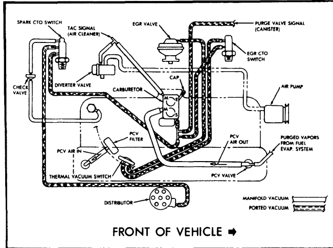
Fig. 3 258" 6 Cyl. Automatic Manual Transmission All Models
