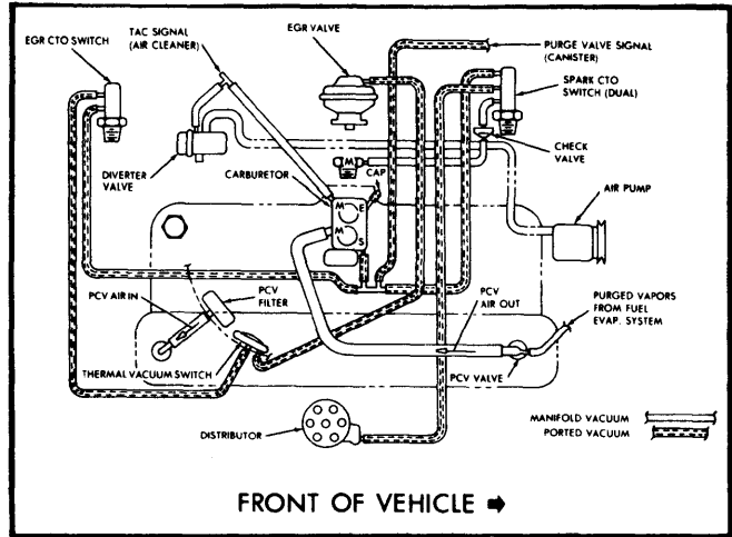
Fig. 8 258" 6 Cyl. California Automatic Transmission "CJ" Models With Heavy Duty Cooling
