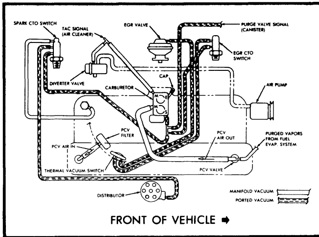
Fig. 1 258" 6 Cyl. Federal Manual Transmission All Models
