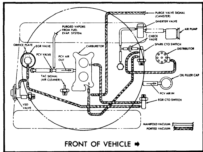
Fig. 20 360" V8 California Automatic Transmission "J" Models
