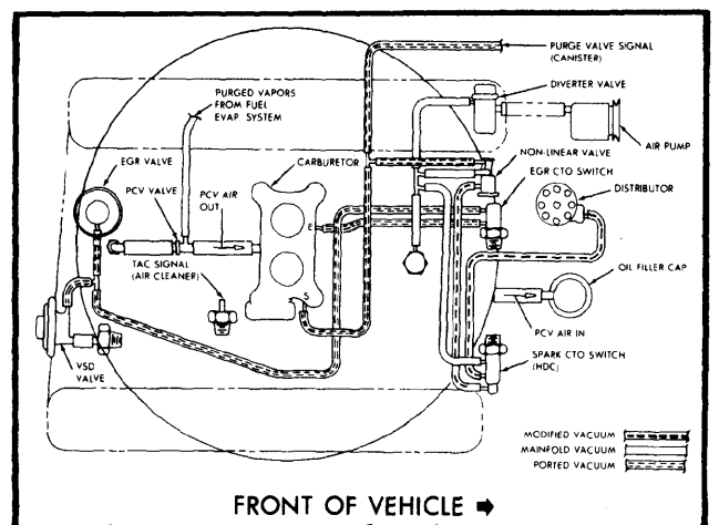
Fig. 18 360" V8 California Manual Transmission "J" Models With Heavy Duty Cooling
