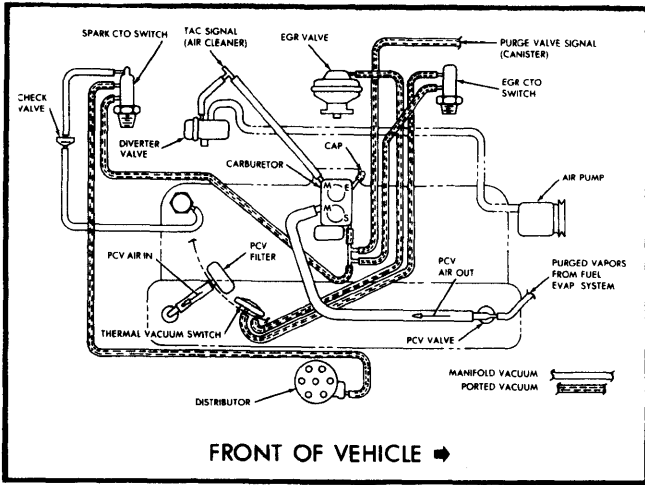
Fig. 7 258" 6 Cyl. California Automatic Transmission "CJ" Models
