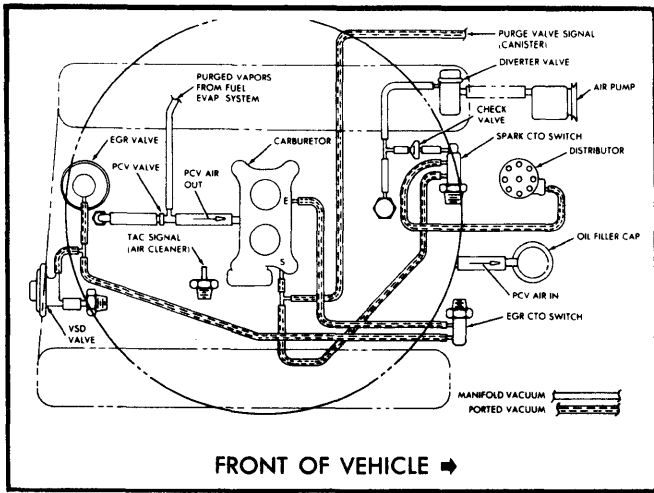
Fig. 19 360" V8 California Automatic Transmission Cherokee and Wagoneer Models
