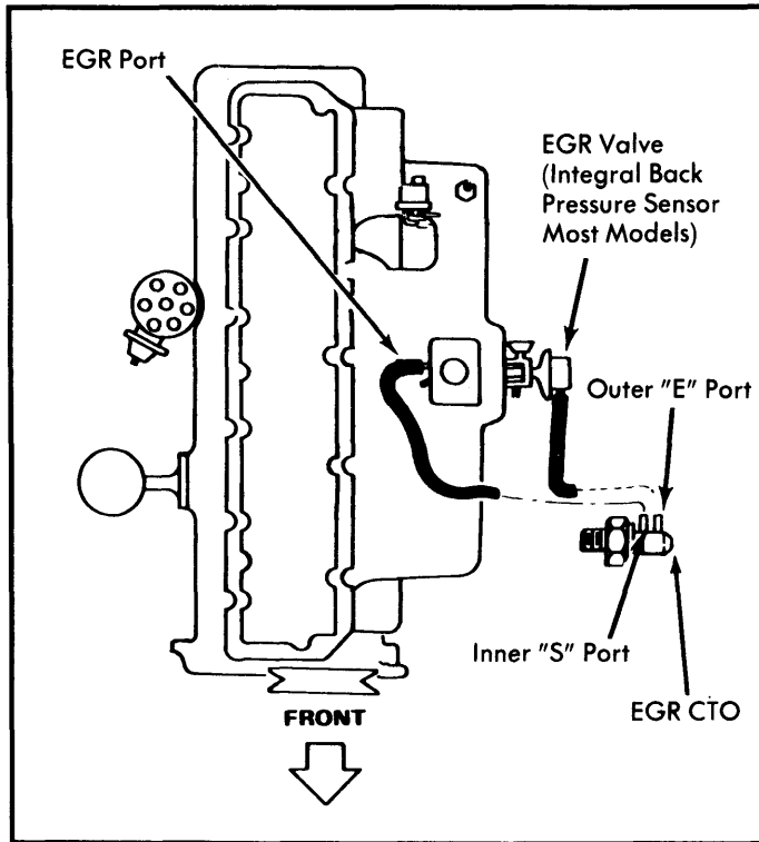
Fig. 5 Vacuum Schematic of EGR System (6 Cyl.)
