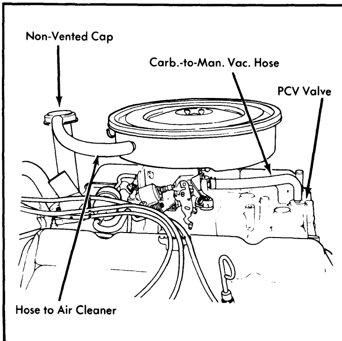
Fig. 2 Vacuum Schematic of PCV System (V8)
