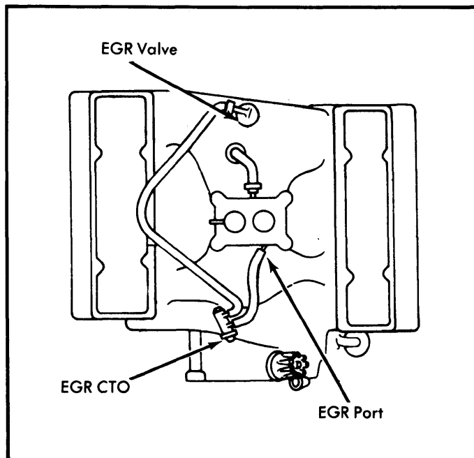
Fig. 6 Vacuum Schematic of EGR System (V8 Typical)
