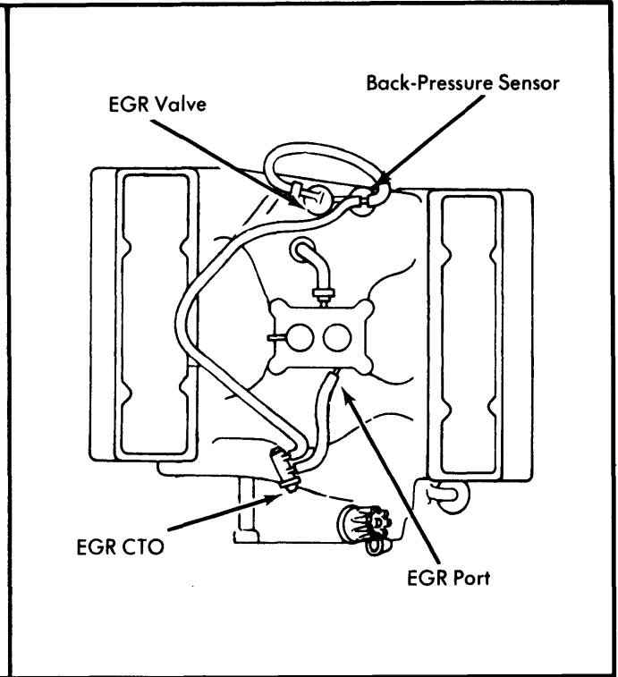
Fig. 7 Vacuum Schematic of EGR System (V8 Calif. "CJ" Models with Man. Trans.)
