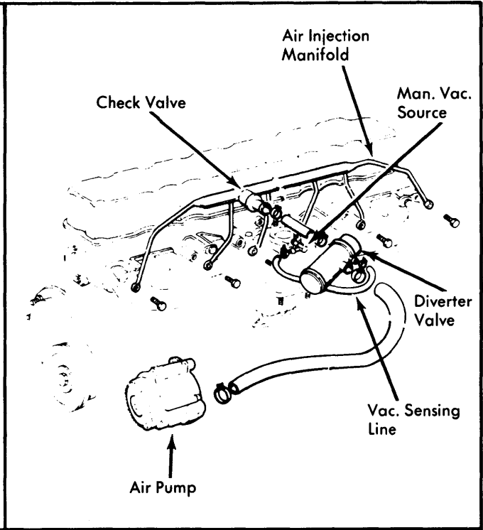
Fig. 3 Vacuum Schematic of A.I.R. System (6 Cyl)
