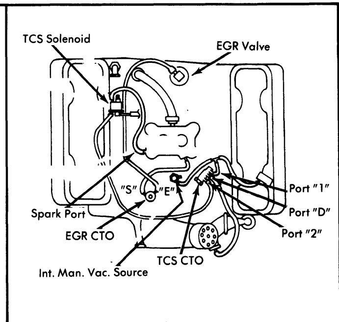
Fig. 8 Vacuum Schematic of TCS System
