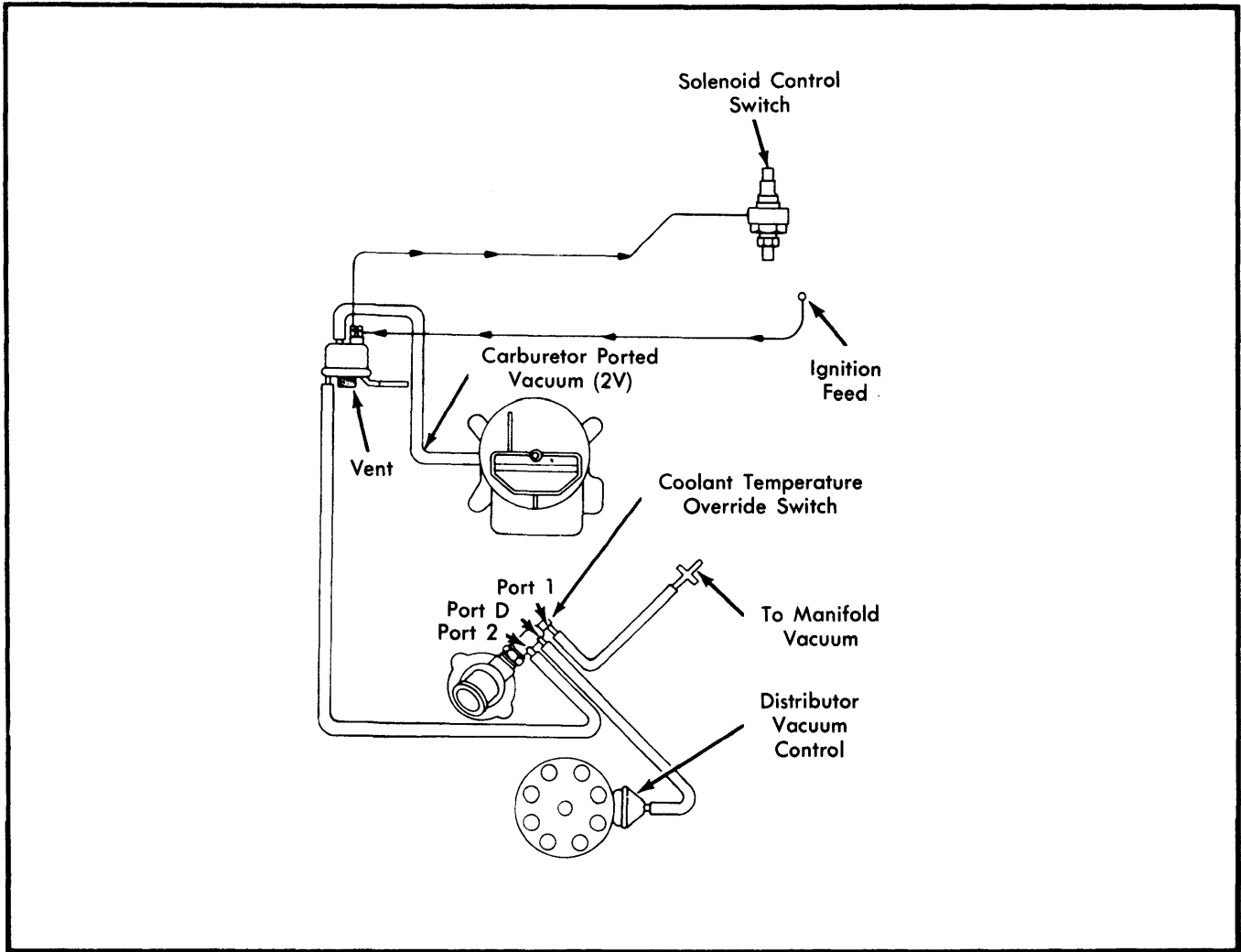
Fig. 9 Vacuum Schematic of VTM System (Typical)
