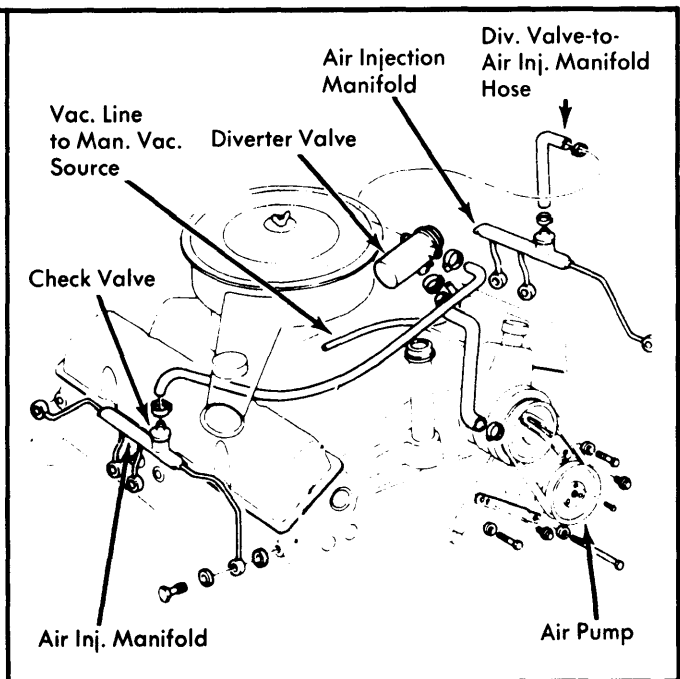
Fig. 4 Vacuum Schematic of A.I.R. System (V8)
