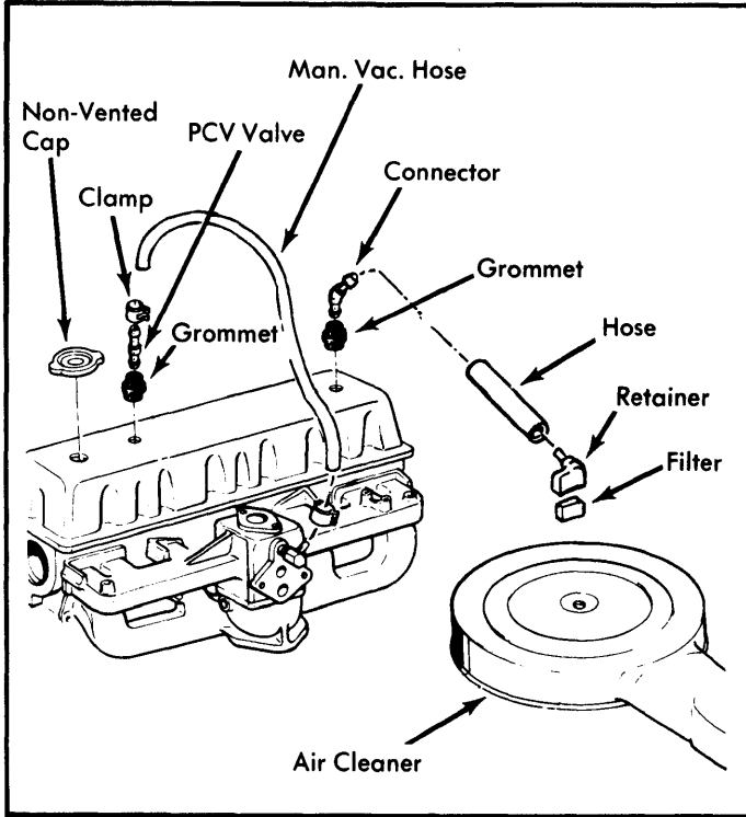
Fig. 1 Vacuum Schematic of PCV System (6Cyl)
