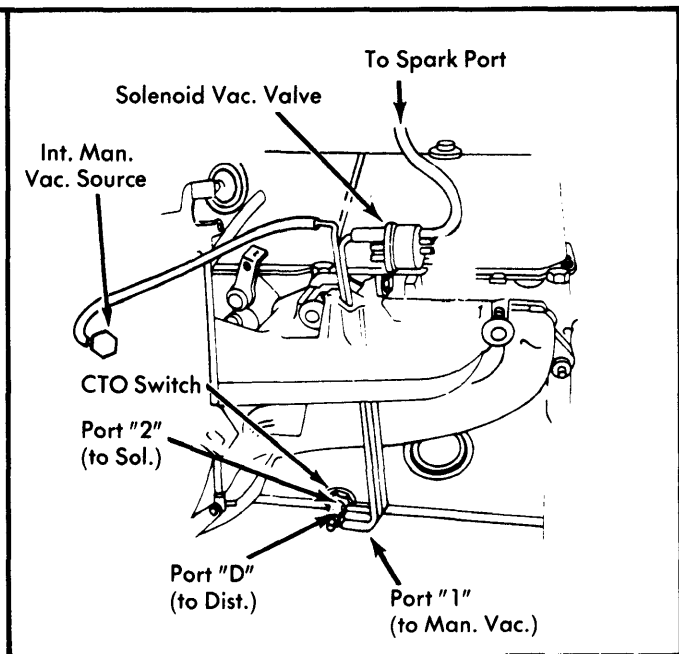
Fig. 8 Vacuum Schematic of TCS System (6 Cyl.)
