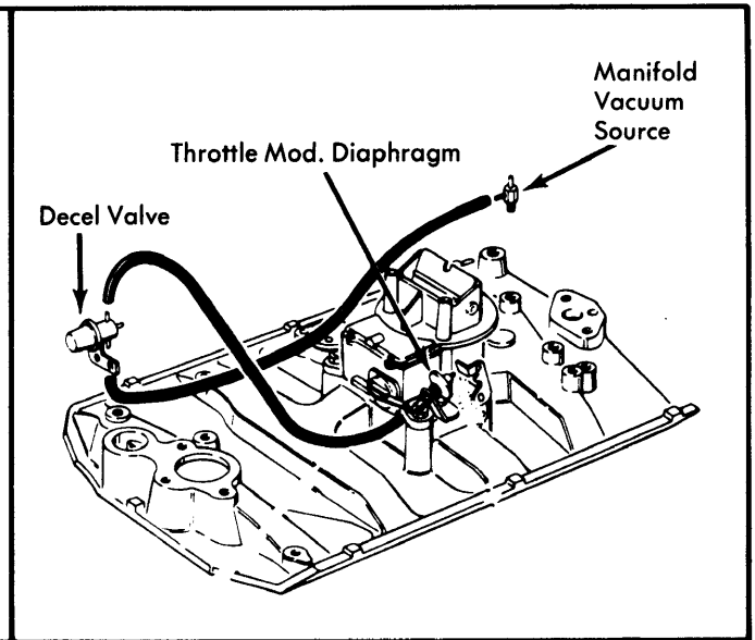
Fig. 10 Vacuum Schematic of VTM System (Typical)
