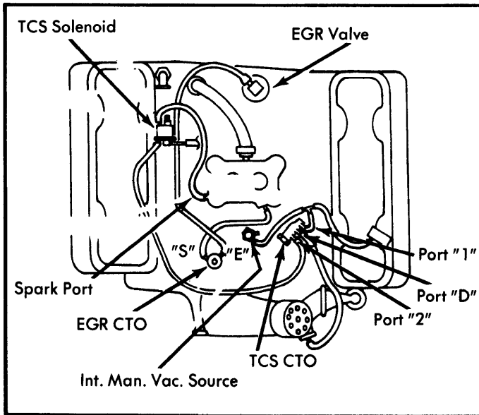
Fig. 9 Vacuum Schematic of TCS System (V8)
