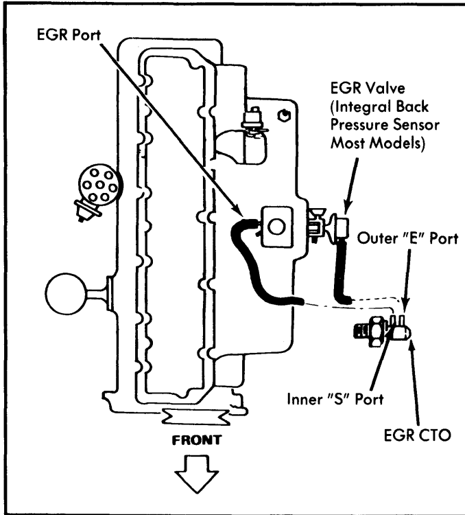
Fig. 5 Vacuum Schematic of EGR System (6 Cyl. Typical)
