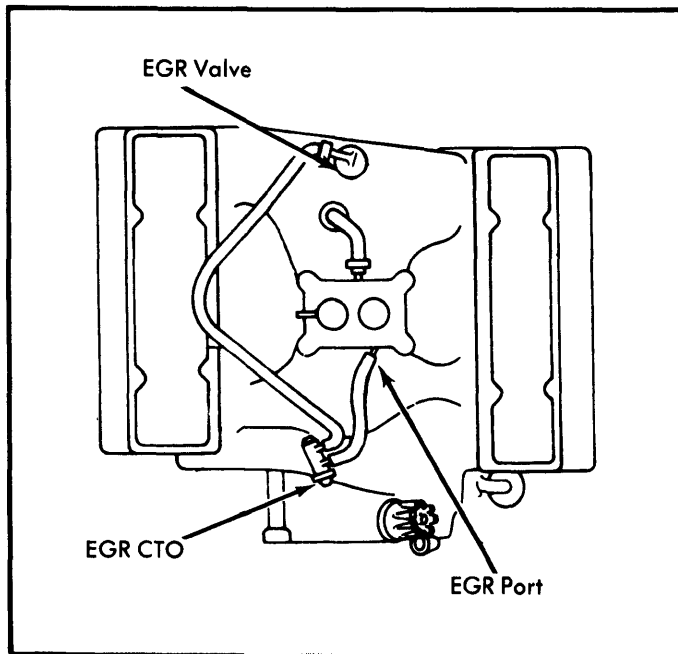
Fig. 6 Vacuum Schematic of EGR System (V8 Typical)
