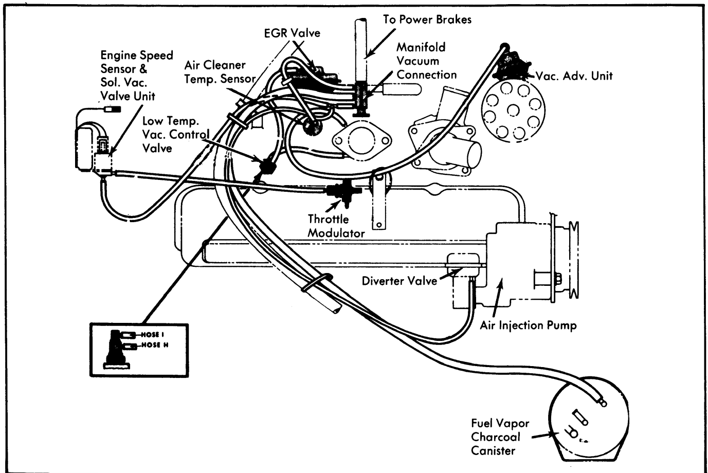
Fig. 2 IHC 196" 4 Cylinder Engine with Holley 1940C (Calif. Models Only)
