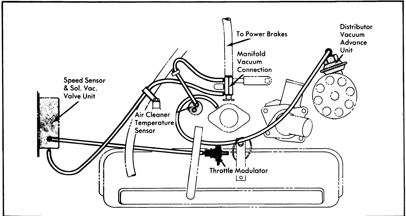
Fig. 1 IHC 196" 4 Cylinder Engine with Holley 1940C (Federal Models Only)
