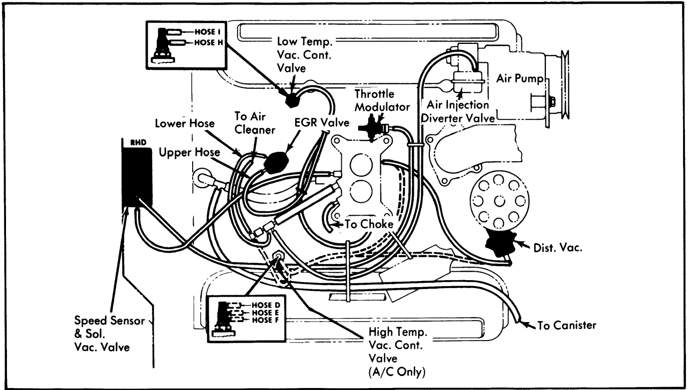
Fig. 5 IHC 345" V8 Engines with Holley 2210C (Calif. Models Only)
