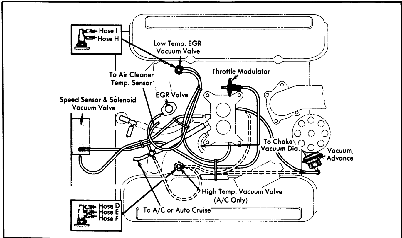
Fig. 3 IHC 304" & 345" V8 Engines with Holley 2210C (Federal Models Only)
