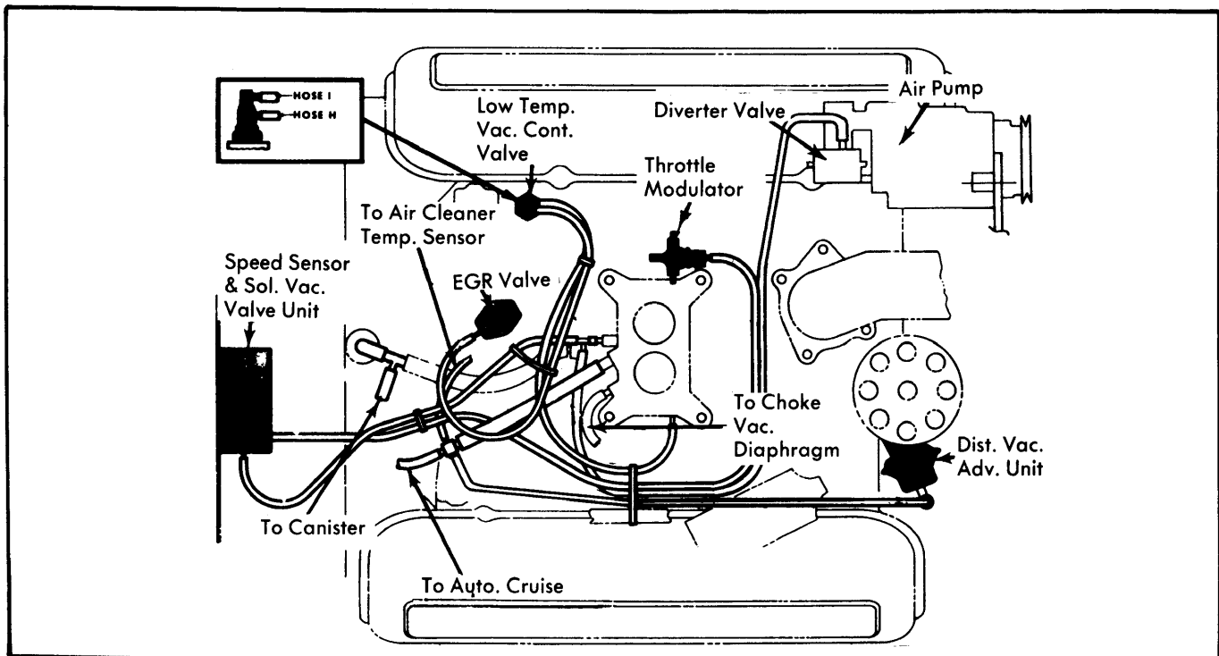
Fig. 4 IHC 304" V8 Engines with Holley 2245C (Calif. Models Only)
