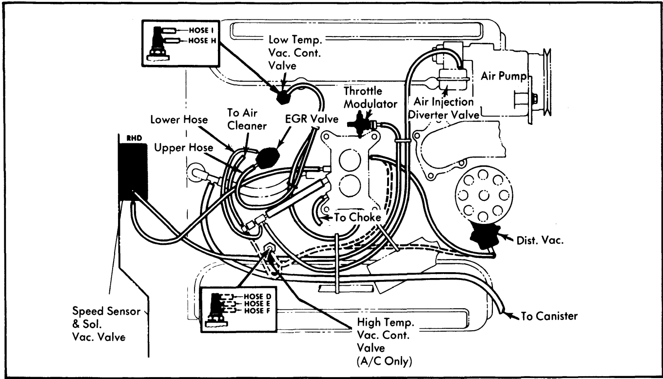
Fig. 5 IHC 345" V8 Engine with Holley 2210 (Calif. Models Only)
