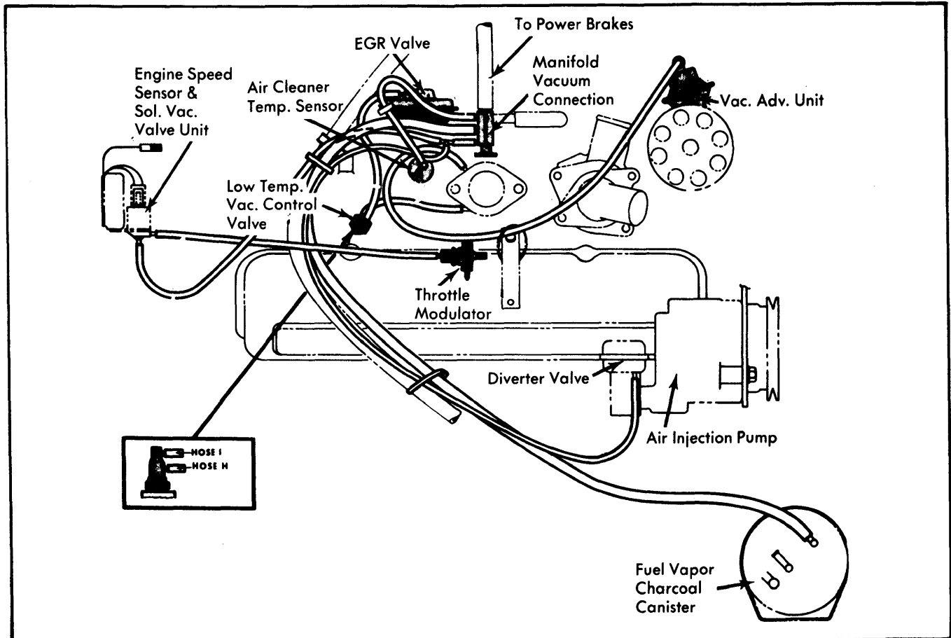
Fig. 2 IHC 196" 4 Cylinder Engine (Calif. Models Only)
