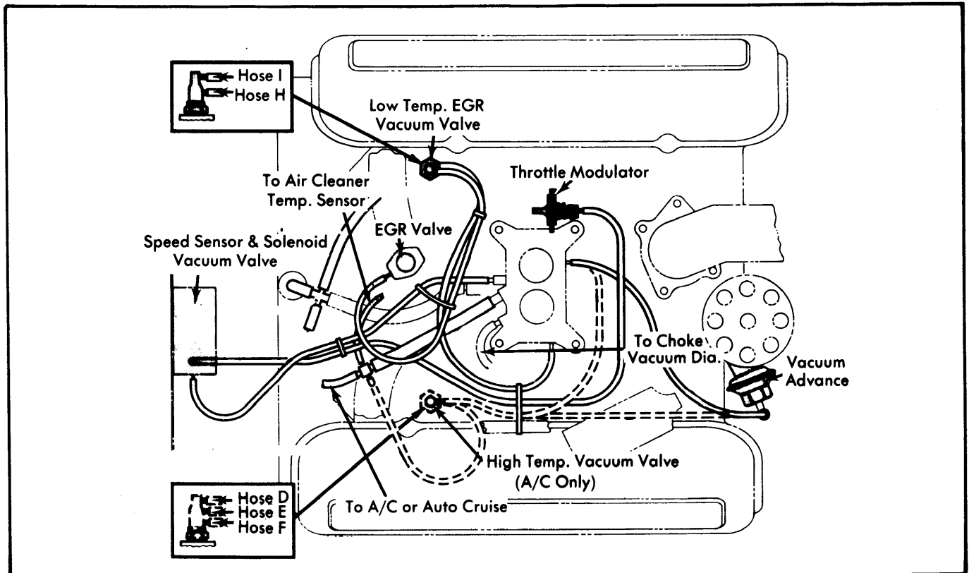
Fig. 3 IHC 304" & 345" V8 Engines with Holley 2210C (Federal Models Only)
