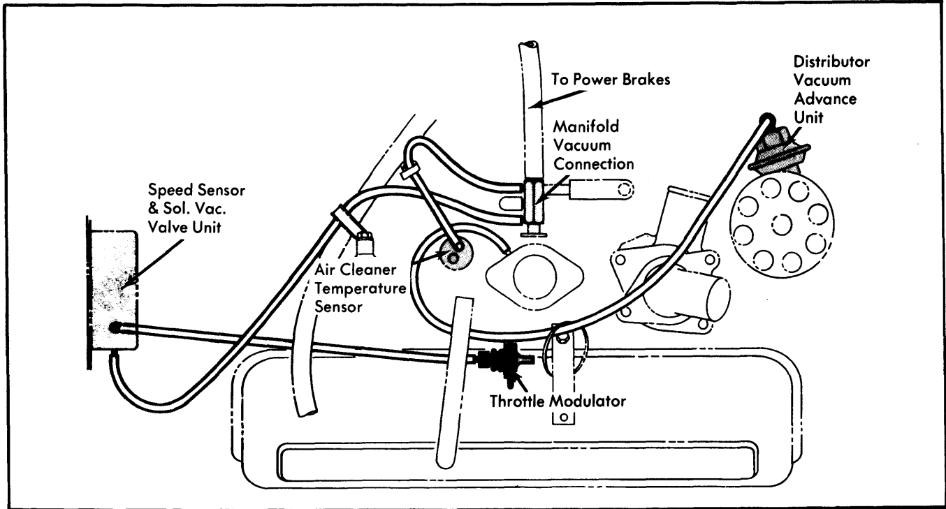
Fig. 1 IHC 196" 4 Cylinder Engine (Federal Models Only)
