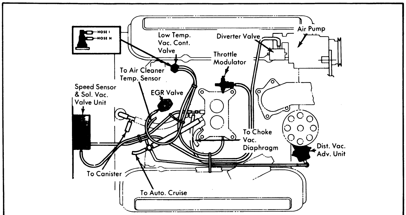
Fig. 4 IHC 304" V8 Engines with Holley 2245C (California Models Only)
