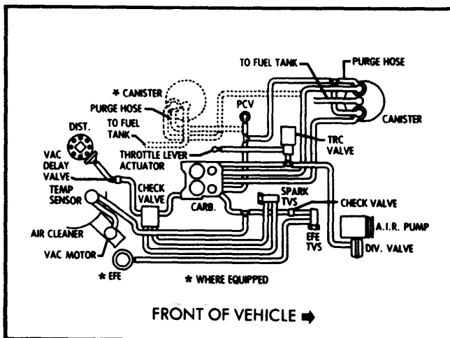
Fig. 15 350" V8 California Heavy Duty Emissions All Models
