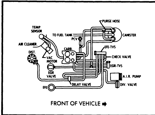
Fig. 11 350" V8 California Light Duty Emissions Single Fuel Evaporation Canister
