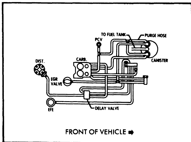
Fig. 9 350" V8 Federal Light Duty Emissions Single Fuel Evaporation Canister
