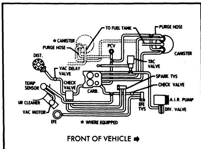
Fig. 21 400" V8 California Heavy Duty Emissions All Models
