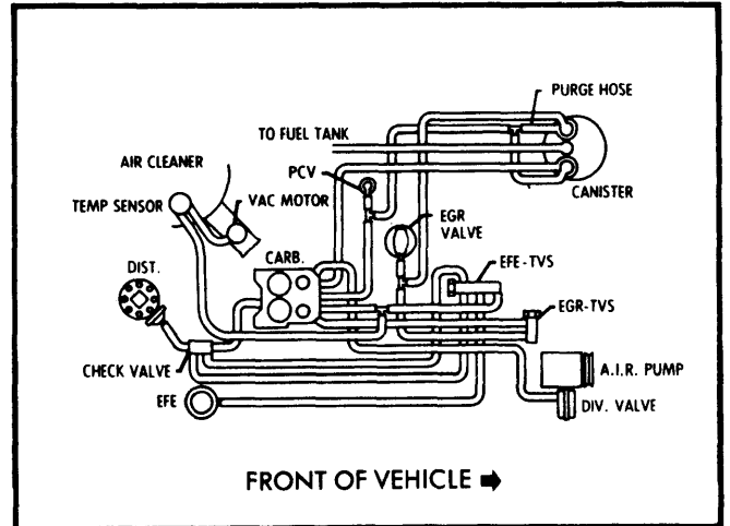
Fig. 24 454" V8 California Light Duty Emissions Single Fuel Evaporation Canister
