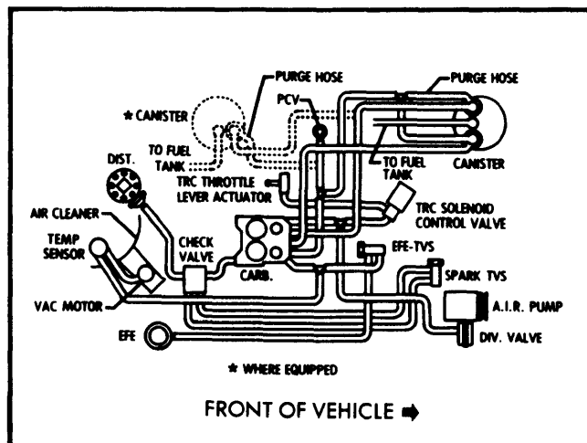
Fig. 27 454" V8 California Heavy Duty Emissions All Models
