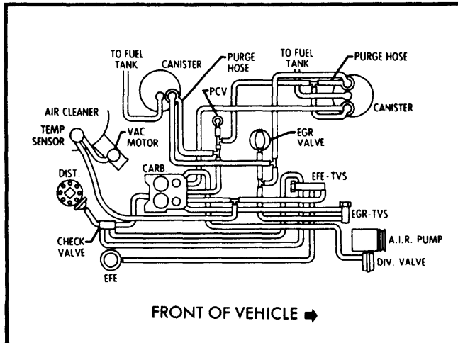
Fig. 25 454" V8 California Light Duty Emissions Dual Fuel Evaporation Canister
