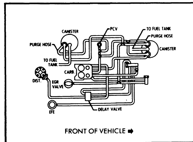
Fig. 10 350" V8 Federal Light Duty Emissions Dual Fuel Evaporation Canister
