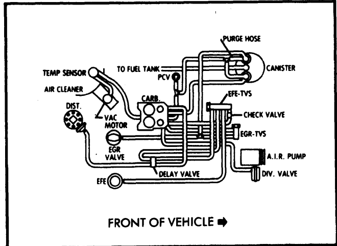
Fig. 18 400" V8 California Light Duty Emissions Single Fuel Evaporation Canister
