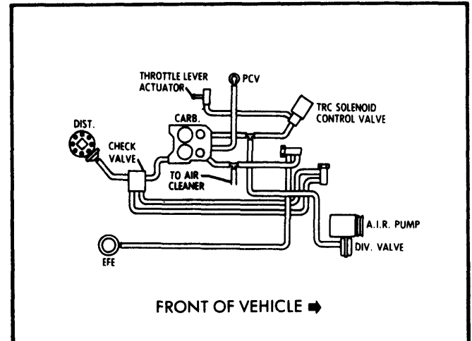
Fig. 26 454" V8 Federal Heavy Duty Emissions All Models
