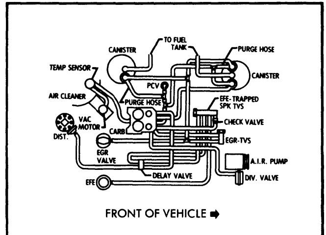
Fig. 12 350" V8 California Light Duty Emissions Dual Fuel Evaporation Canister
