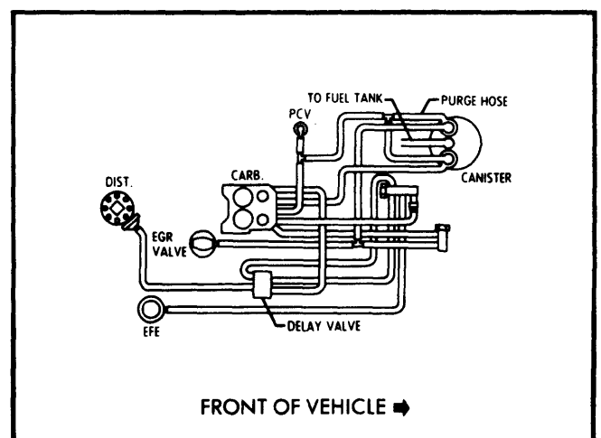
Fig. 16 400" V8 Federal Light Duty Emissions Single Fuel Evaporation Canister
