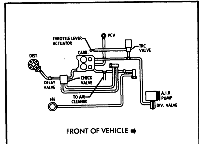
Fig. 20 400" V8 Federal Heavy Duty Emissions All Models
