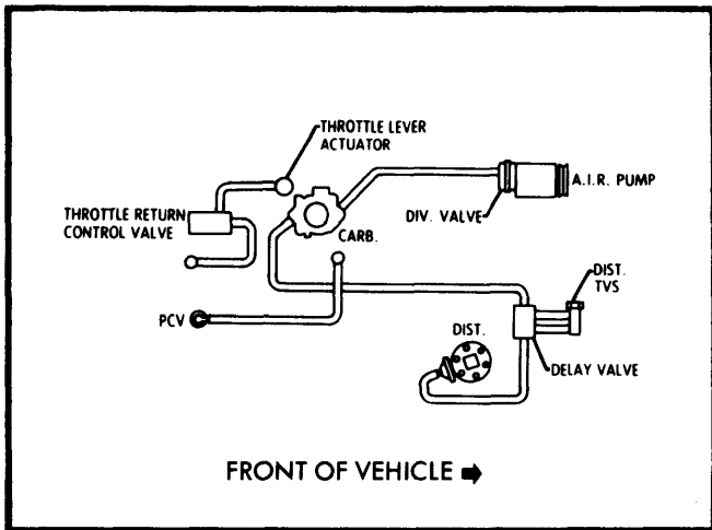
Fig. 5 292" 6 Cyl. Federal Heavy Duty Emissions All Models
