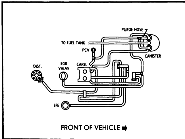
Fig. 7 305" V8 Federal Light Duty Emissions Single Fuel Evaporation Canister
