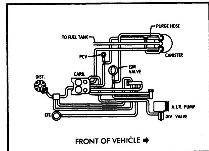
Fig. 22 454" V8 Federal Light Duty Emissions Single Fuel Evaporation Canister
