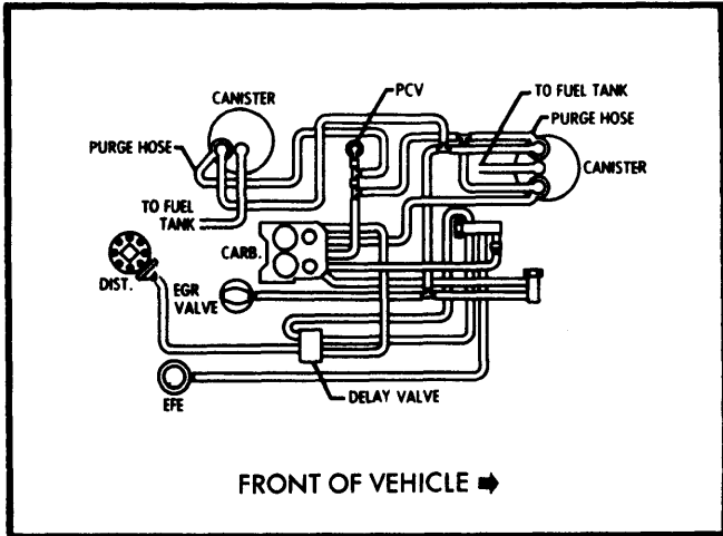
Fig. 17 400" V8 Federal Light Duty Emissions Dual Fuel Evaporation Canister
