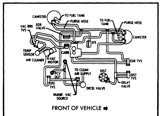
Fig. 4 250" 6 Cyl. California Light Duty Emissions Dual Fuel Evaporation Canister
