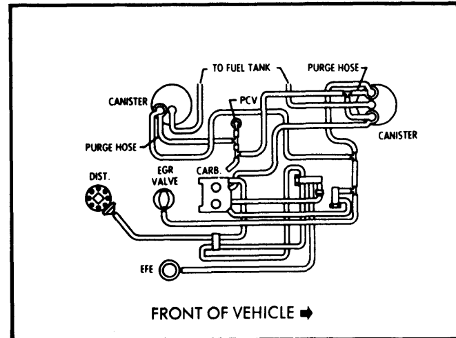
Fig. 8 305" V8 Federal Light Duty Emissions Dual Fuel Evaporation Canister
