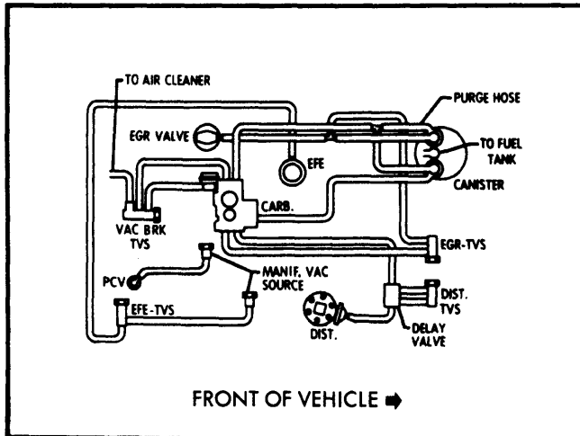
Fig. 1 250" 6 Cyl. Federal Light Duty Emissions Single Fuel Evaporation Canister
