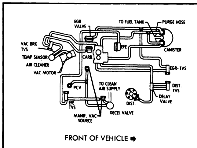
Fig. 3 250" 6 Cyl. California Light Duty Emissions Single Fuel Evaporation Canister
