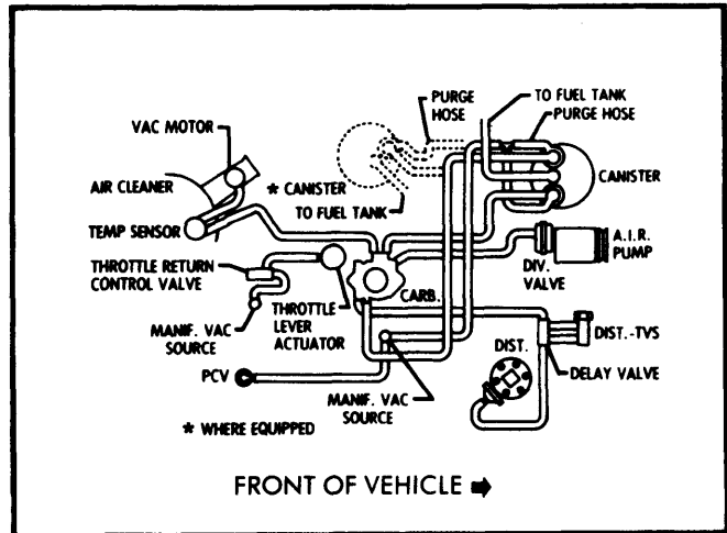
Fig. 6 292" 6 Cyl. California Heavy Duty Emissions All Models
