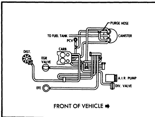
Fig. 13 350" V8 Altitude Light Duty Emissions Single Fuel Evaporation Canister
