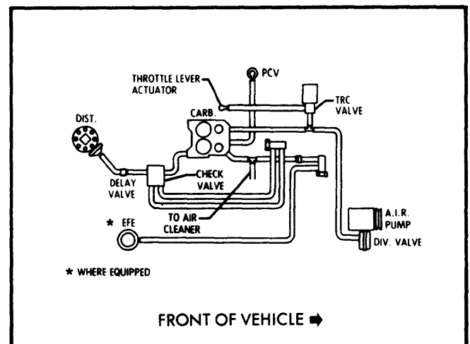
Fig. 14 350" V8 Federal Heavy Duty Emissions All Models
