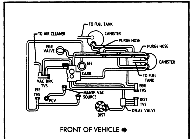
Fig. 2 250" 6 Cyl. Federal Light Duty Emissions Dual Fuel Evaporation Canister
