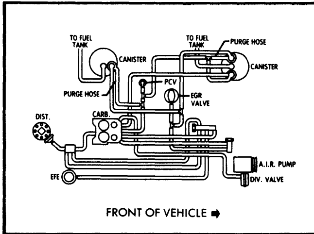
Fig. 23 454" V8 Federal Light Duty Emissions Dual Fuel Evaporation Canister
