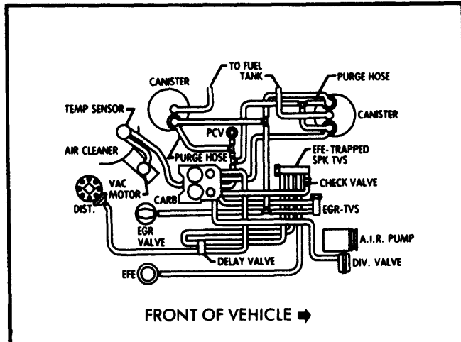
Fig. 19 400" V8 California Light Duty Emissions Dual Fuel Evaporation Canister
