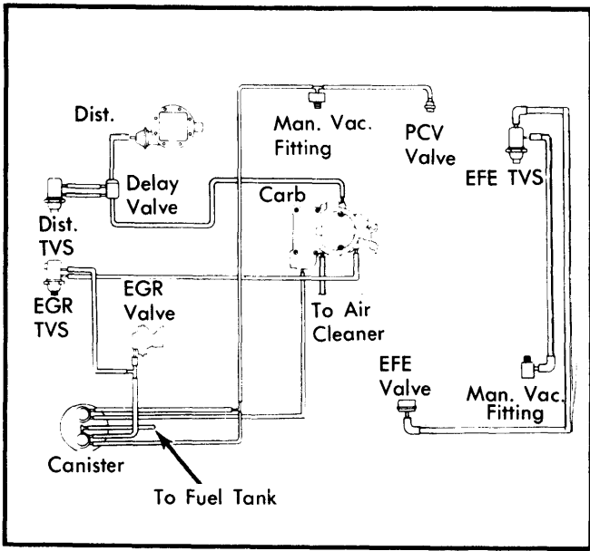
Fig. 1 Vacuum Hose Schematic for 250" Federal Light Duty Emission System
