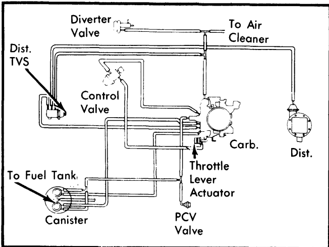
Fig. 12 Vacuum Hose Schematic for 350" & 400" Calif. Heavy Duty Emission System (W/A/C)
