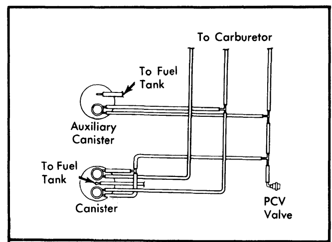
Fig. 16 Vacuum Hose Schematic for All Trucks with Two Canister System
