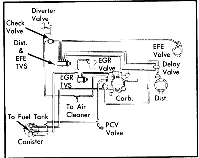
Fig. 8 Vacuum Hose Schematic for 350" Calif. Light Duty Emission System
