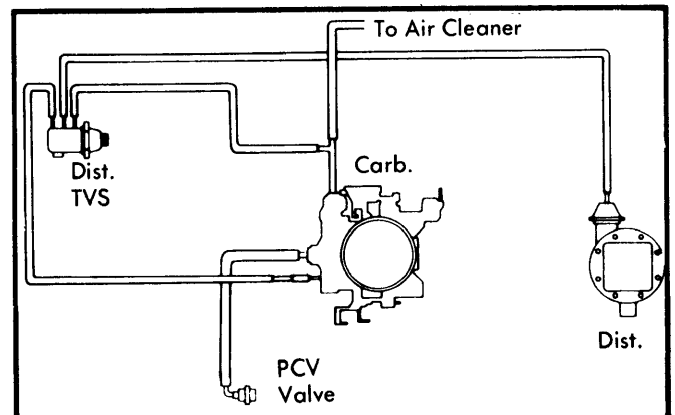
Fig. 10 Vacuum Hose Schematic for 350" & 400" Heavy Duty Emission System (W/A/C)
