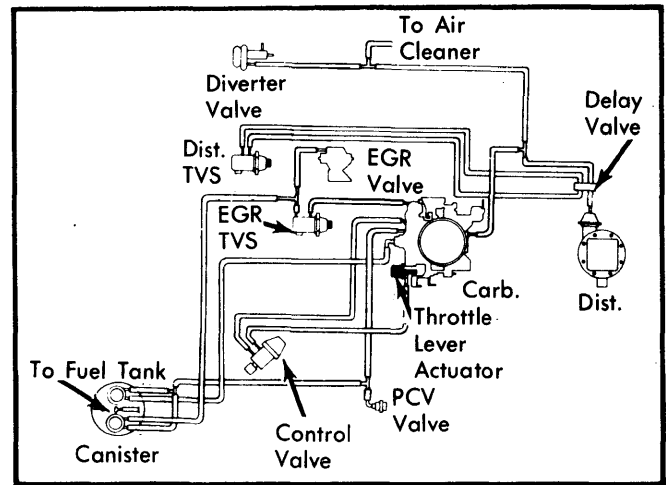
Fig. 15 Vacuum Hose Schematic for 454" Calif. Heavy Duty Emission System
