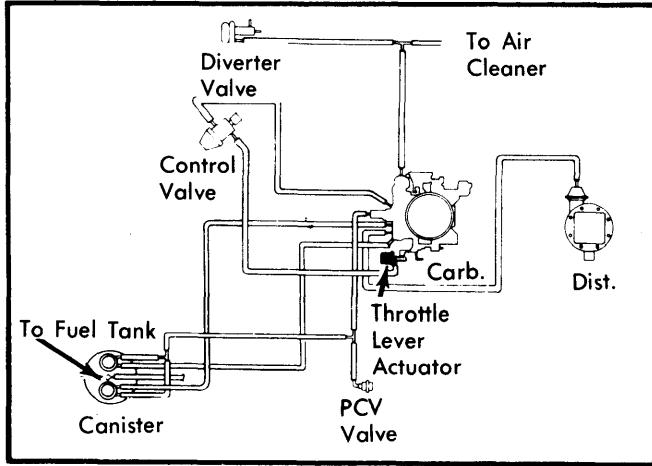
Fig. 11 Vacuum Hose Schematic for 350" & 400" Calif. Heavy Duty Emission System (W/O A/C)
