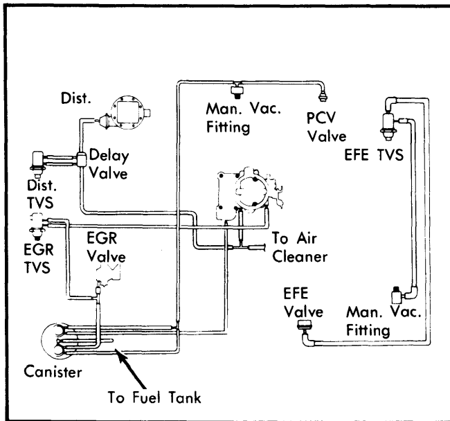
Fig. 2 Vacuum Hose Schematic for 250" Calif. Light Duty Emission System
