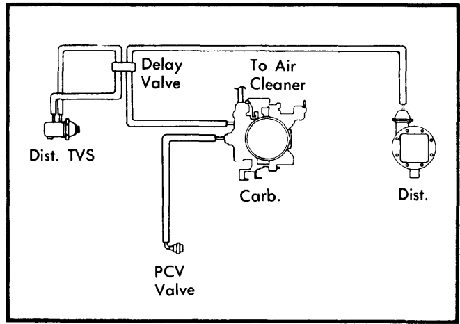
Fig. 14 Vacuum Hose Schematic for 454" Federal Heavy Duty Emission System
