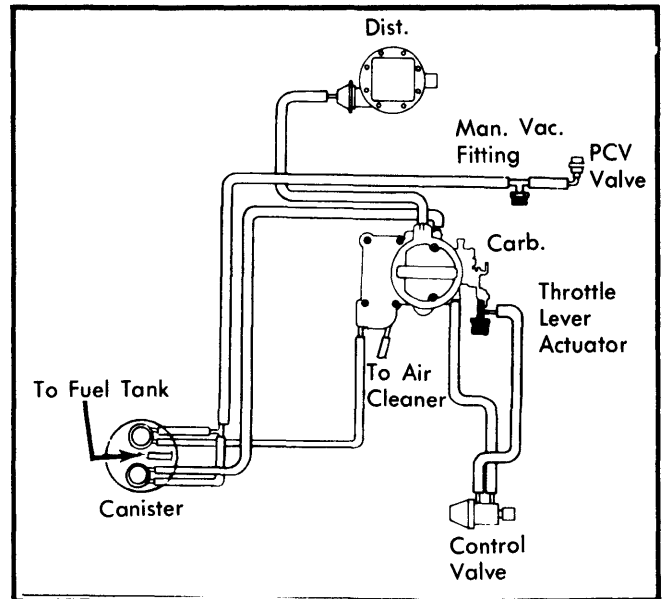
Fig. 4 Vacuum Hose Schematic for 292" Calif. Heavy Duty Emission System
