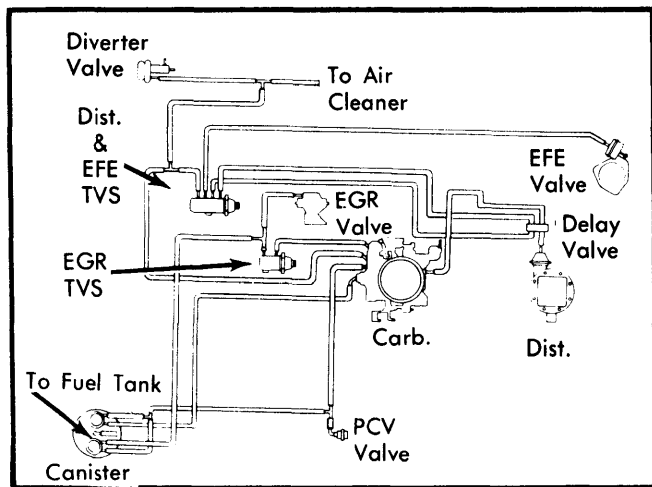
Fig. 13 Vacuum Hose Schematic for 454" Light Duty Emission System
