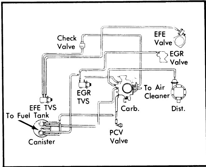
Fig. 5 Vacuum Hose Schematic for 305" Low Altitude Light Duty Emission System
