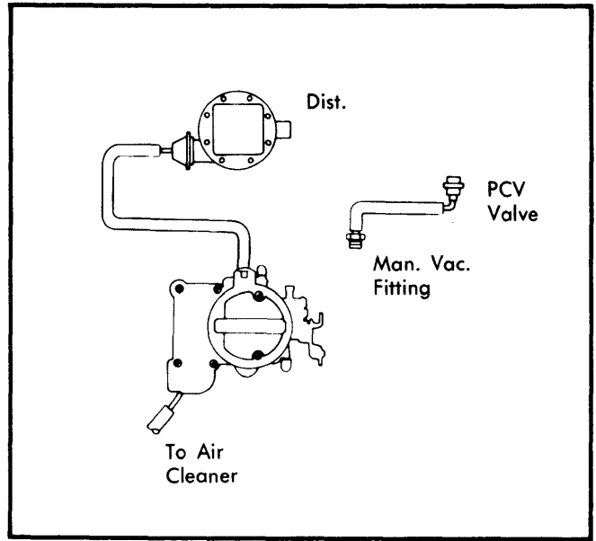
Fig. 3 Vacuum Hose Schematic for 250" & 292" Federal Heavy Duty Emission System
