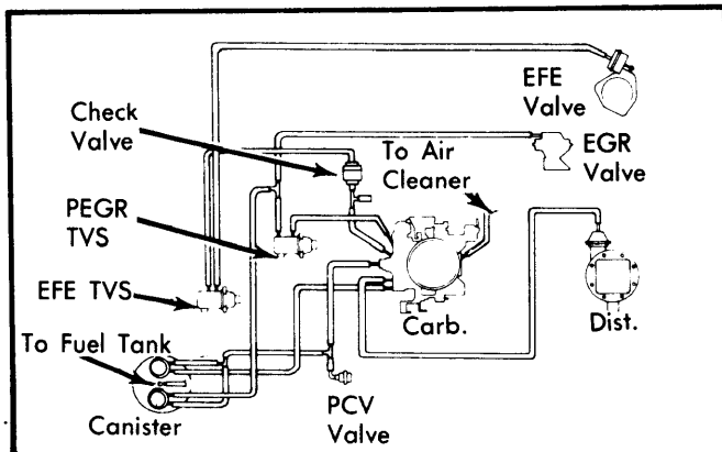
Fig. 7 Vacuum Hose Schematic for 350" Low Altitude Light Duty Emission System
