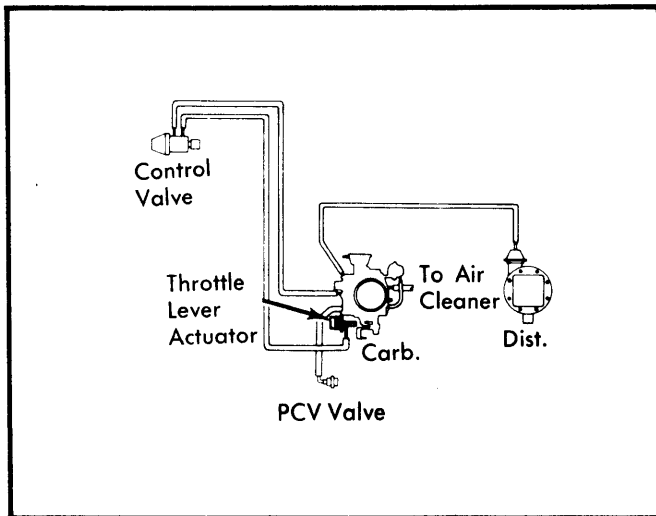
Fig. 5 Vacuum Hose Schematic for 305" Low Altitude Light Duty Emission System
