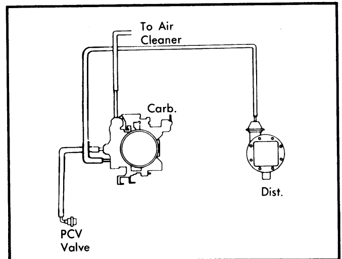
Fig. 8 Vacuum Hose Schematic for 350" Calif. Light Duty Emission System
