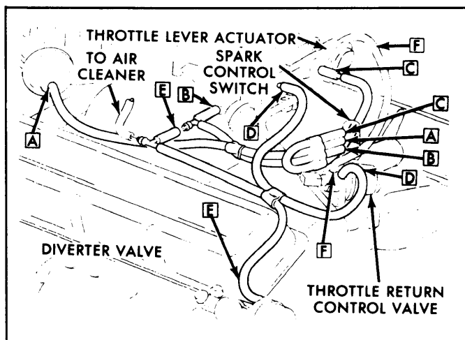
Fig. 9: California Light & Heavy Duty Pickup 400" V8 (4WD)
