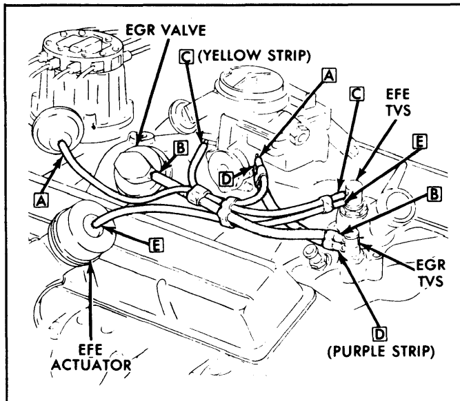
Fig. 2: Federal Light Duty Van 350" V8 2-Bbl.
