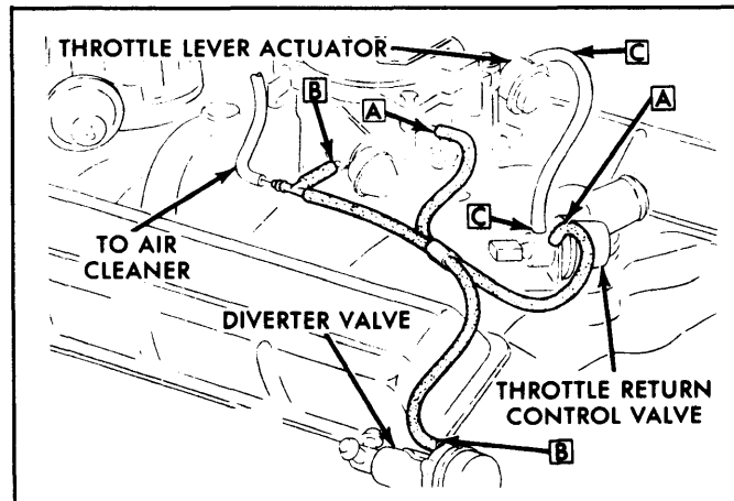
Fig. 3: California Pickup 350" & 400" V8 (2WD) & Heavy Duty California Step Van 350" V8
