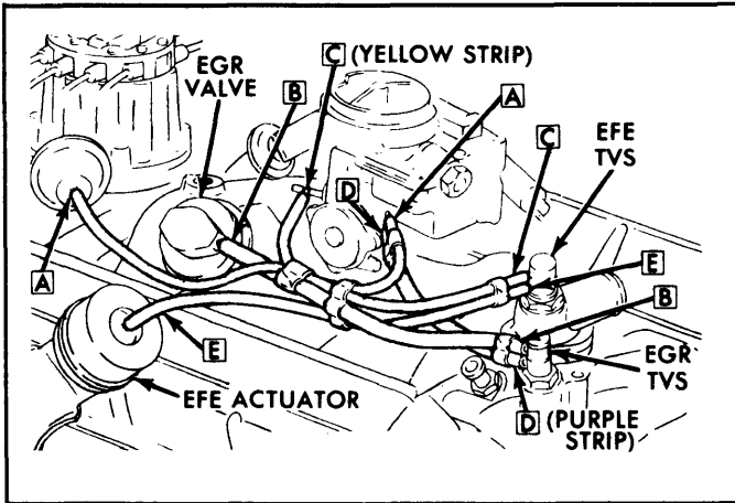
Fig. 1: Federal Light Duty 350" V8 2-Bbl. (2WD)
