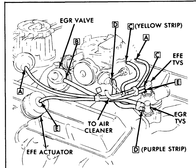
Fig. 6: Federal Light Duty Pickup 350" V8 4-Bbl. (4WD)
