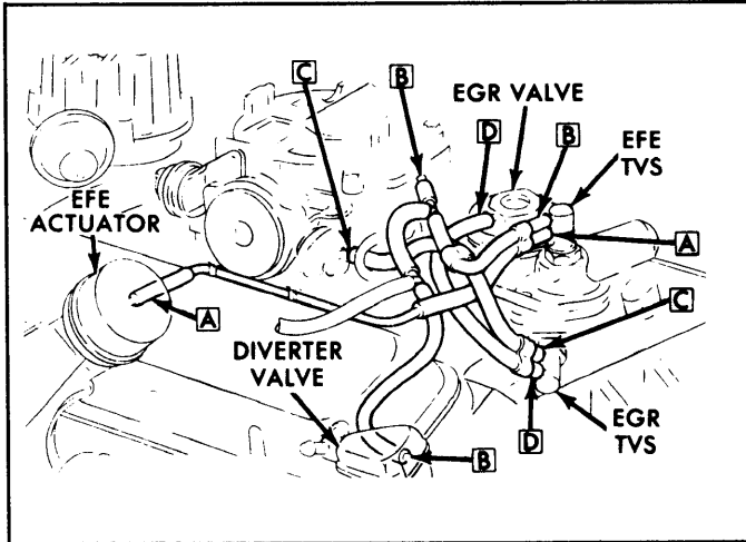
Fig. 13: Federal Light Duty Pickup 454" V8
