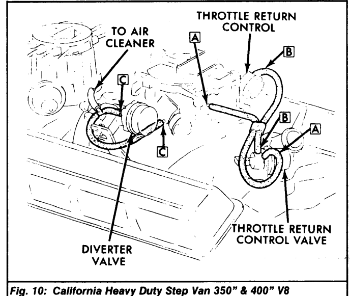
Fig. 10: California Heavy Duty Step Van 350" & 400" V8
