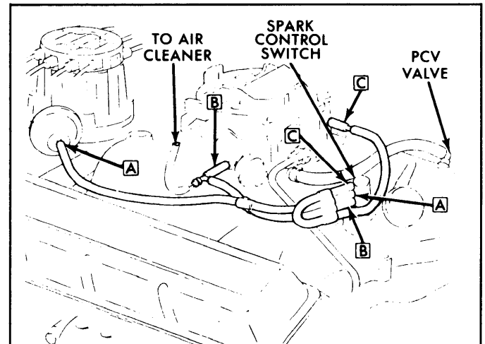
Fig. 11: California Heavy Duty Step Van 400" V8
