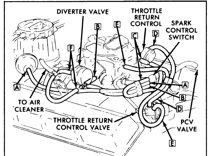
Fig. 11: California Heavy Duty Step Van 400" V8
