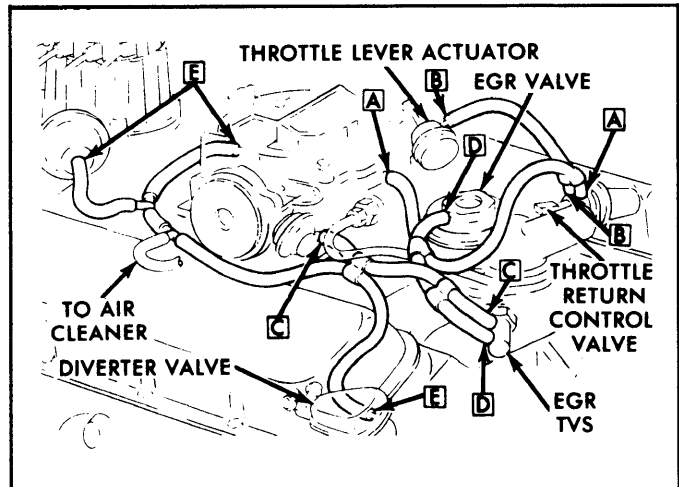
Fig. 14: California Light & Heavy Duty Pickup 454" V8 (2WD) & California Heavy Duty Step Van 454" V8
