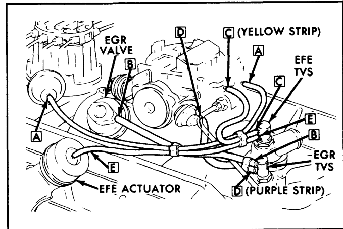
Fig. 5: Federal Light Duty Pickup 350" V8 4-Bbl. (2WD Without Air Injection Reactor)
