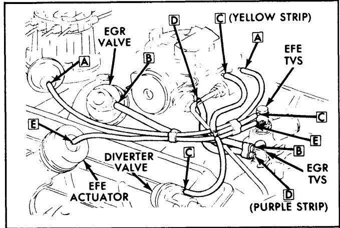
Fig. 4: Federal Light Duty Pickup 350" V8 4-Bbl. (2WD With Air Injection Reactor)
