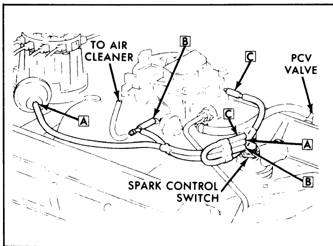
Fig. 8: Federal Light & Heavy Duty Pickup 400" V8 (4WD Without Air Injection Reactor)
