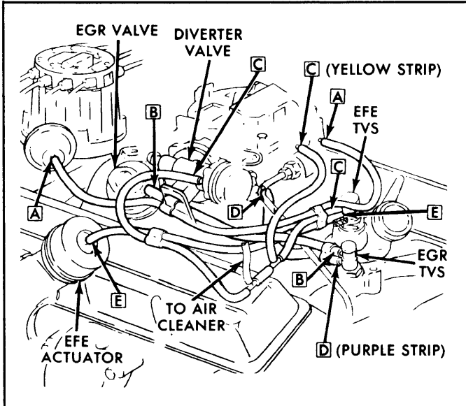
Fig. 7: California Light Duty Pickup 350" V8 4-Bbl. (4WD)
