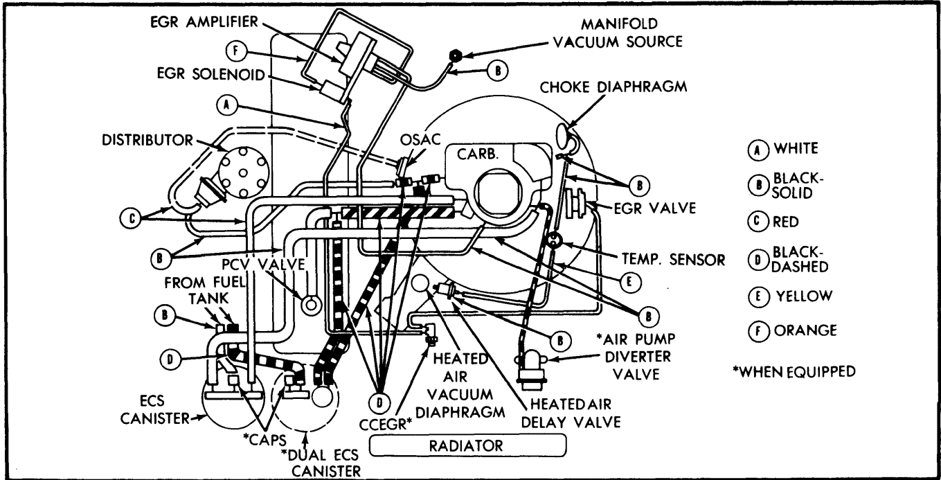
Fig. 1 225" 6 Cyl. Federal All Models
