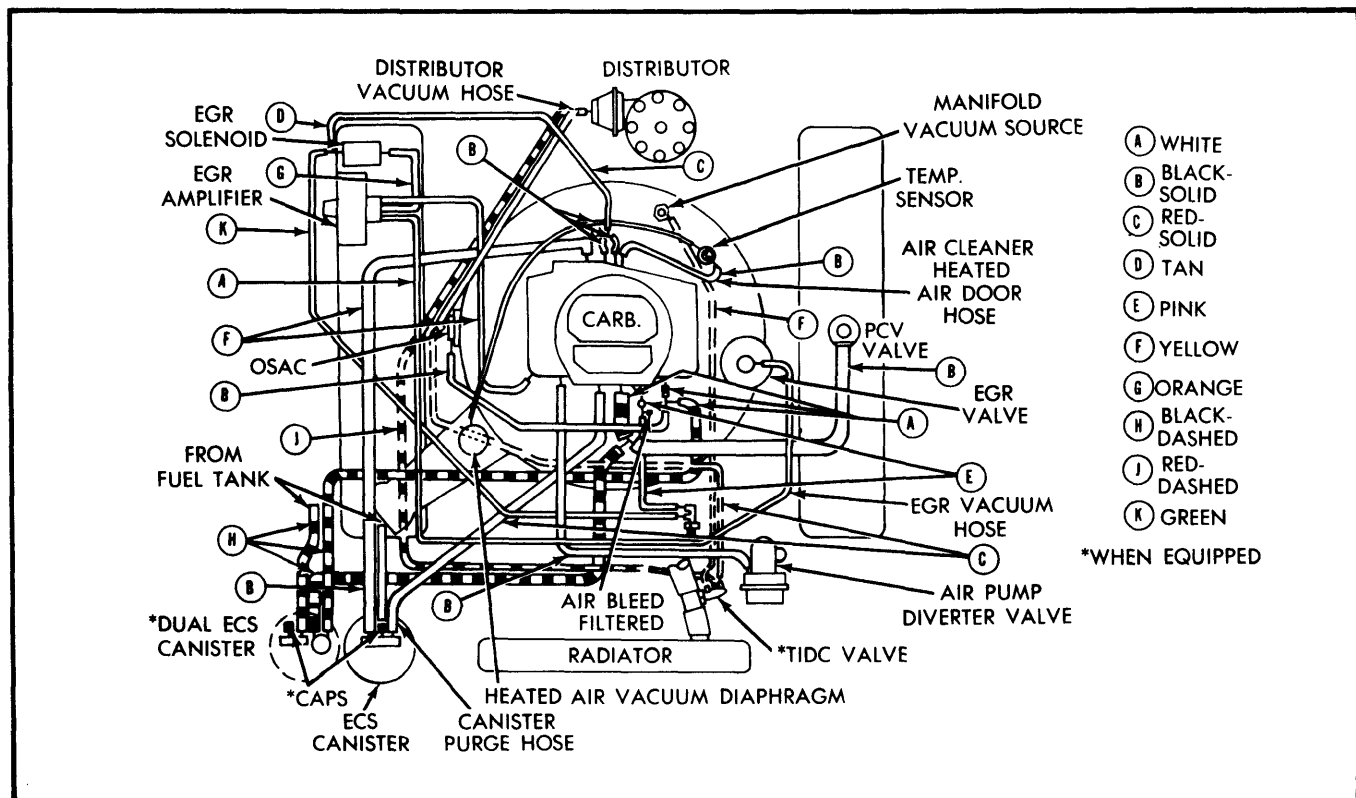
Fig. 8 360" V8 4-Barrel California Light Duty Emissions All Models
