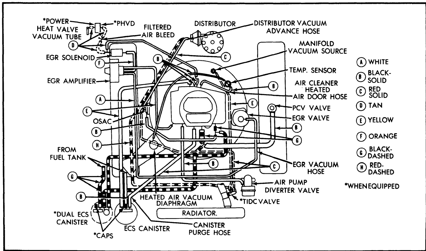
Fig. 4 318" V8 California All Models
