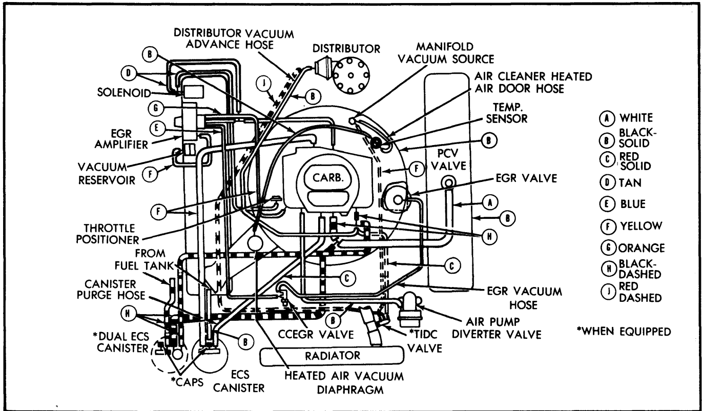
Fig. 9 360" V8 4-Barrel Heavy Duty Emissions All Models
