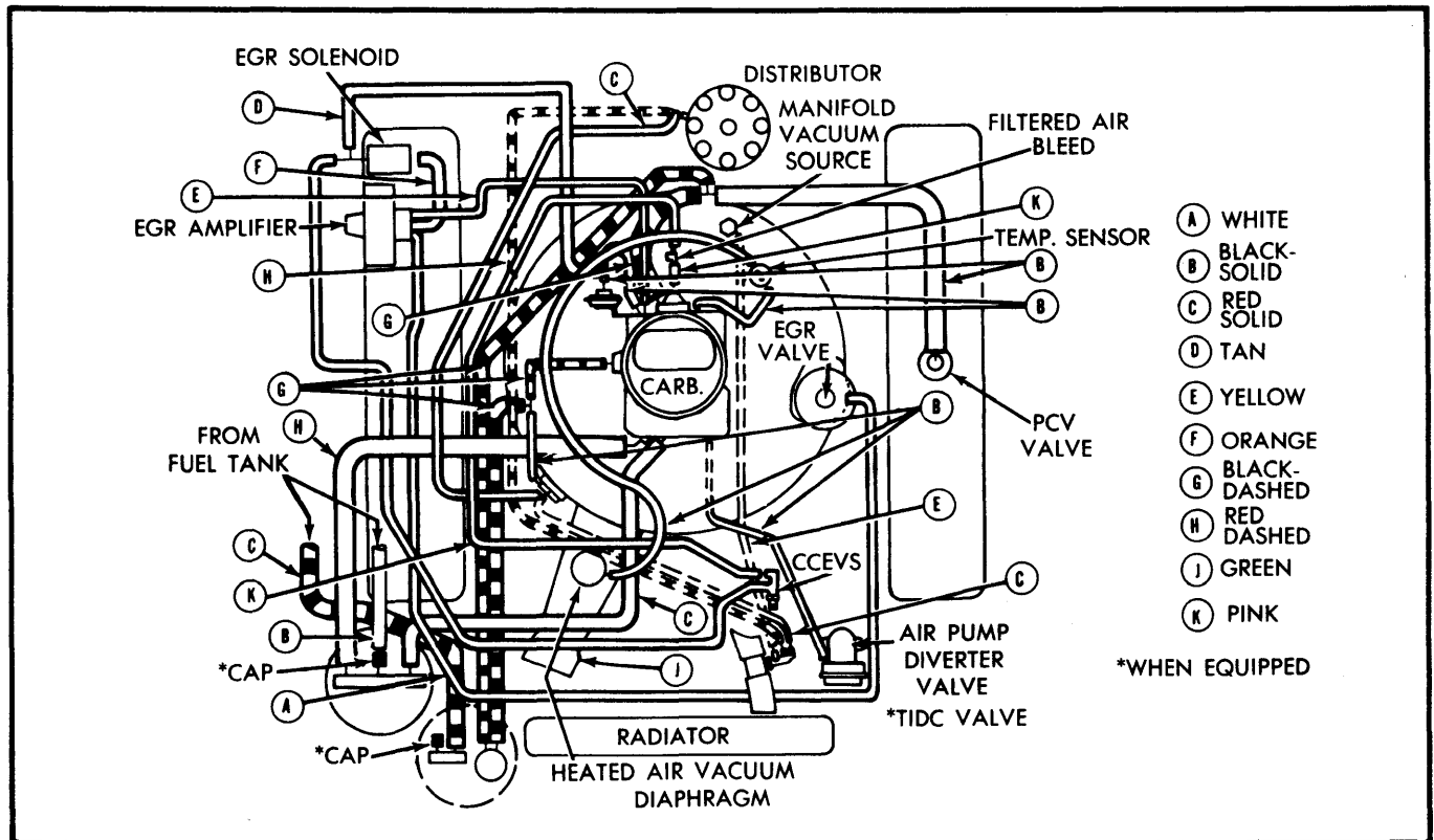
Fig. 5 360" V8 2-Barrel Federal All Models
