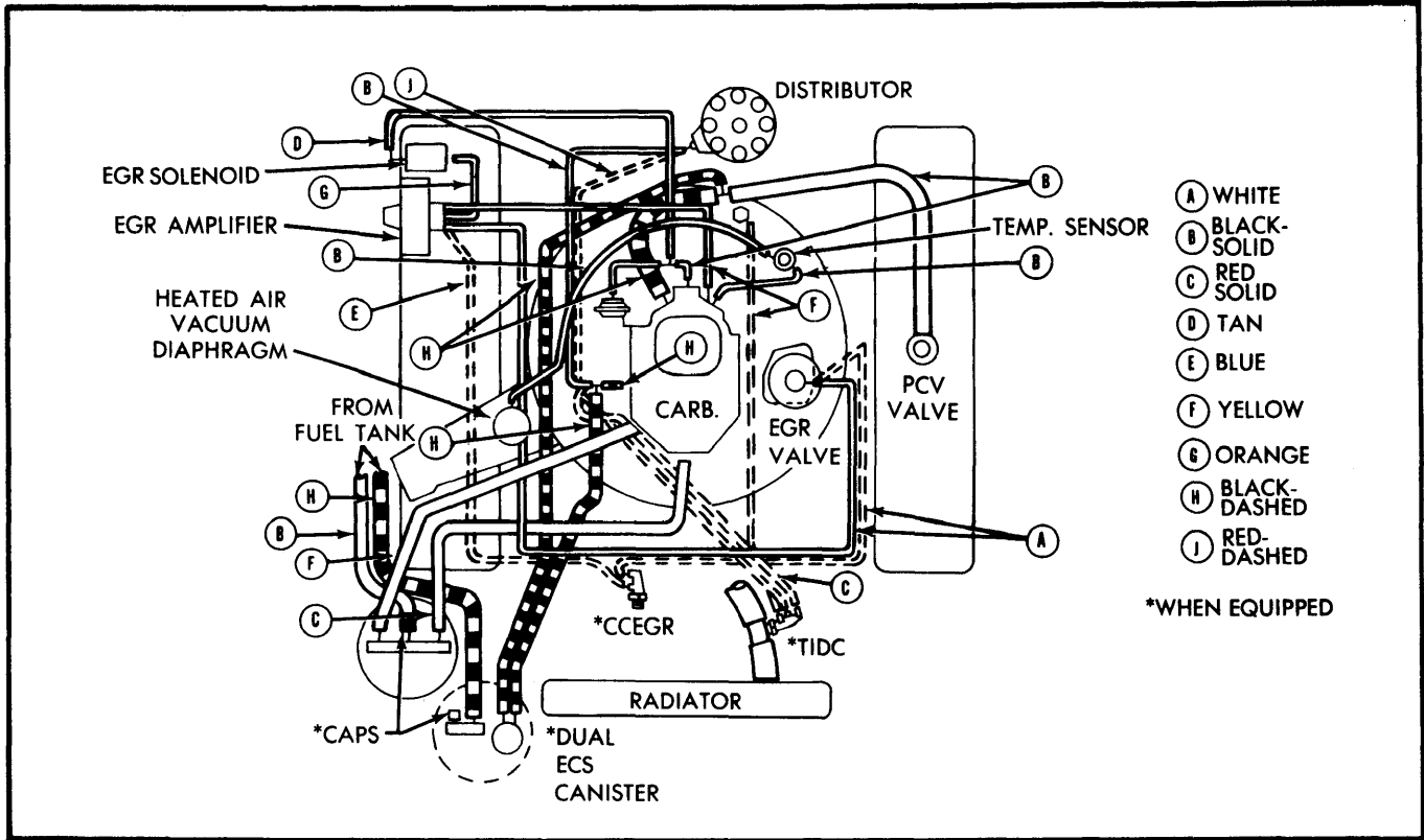
Fig. 3 318" V8 Federal All Model
