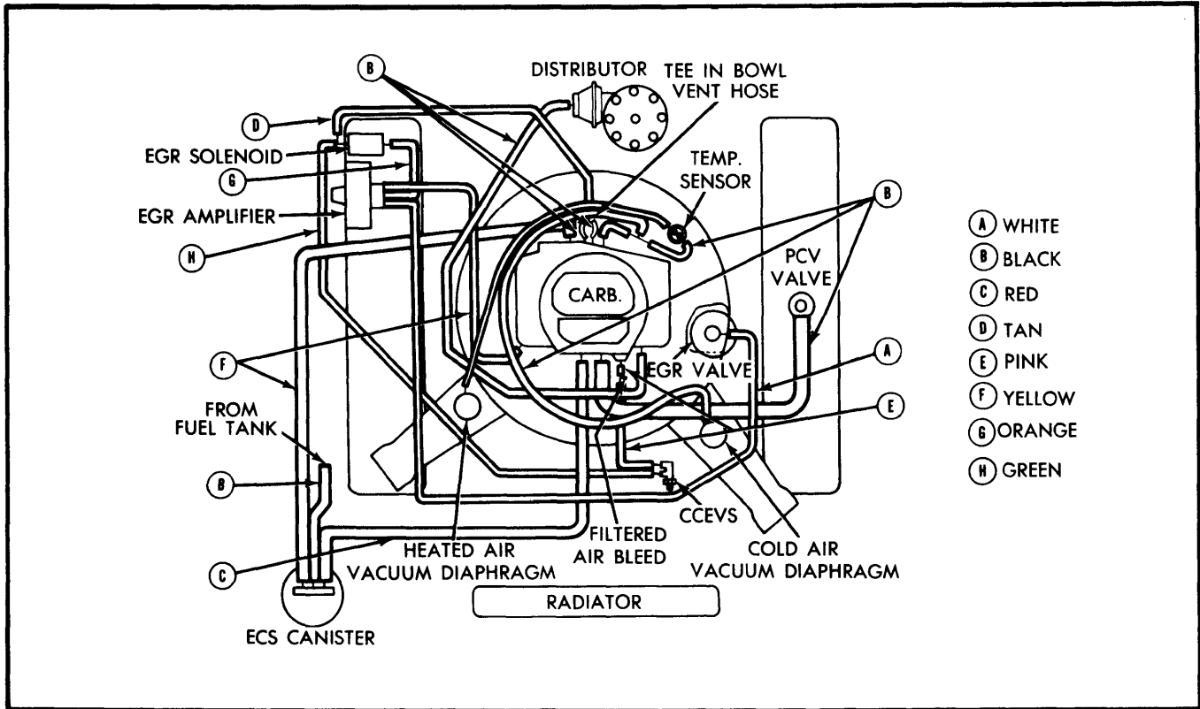
Fig. 7 360" V8 4-Barrel Federal Light Duty Emissions All Models
