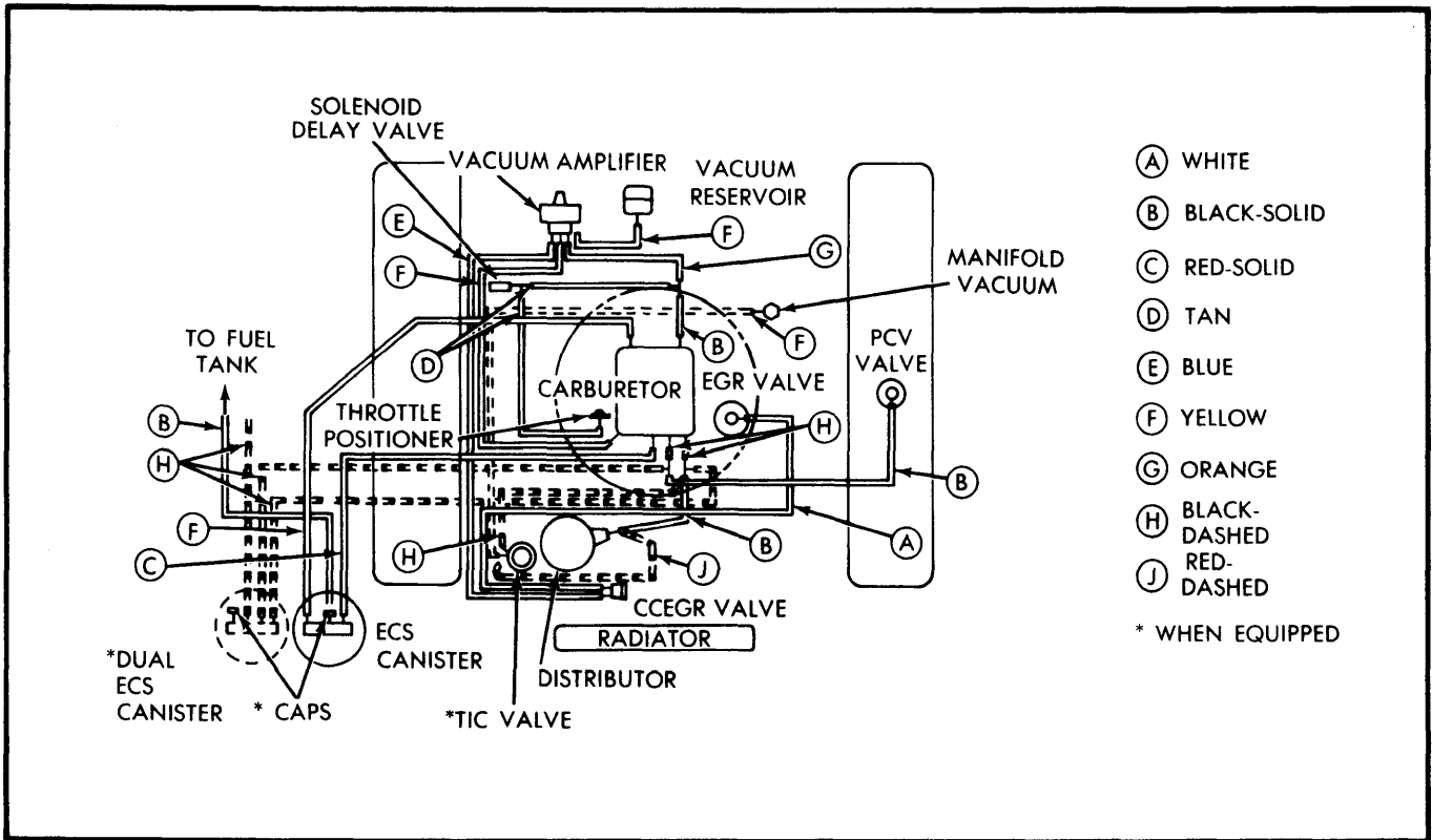
Fig. 11 440" V8 Heavy Duty Emissions Motor Home Chassis
