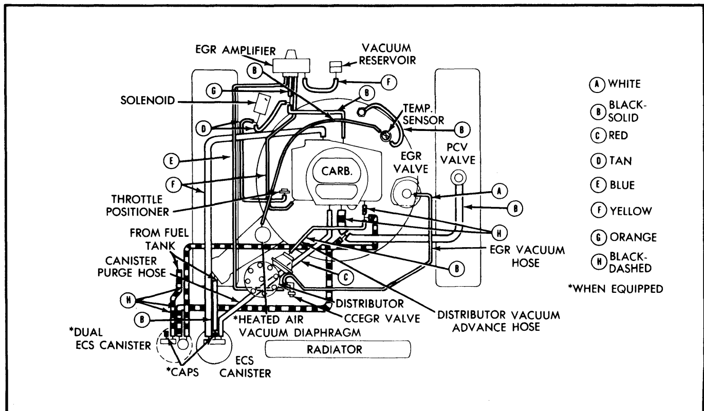
Fig. 10 440" V8 Heavy Duty Emissions All Models Exc. Motor Home Chassis
