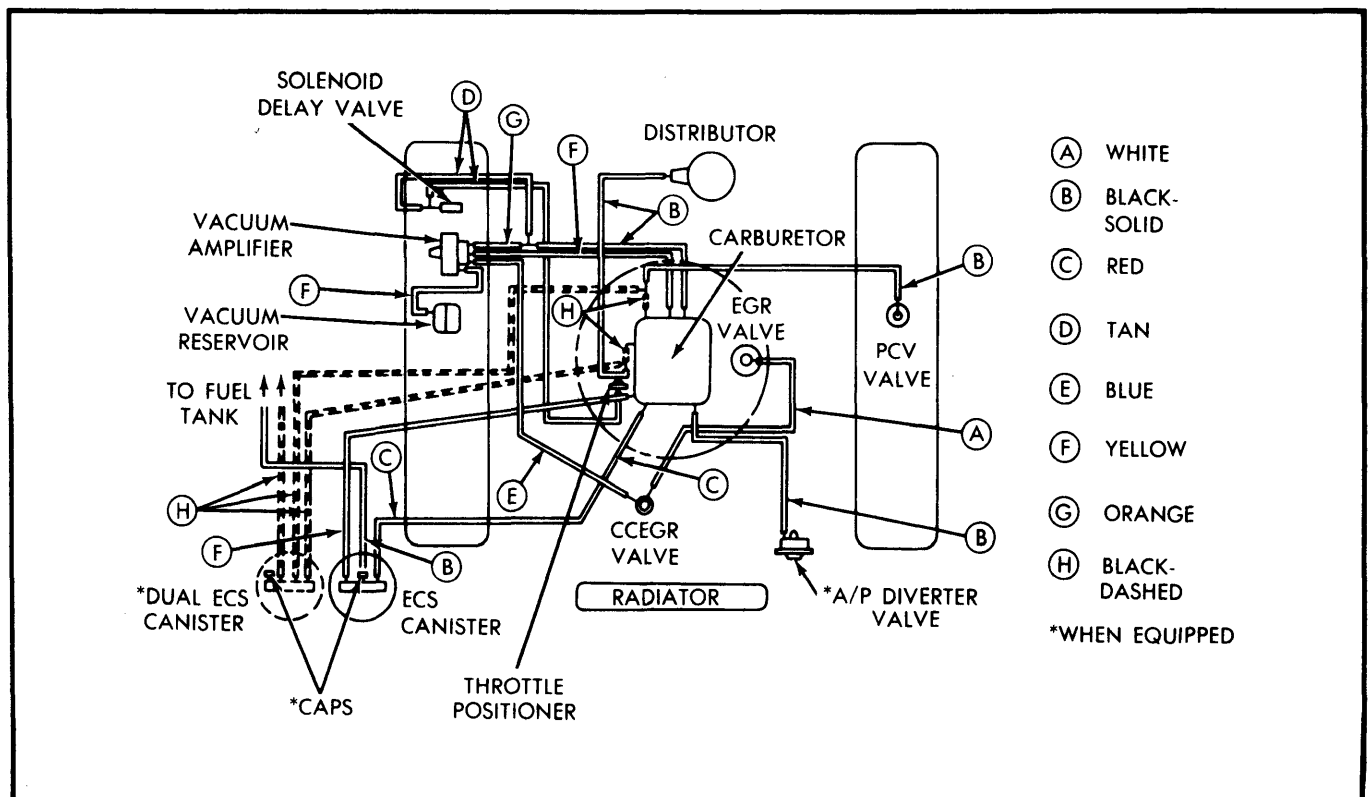
Fig. 6 360" V8 2-Barrel California Motor Home Chassis Models
