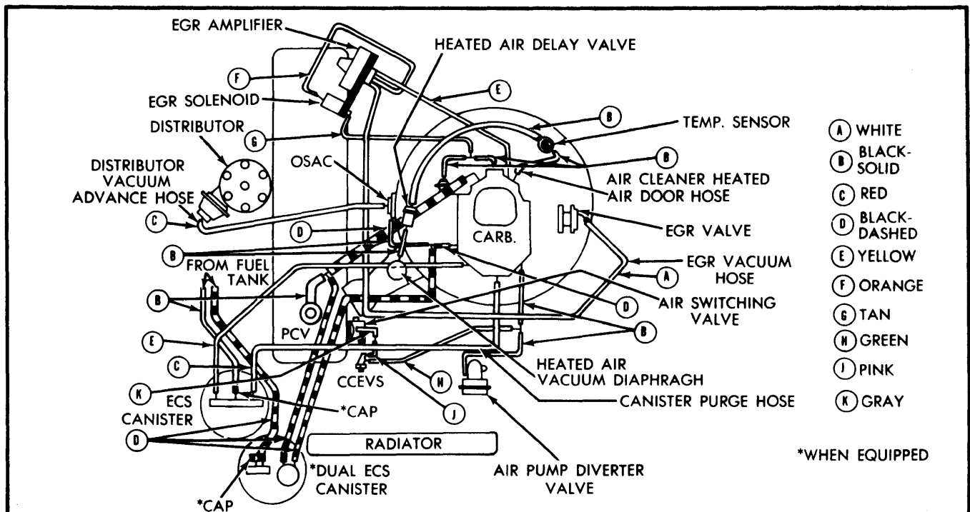
Fig. 2 225" 6 Cyl. California All Models
