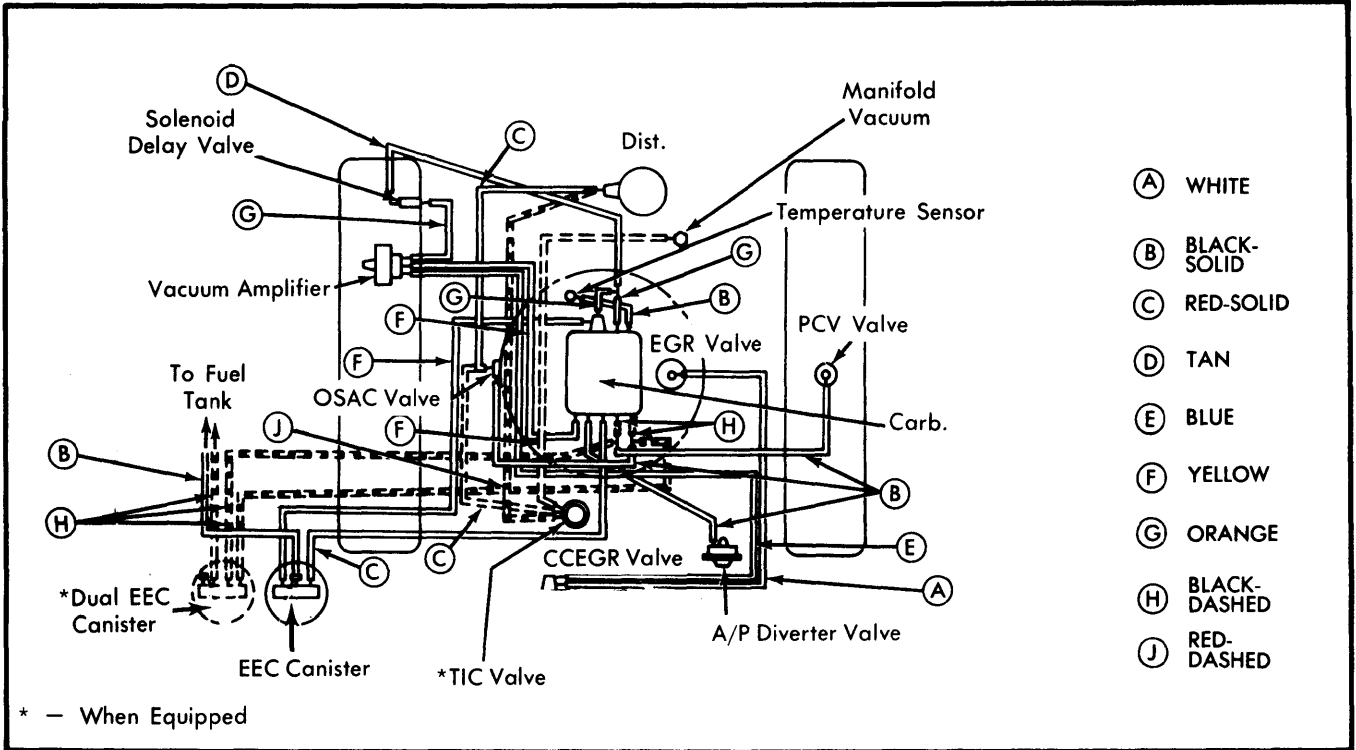
Fig. 11 Emission Vacuum Hose Routing for 360" 4-Bbl. Engines, Calif. Light Duty Vehicles (Voyager, Compact & Motor Homes Only)
