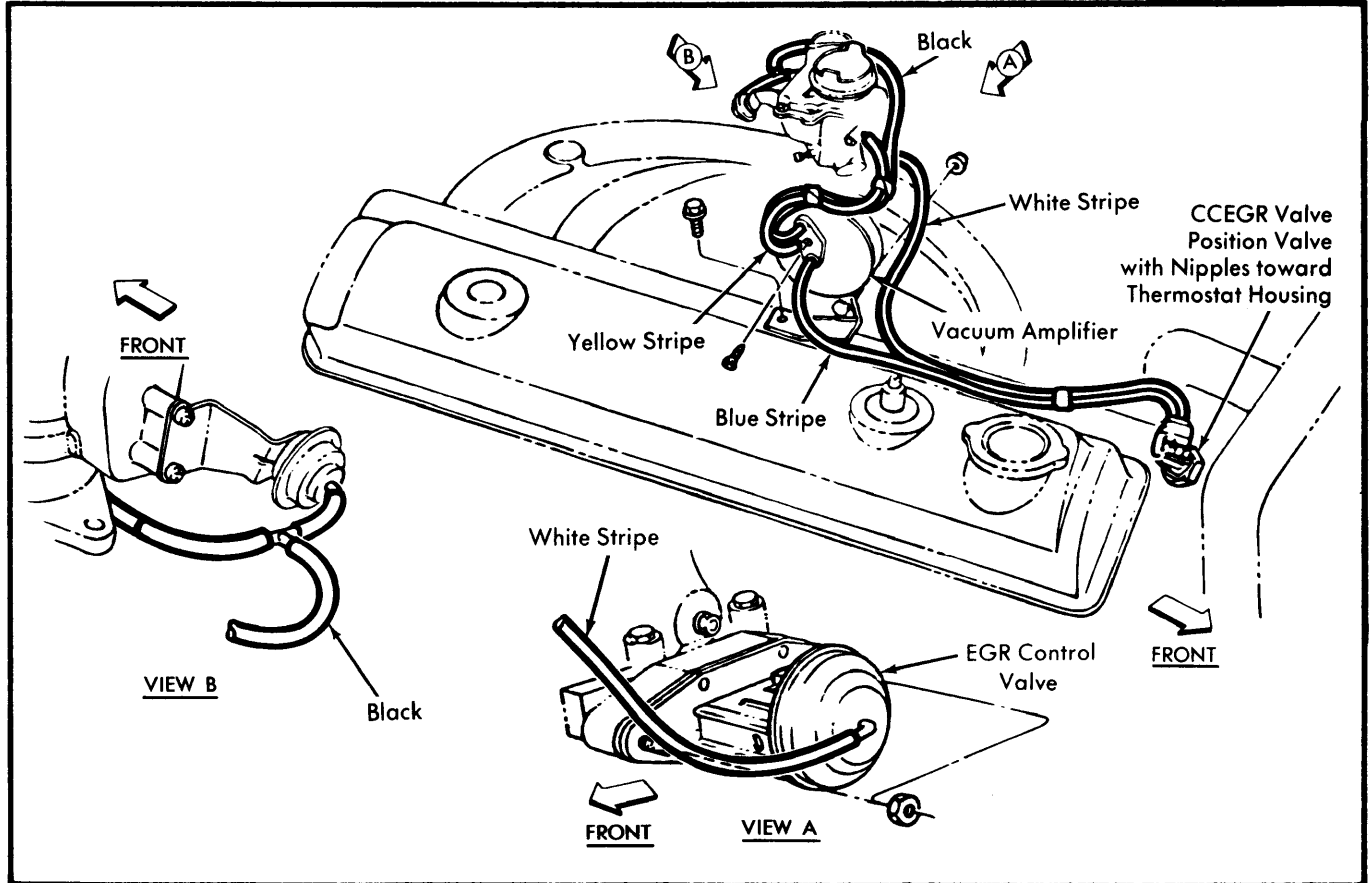
Fig. 3 EGR Vacuum Hose System for 225" Engine (Light Duty Cycle)
