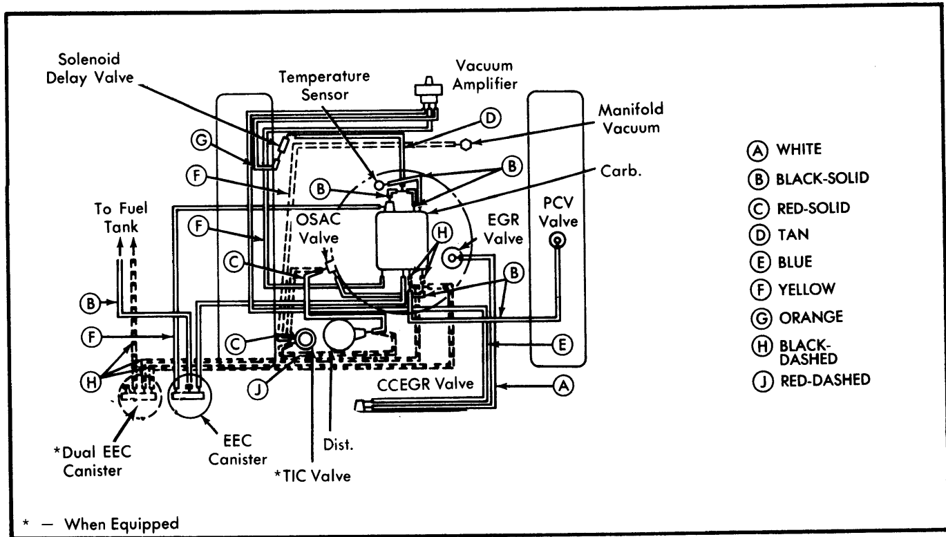
Fig. 13 Emission Vacuum Hose Routing for 440" Engines, Calif. Light Duty Vehicles (Voyager, Compact & Motor Homes)
