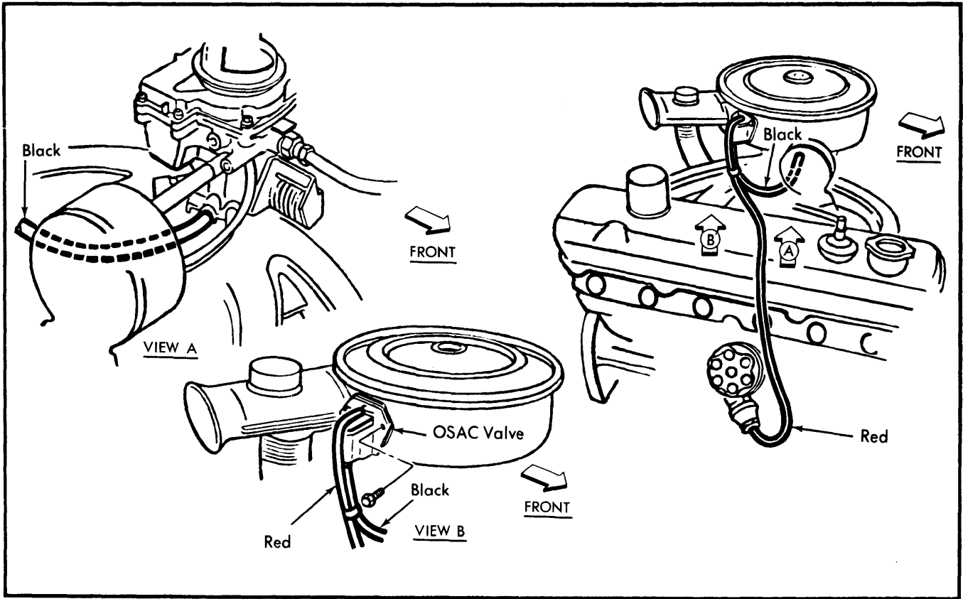
Fig. 1 OSAC Vacuum Hose System for 225" Engine (Light Duty Cycle)
