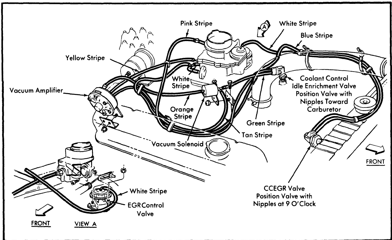
Fig. 6 EGR & Idle Enrichment Vacuum Hose System for Auto. Trans. 318 n Engines (Light Duty Cycle)
