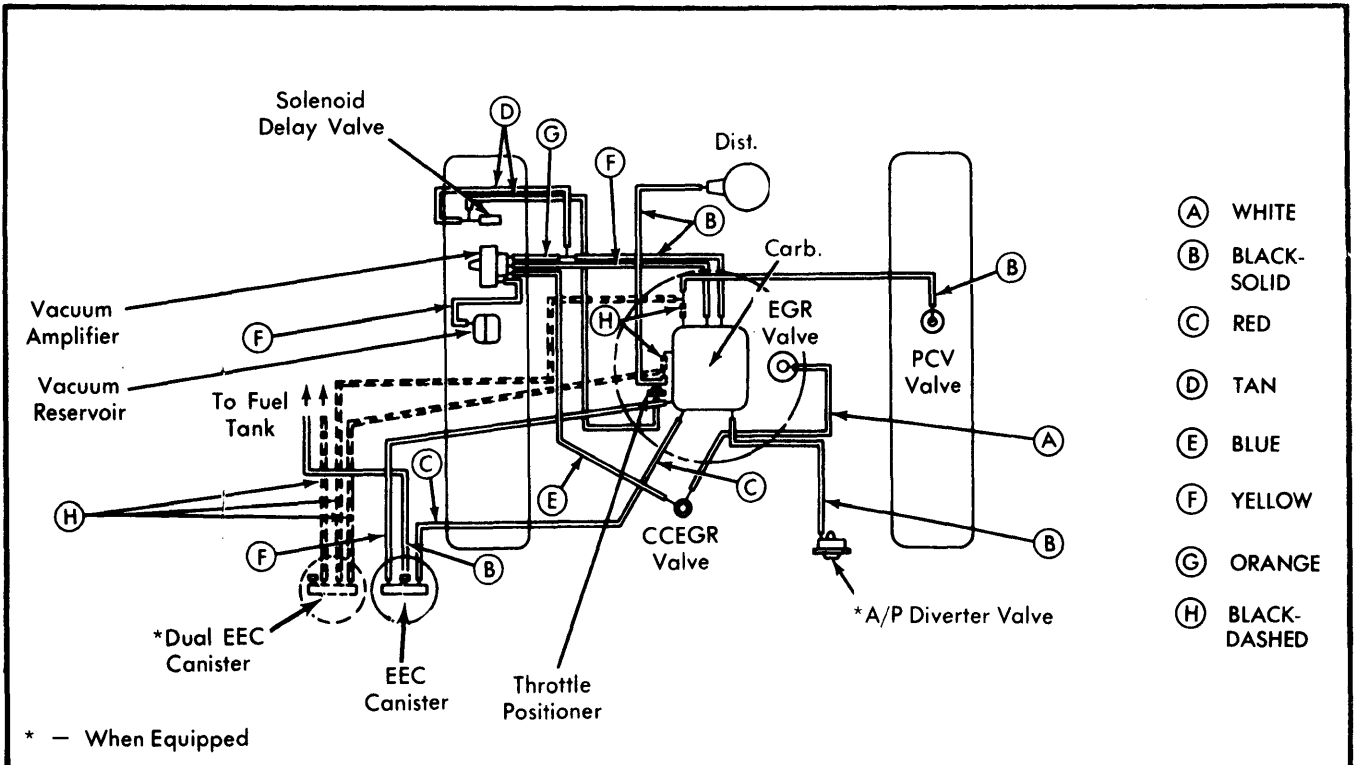
Fig. 12 Emission Vacuum Hose Routing for 360" 2-Bbl., Calif. Heavy Duty Vehicles (Voyager, Compact & Motor Homes Only)
