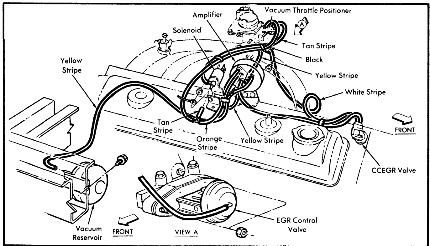
Fig. 4 EGR & Throttle Positioner Vacuum Hose System for 225" Engine (Heavy Duty Cycle Calif. Only)
