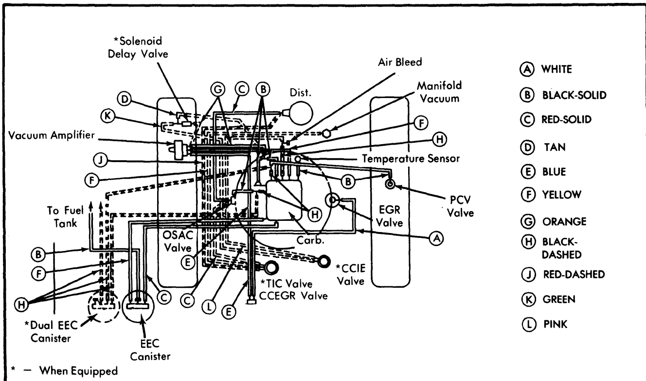
Fig. 10 Emission Vacuum Hose Routing for 318" & 360" 2-Bbl. Engines, Federal Light Duty Vehicles (Voyager, Compact & Motor Homes Only)
