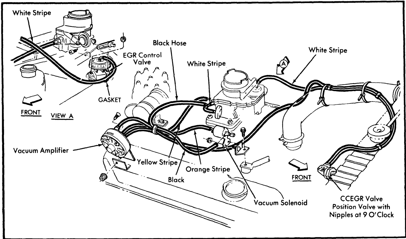
Fig. 5 EGR Vacuum Hose System for Man. Trans. 318 n Engines (Light Duty Cycle)
