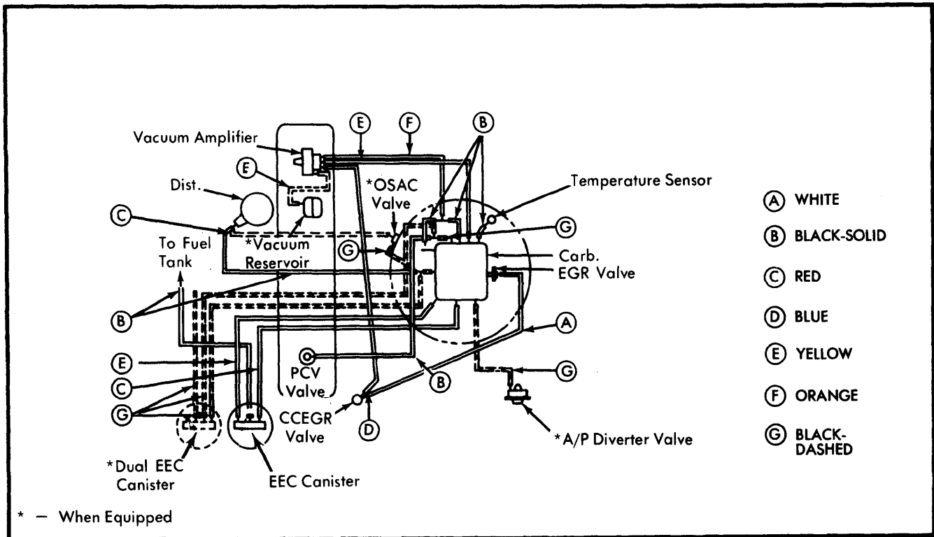
Fig. 9 Emission Vacuum House Routing for 225" Engines, Light Duty Vehicles (Voyager, Compact & Motor Homes Only)
