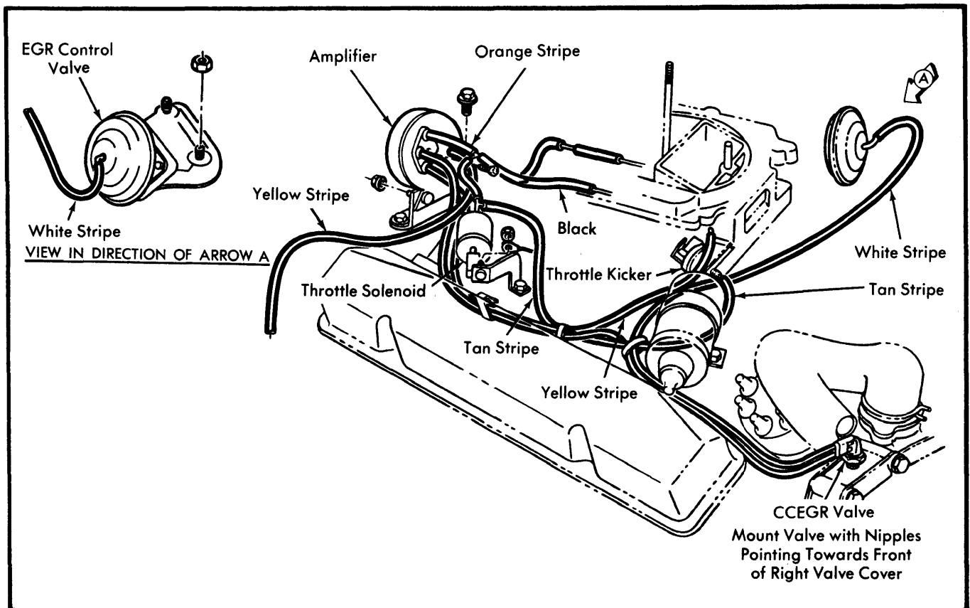
Fig. 8 EGR Vacuum Hose System for 440" Engine (Heavy Duty Cycle Calif. Only)
