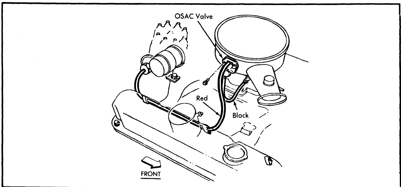
Fig. 2 OSAC Vacuum Hose System for 318" & 360" Engines (Light Duty Cycle)
