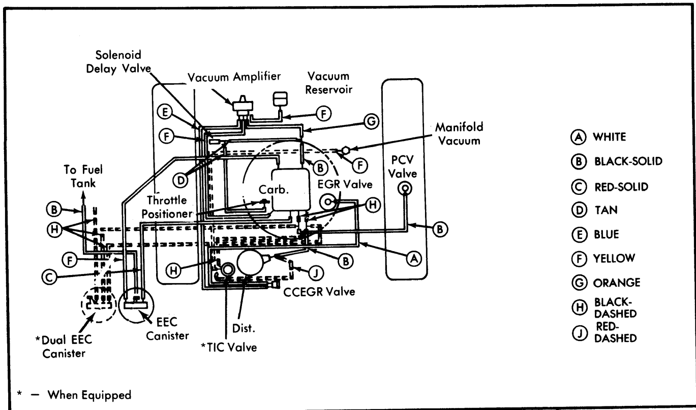
Fig. 14 Emission Vacuum Hose Routing for 440" Engines, Calif. Heavy Duty Vehicles (Voyager, Compact & Motor Homes Only)
