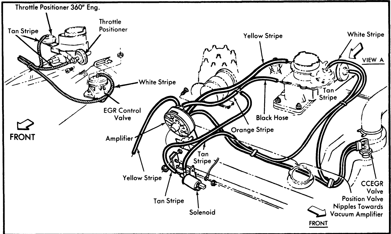
Fig. 7 EGR Vacuum Hose System for 318" & 360" Engines (Heavy Duty Cycle Calif. Only)
