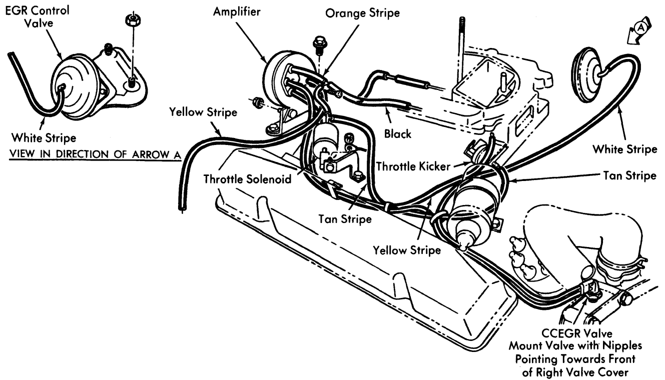
Fig. 9 EGR Vacuum Hose System for 440" Engine (Heavy Duty Cycle California Only)
