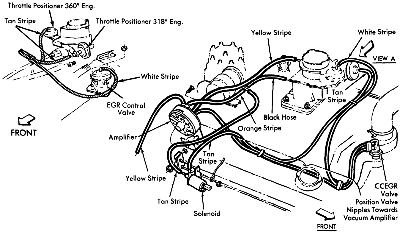
Fig. 7 EGR Vacuum Hose System for 318" & 360" Engines (Heavy Duty Cycle California Only)
