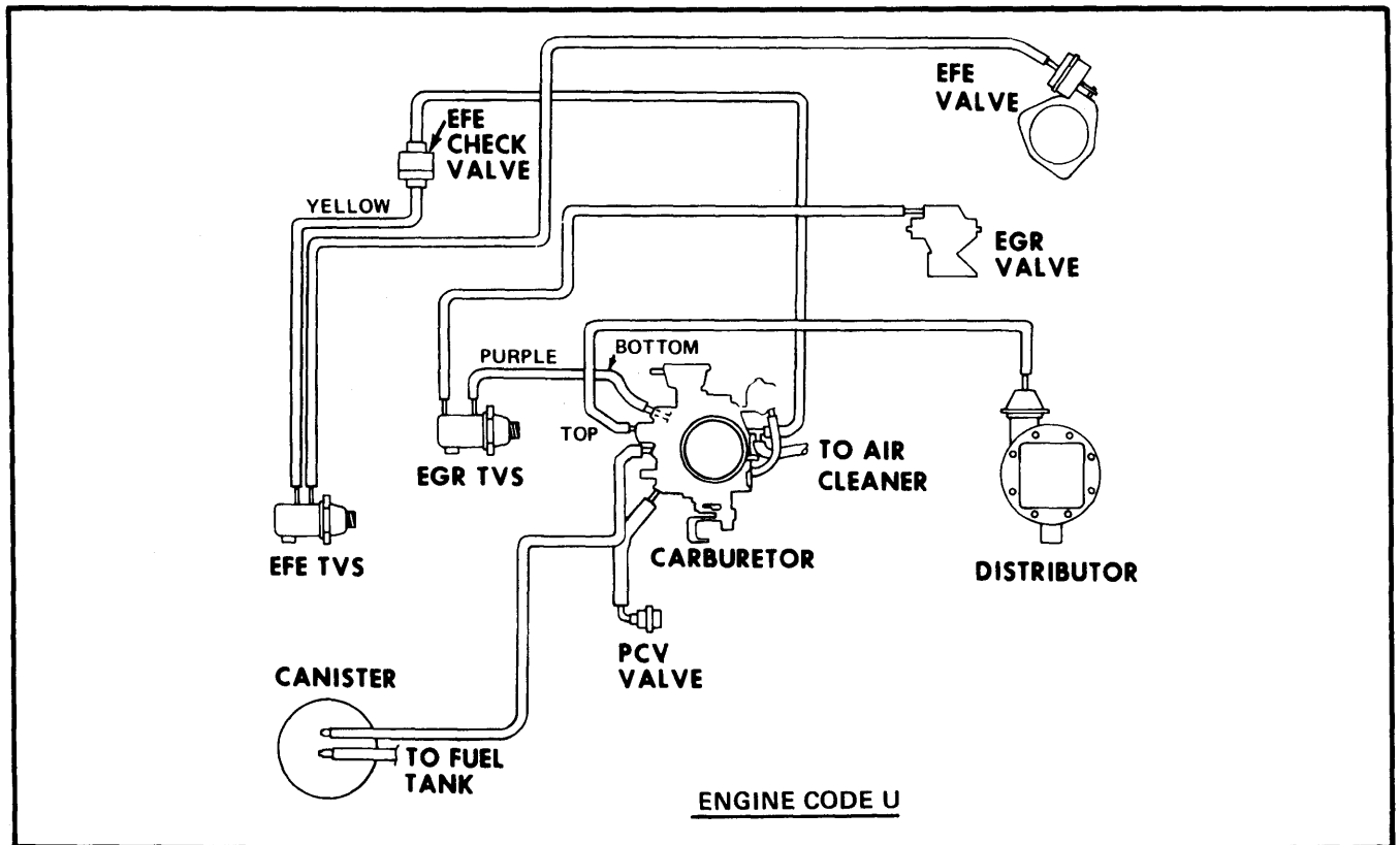
Fig. 6 305 CID Vacuum Hose Routing (Federal)
