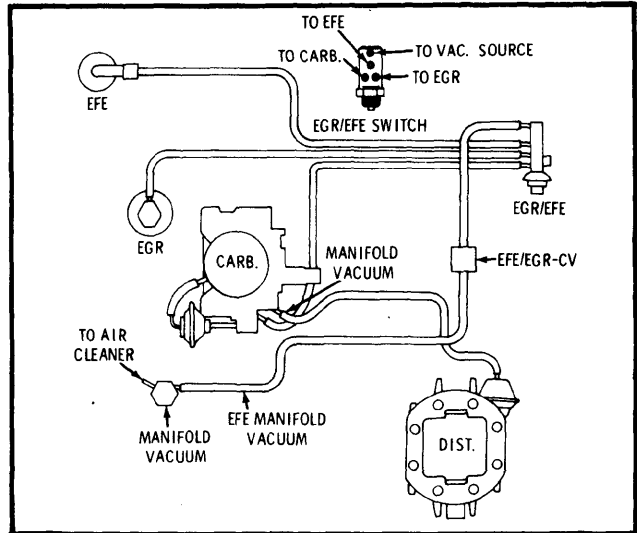
Fig. 2 231 CID Vacuum Hose Routing (Federal)
