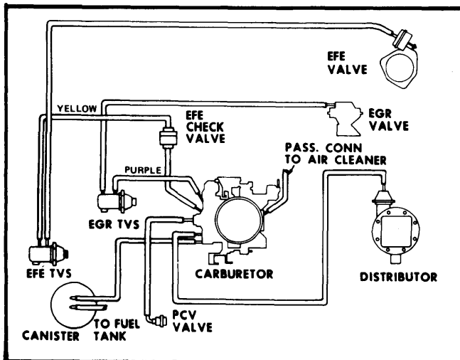
Fig. 11 88 350 CID VIN "L" Vac. Hose Routing (Federal)
