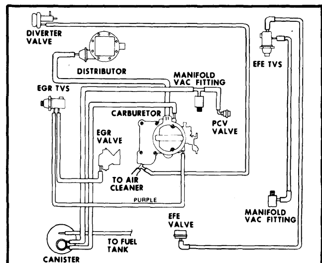
Fig. 6 All Models 250 CID Vacuum Hose Routing (Calif.)
