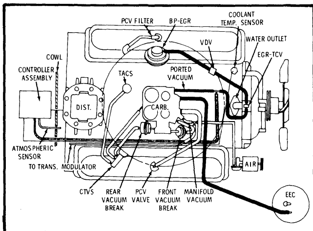
Fig. 17 Toronado 403 CID Vacuum Hose Routing (Calif.)
