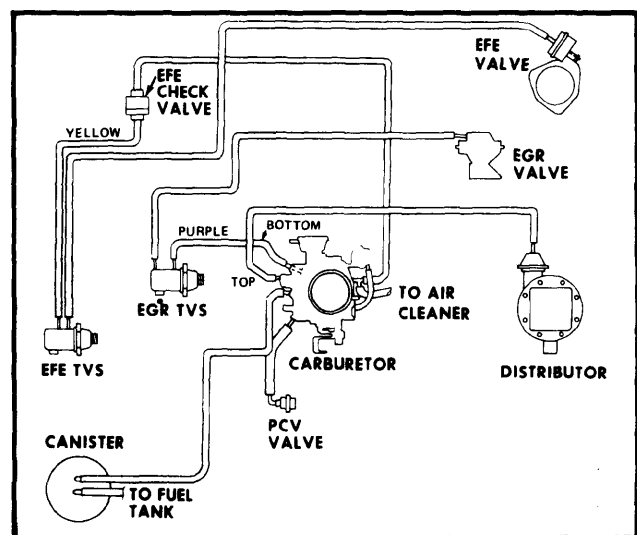
Fig. 6 Starfire 305 CID Vacuum Hose Routing (Federal)
