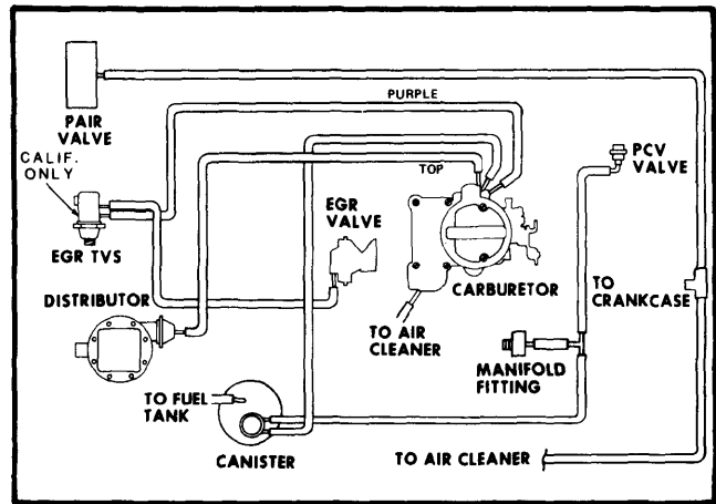
Fig. 2 Chevette Vacuum Hose Routing (High Alt. & Calif.)
