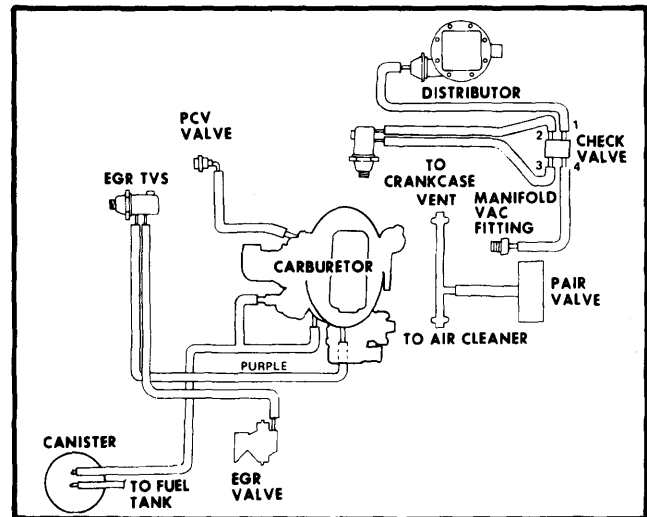
Fig. 4 Vega & Monza 140 CID Vacuum Hose Routing (High Alt. & Calif.)
