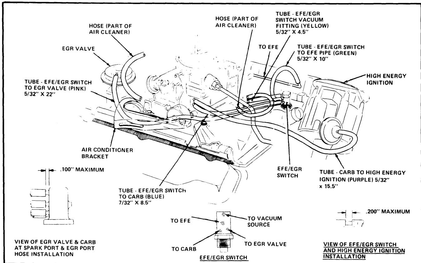
Fig. 8 350 CID Engine Code "H" Vacuum Hose Routing (Federal)
