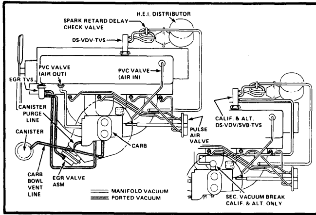
Fig. 1 140 CID Vacuum Hose Routing (All States)
