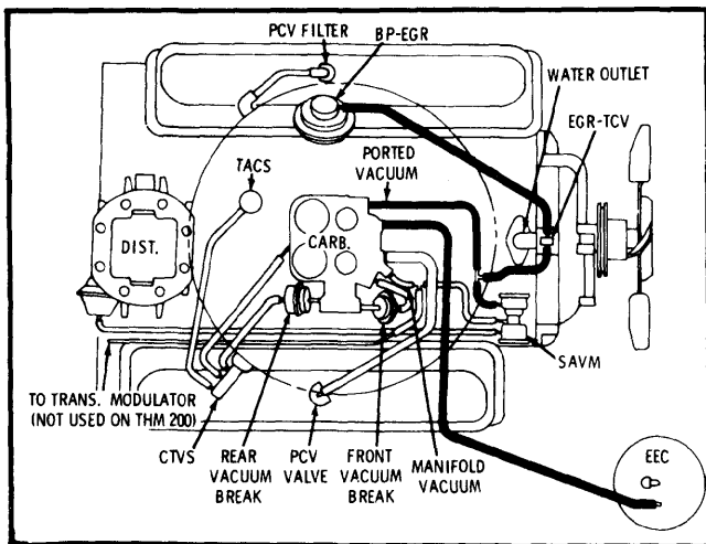
Fig. 15 403 CID Vacuum Hose Routing (Federal)
