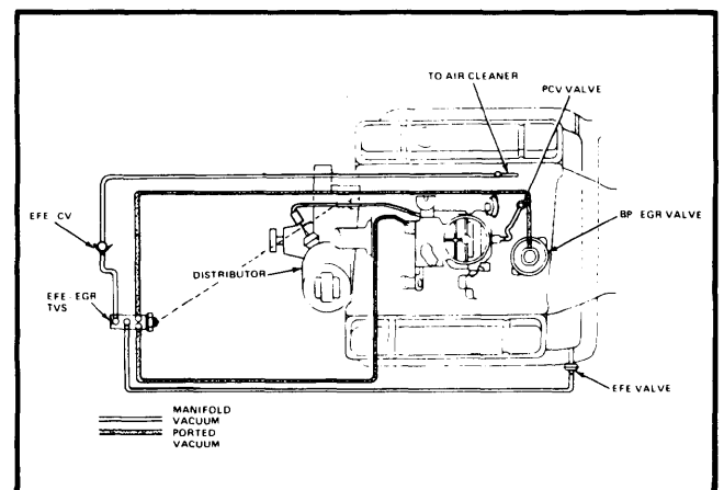
Fig. 6 231 CID Vacuum Hose Routing (Federal)
