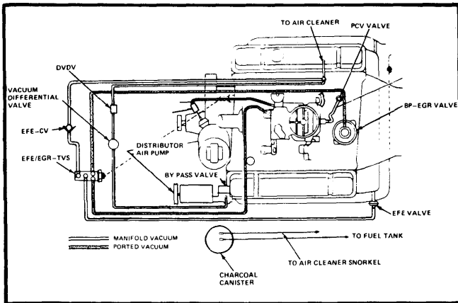
Fig. 9 231 CID Vacuum Hose Routing (Calif. w/Auto. Trans.)
