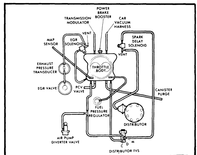
Fig. 6 425 CID with EFI Vacuum Hose Routing (Fed. & High Alt.)
