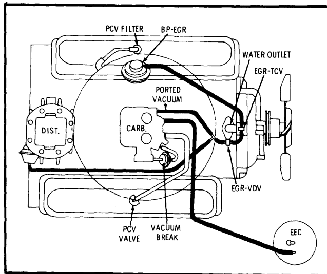
Fig. 5 260 CID w/5-Speed Man. Trans. Vacuum Hose Routing (Federal)
