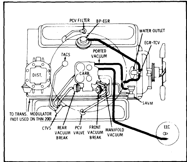
Fig. 13 403 CID Late Production Vacuum Hose Routing (Federal)
