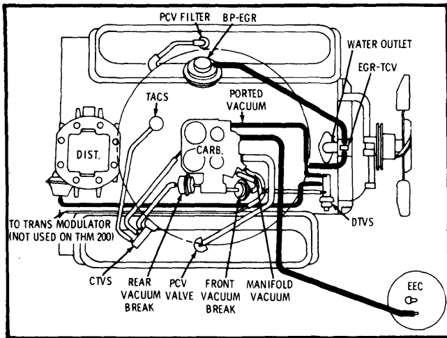
Fig. 13 350 & 403 CID VIN "R" Vacuum Hose Routing (High Altitude)
