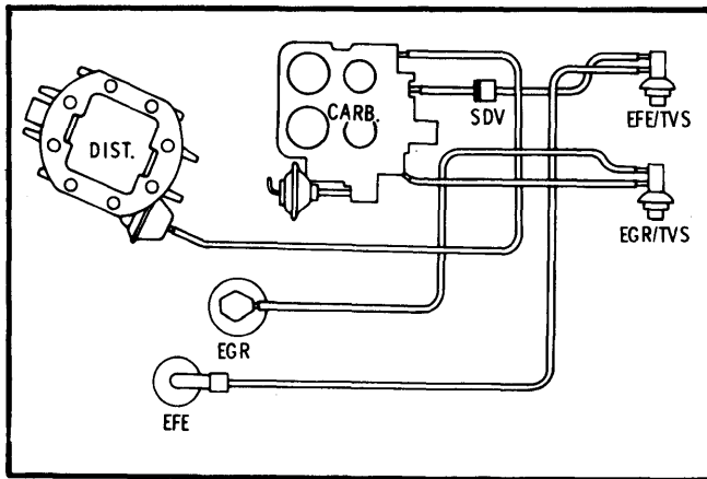
Fig. 9 Omega 350 CID VIN "L" Vac. Hose Routing (Federal)
