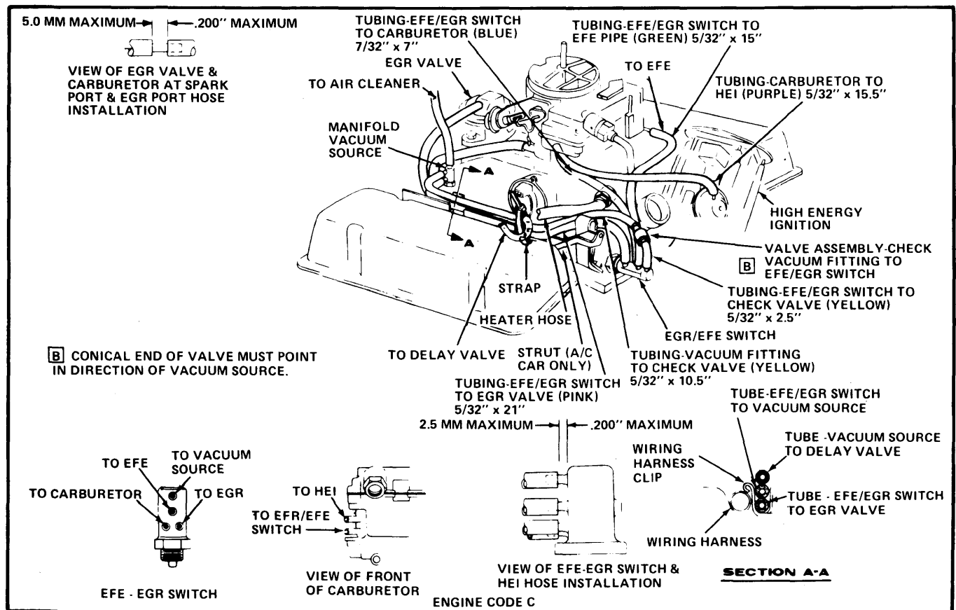
Fig. 2 231 CID Vacuum Hose Routing (High Alt. & Calif.)
