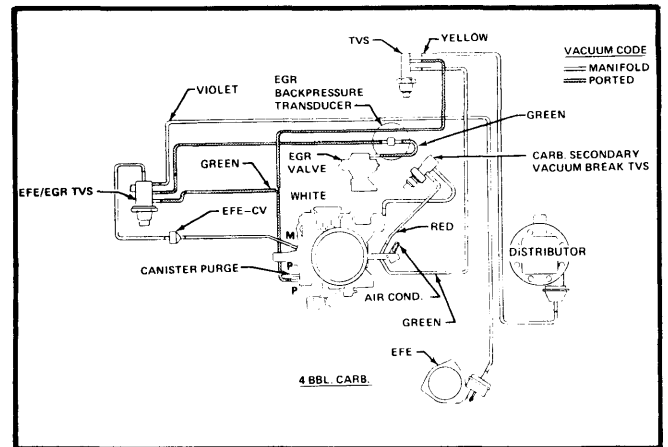
Fig. 14 400 CID Vacuum Hose Routing (Federal w/Man Trans.)
