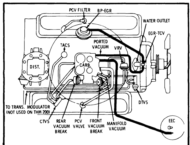
Fig. 12 350 CID VIN "R" Vacuum Hose Routing (Federal)
