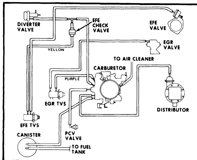
Fig. 11 All Models 350 CID Vacuum Hose Routing (High Alt. & Calif.)
