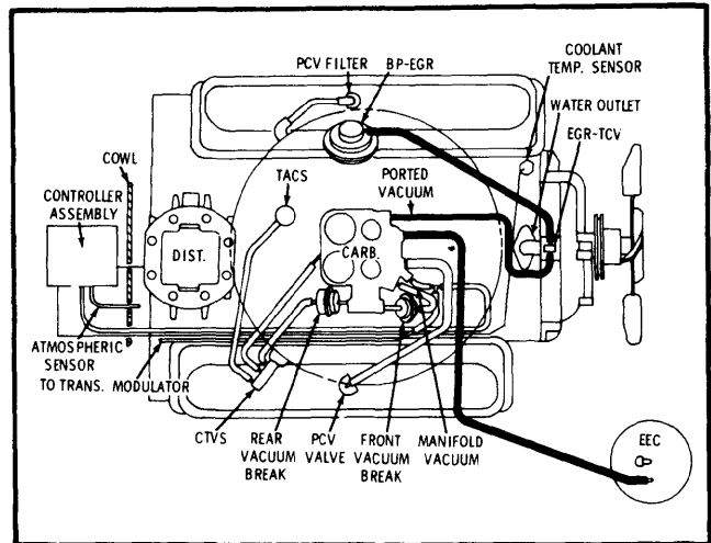
Fig. 16 Toronado 403 CID Vacuum Hose Routing (Federal)
