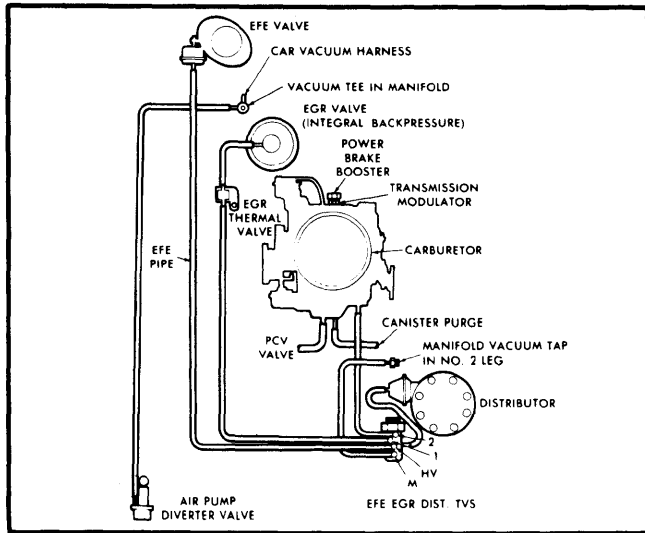
Fig. 1 425 CID without EFI Vacuum Hose Routing (Calif.)
