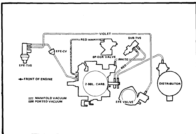
Fig. 11 301 CID Vacuum Hose Routing (Federal Auto. Trans. without A/C)
