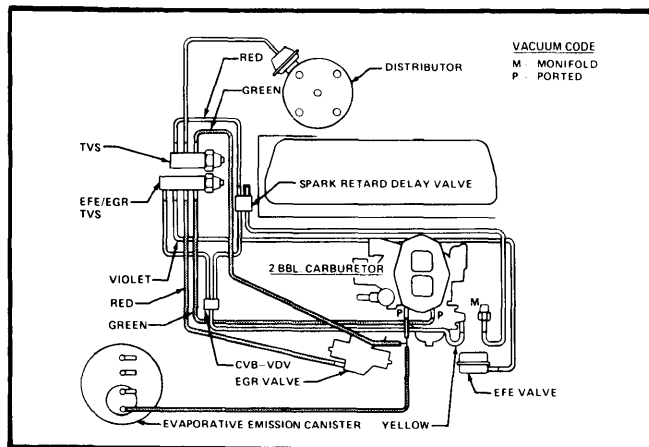
Fig. 5 151 CID Vacuum Hose Routing (Federal with Auto. Trans. & A/C)
