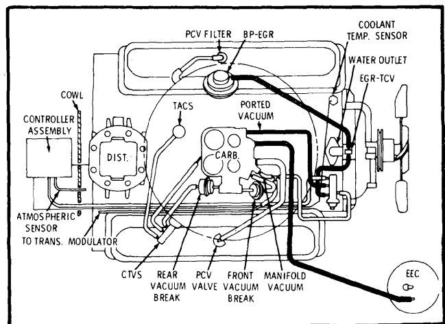
Fig. 18 Toronado 403 CID Vacuum Hose Routing (High Alt.)
