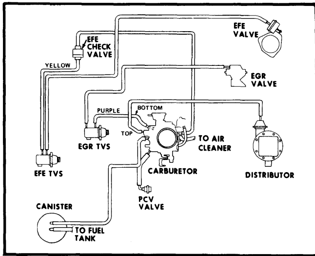
Fig. 7 All Models 305 CID Vacuum Hose Routing (Federal)
