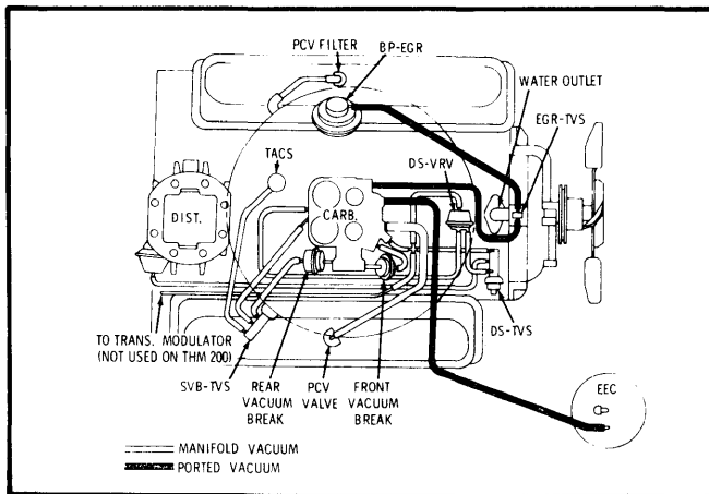
Fig. 15 350 & 403 CID VIN "R" & "K" Vac. Hose Routing (Federal)
