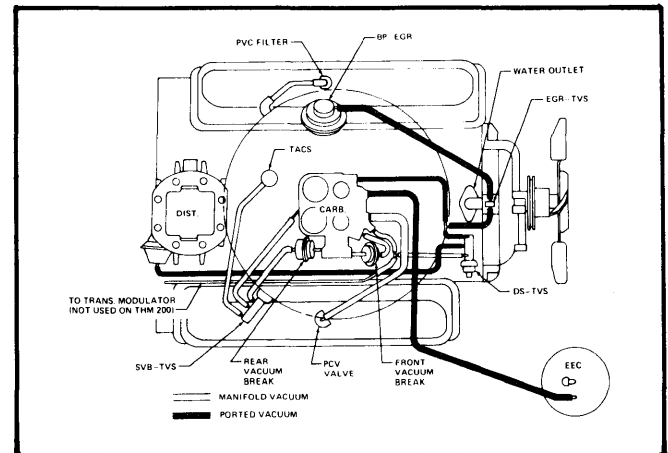
Fig. 16 350 & 403 CID VIN "R" & "K" Vac. Hose Routing (High Altitude)
