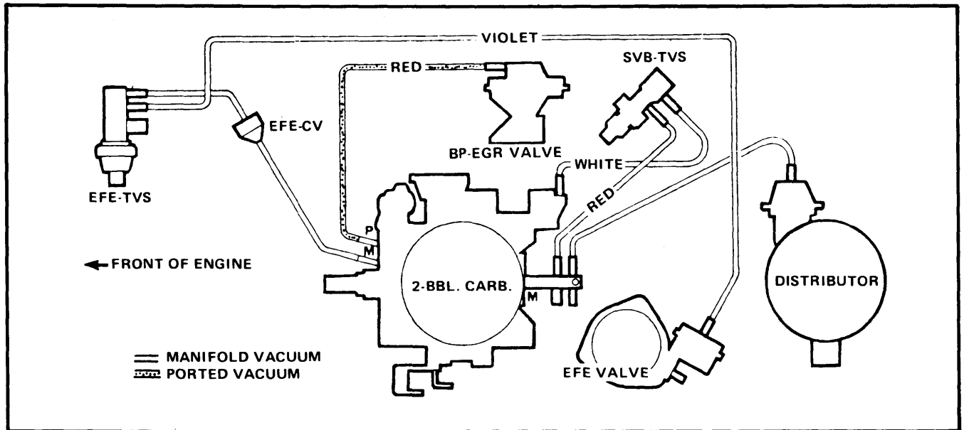
Fig. 5 301 CID Auto. Trans. without A/C Vacuum Hose Routing (Federal)
