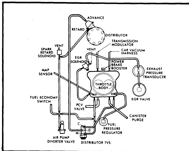
Fig. 5 425 CID with EFI Vacuum Hose Routing (Calif.)
