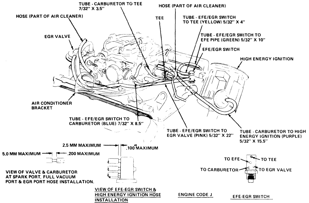
Fig. 9 350 CID Engine Code "J" Vacuum Hose Routing (Federal)
