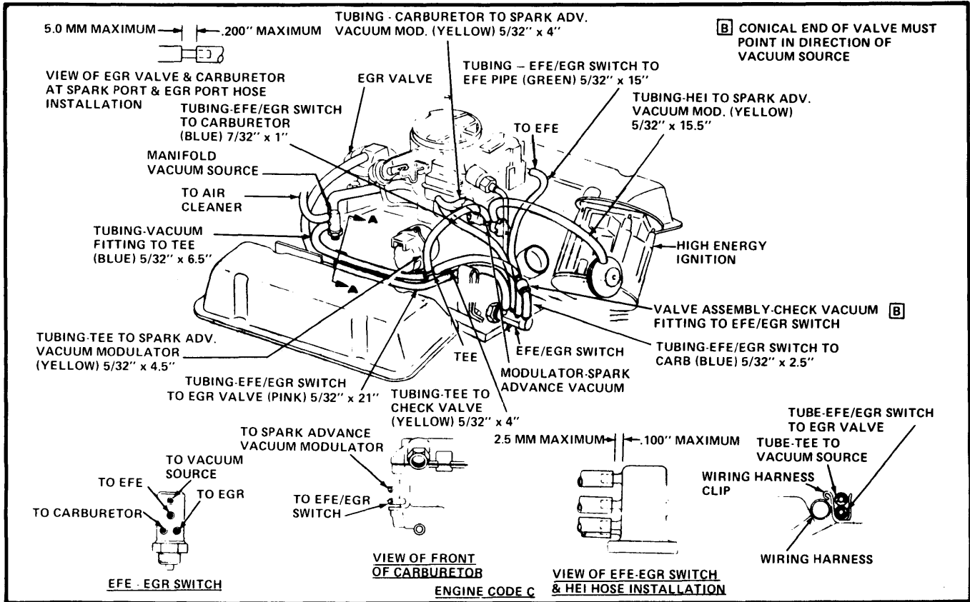
Fig. 3 231 CID "Economy Special" Vacuum Hose Routing
