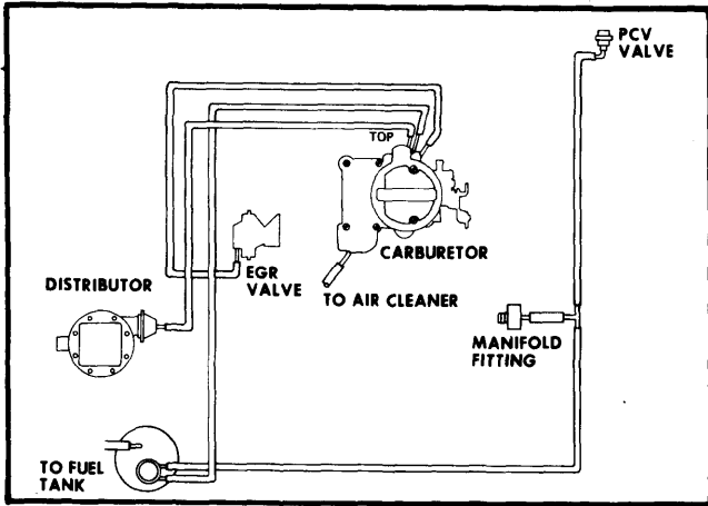
Fig. 1 Chevette Vacuum Hose Routing (Federal)
