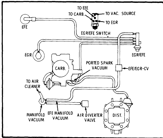
Fig. 3 231 CID Vacuum Hose Routing (High Alt. & Calif.)
