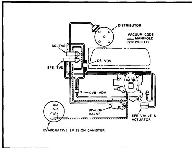
Fig. 3 151 CID Vacuum Hose Routing (Calif. with Auto. Trans. & A/C)
