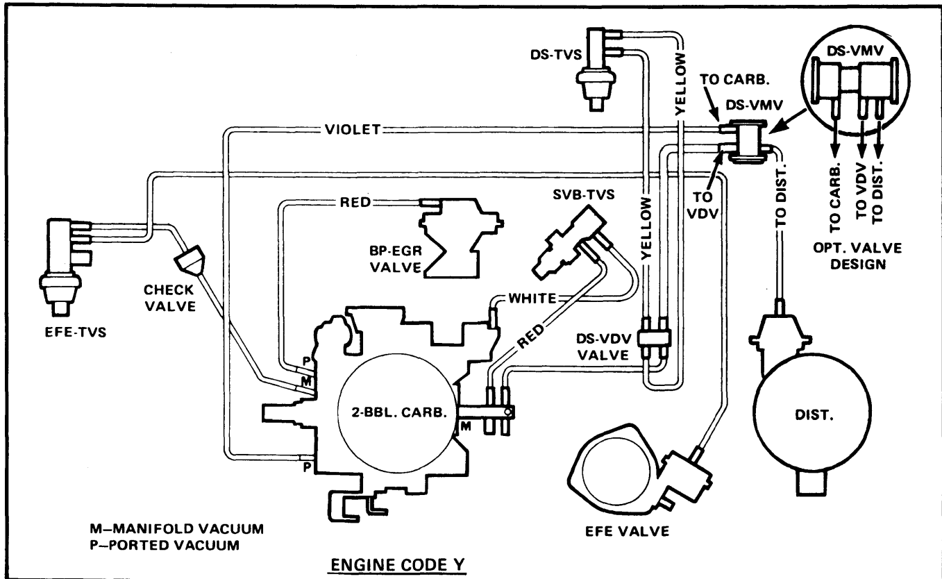
Fig. 4 301 CID Auto. Trans. with A/C Vacuum Hose Routing (Federal)
