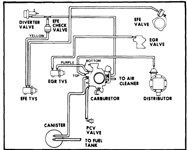
Fig. 8 All Models 305 CID Vacuum Hose Routing (High Alt.)
