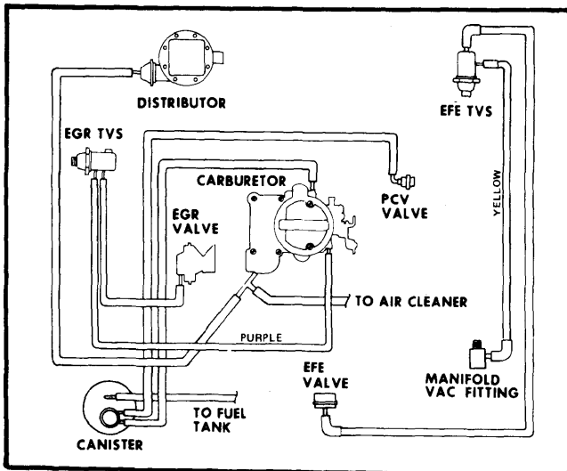
Fig. 5 All Models 250 CID Vacuum Hose Routing (Fed. & High Alt.)
