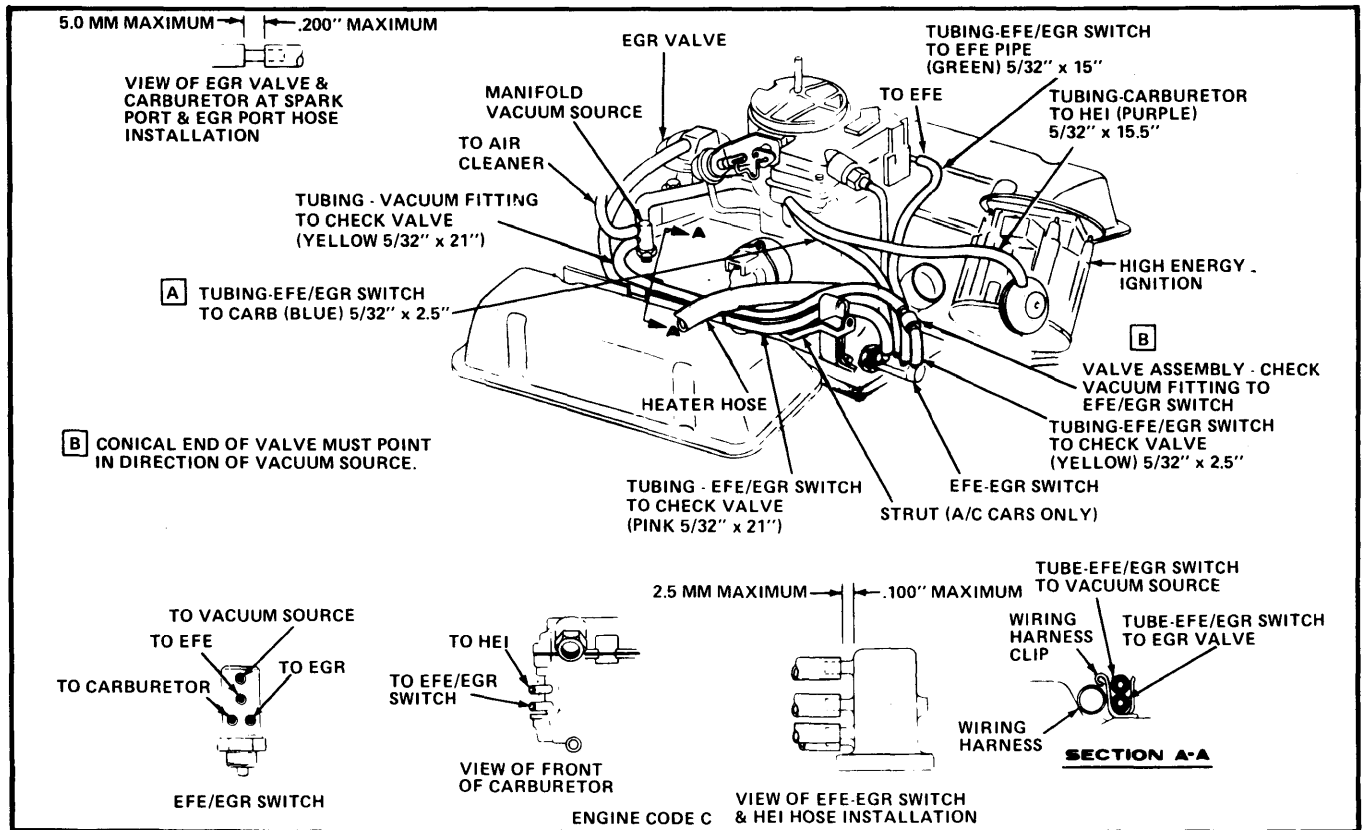
Fig. 1 231 CID Vacuum Hose Routing (Federal)
