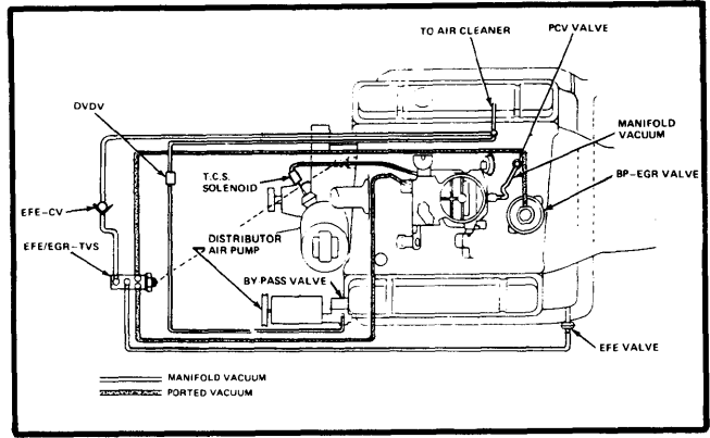
Fig. 8 231 CID Vacuum Hose Routing (Calif. w/Man. Trans.)
