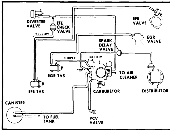
Fig. 9 All Models 305 CID Vacuum Hose Routing (Calif.)
