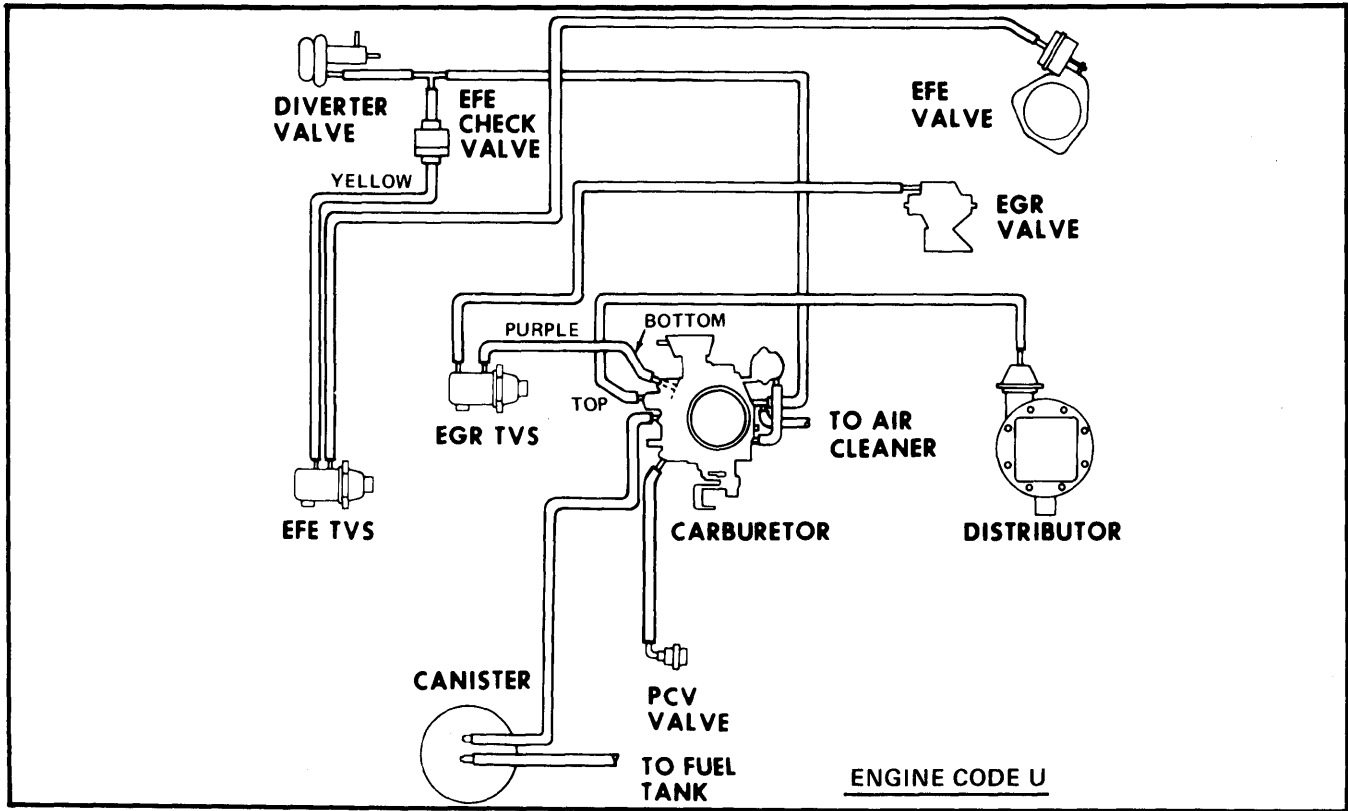
Fig. 7 305 CID Vacuum Hose Routing (High Altitude)
