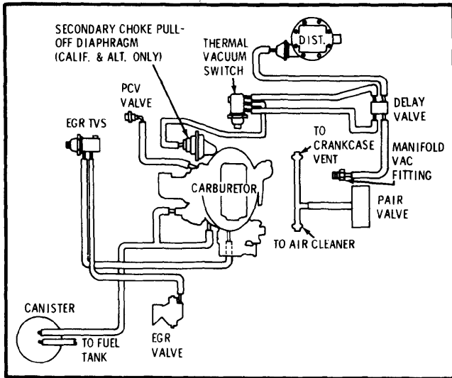
Fig. 1 140 CID Vacuum Hose Routing (All)
