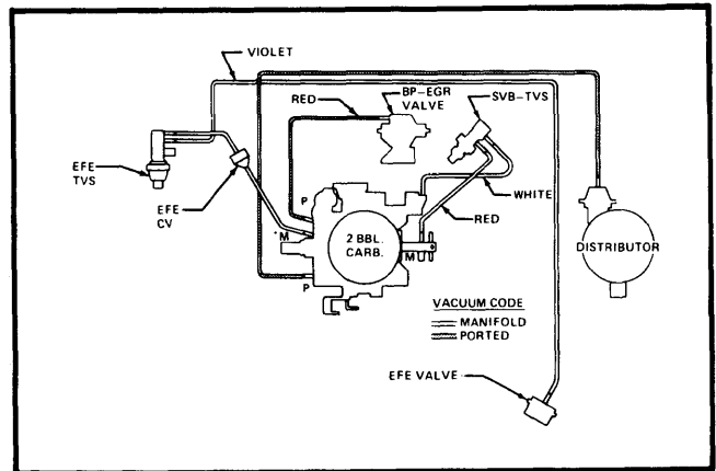
Fig. 10 301 CID Vacuum Hose Routing (Federal w/Man. Trans.)
