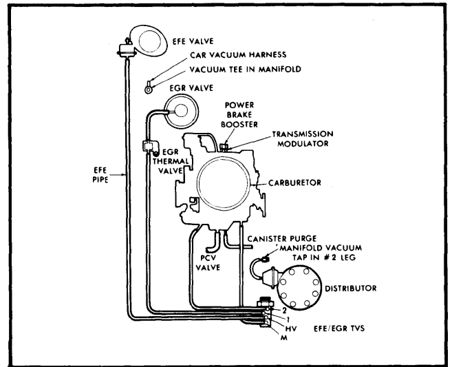
Fig. 2 425 CID without EFI Vacuum Hose Routing (Fed. & High Alt.)
