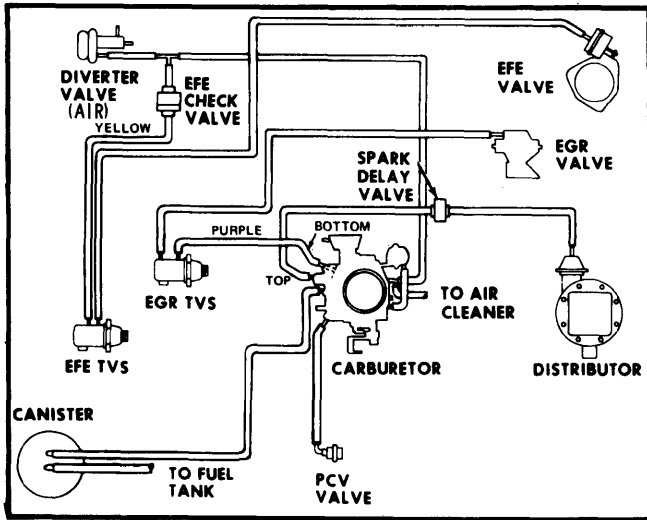
Fig. 7 Starfire 305 CID Vacuum Hose Routing (High Alt. & Calif.)
