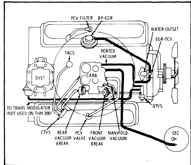
Fig. 15 305 & 403 CID Engine Code "K" & "R" Vacuum Hose Routing (High Alt.)
