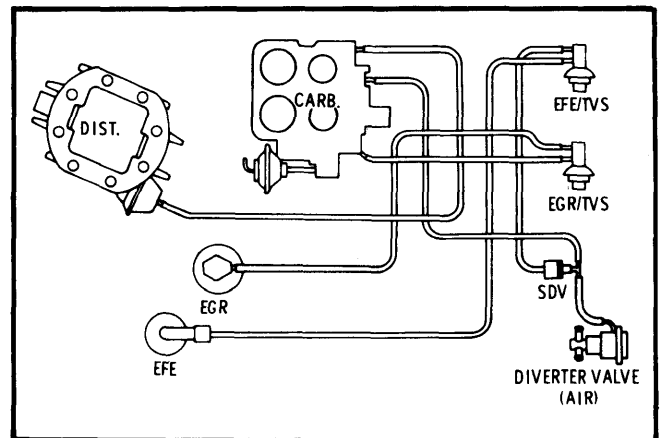
Fig. 10 Omega 350 CID VIN "L" Vac. Hose Routing (High Altitude & California)
