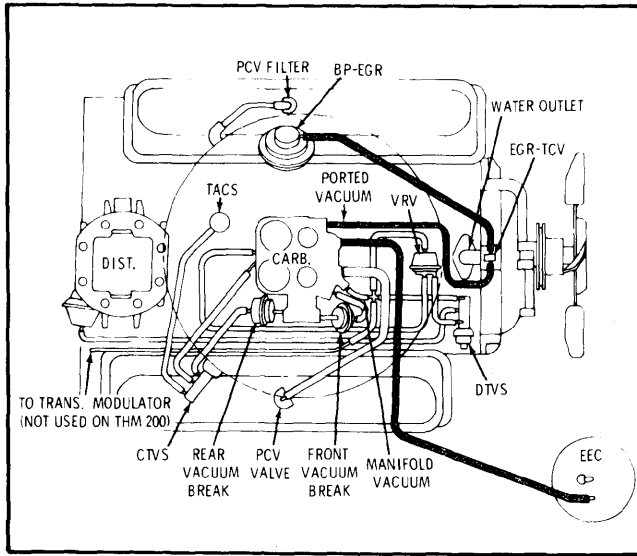
Fig. 12 350 & 403 CID Engine Code "R" Vacuum Hose Routing (Federal)
