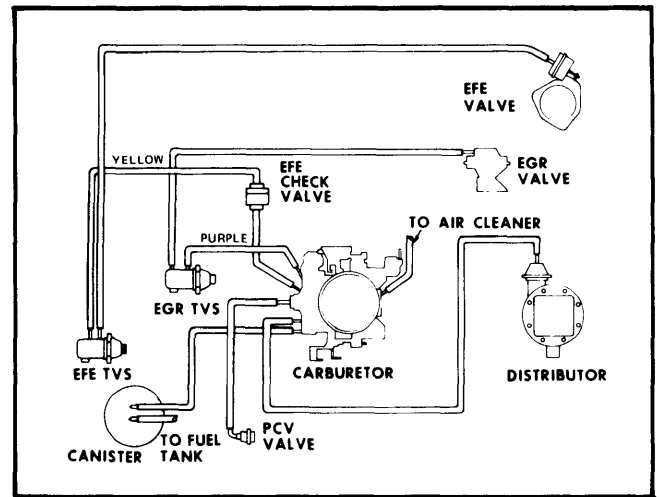
Fig. 10 All Models 350 CID Vacuum Hose Routing (Federal)
