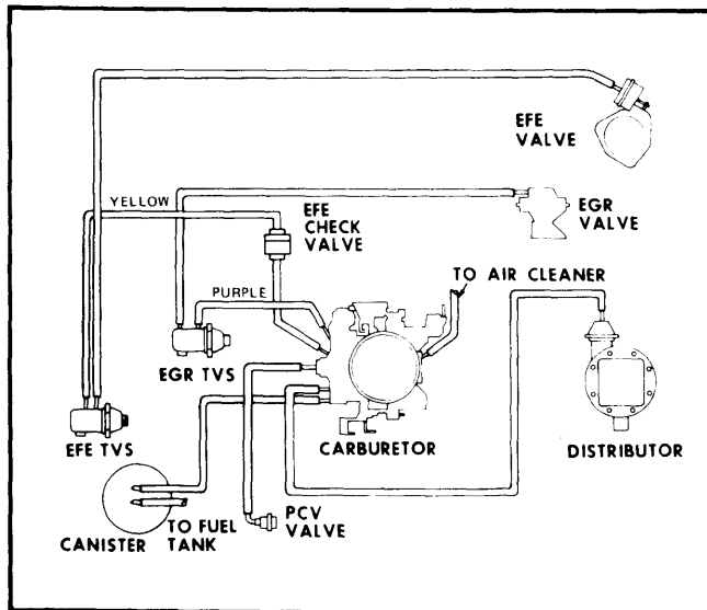
Fig. 10 350 CID Engine Code "L" Vacuum Hose Routing (Federal)
