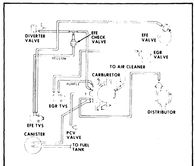
Fig. 11 350 CID Engine Code "L" Vacuum Hose Routing (High Alt. & Calif.)
