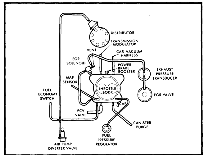
Fig. 4 350 CID with EFI Vacuum Hose Routing (Fed. & High Alt.)
