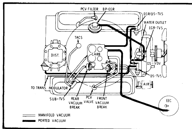
Fig. 17 350 & 403 CID VIN "R" & "K" Vac. Hose Routing (Calif.)
