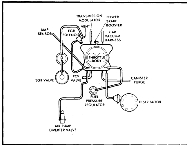
Fig. 3 350 CID with EFI Vacuum Hose Routing (Calif.)
