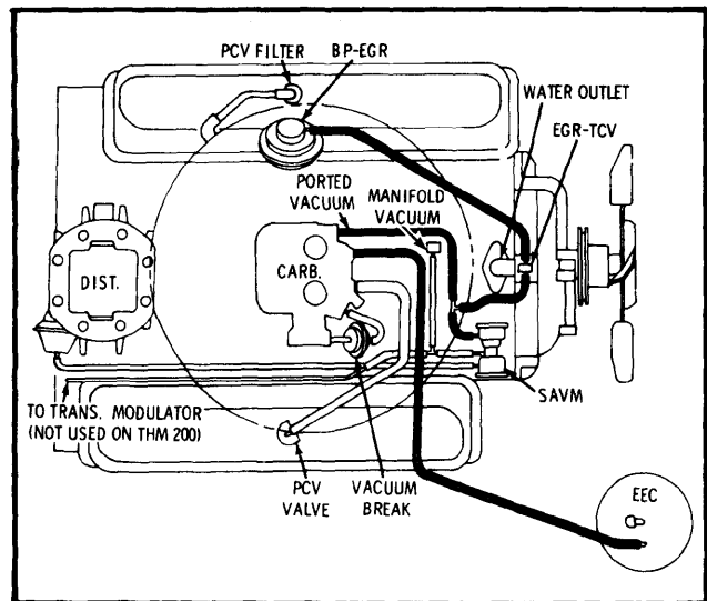
Fig. 4 260 CID Vacuum Hose Routing (Federal)
