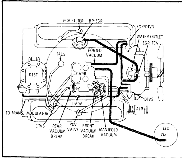
Fig. 14 350 & 403 CID Engine Code "K" & "R" Vacuum Hose Routing (California)
