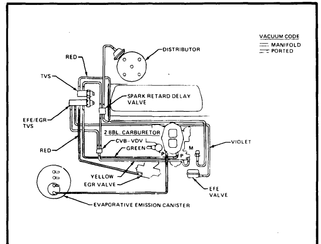
Fig. 4 151 CID Vacuum Hose Routing (Federal with Man. Trans. & Auto. Trans., non-A/C)
