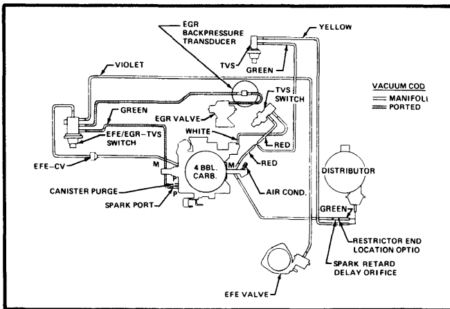
Fig. 13 350 & 400 CID VIN "P" & "Z" Vac. Hose Routing (Federal with Auto. Trans.)
