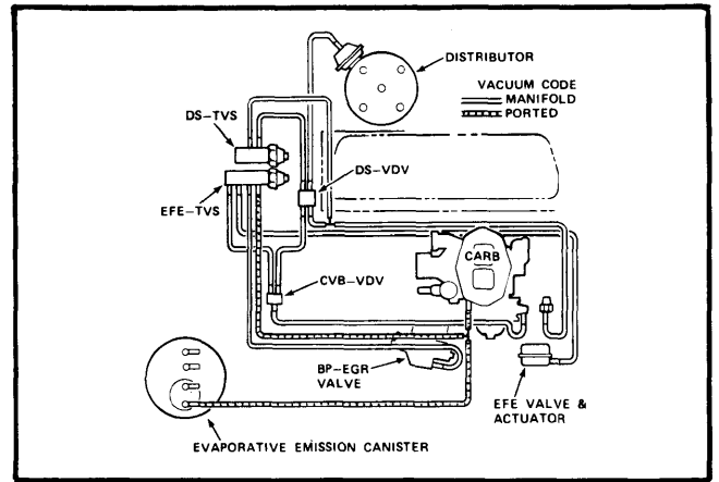
Fig. 2 151 CID Vacuum Hose Routing (Calif. with Auto. Trans., non-A/C)
