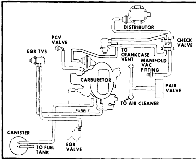
Fig. 3 Vega & Monza 140 CID Vacuum Hose Routing (Federal)
