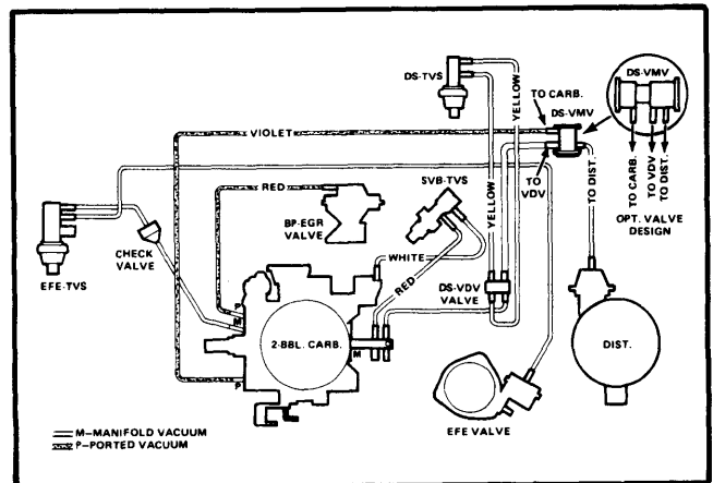
Fig. 12 301 CID Vacuum Hose Routing (Federal Auto. Trans. with A/C)
