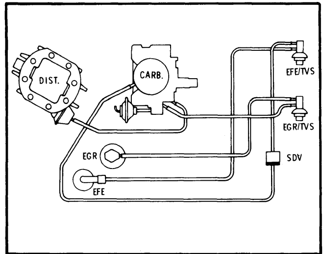
Fig. 8 Omega 305 CID Vacuum Hose Routing (Federal)
