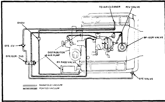
Fig. 7 231 CID Vacuum Hose Routing (High Alt.)
