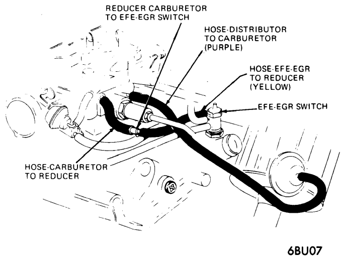
VACUUM HOSE ROUTING 350" 4-BBL. V8 WITHOUT AIR CONDITIONING
