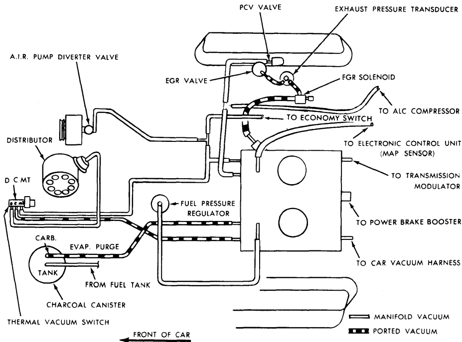
VACUUM HOSE ROUTING 500" V8 WITH FUEL INJECTION
