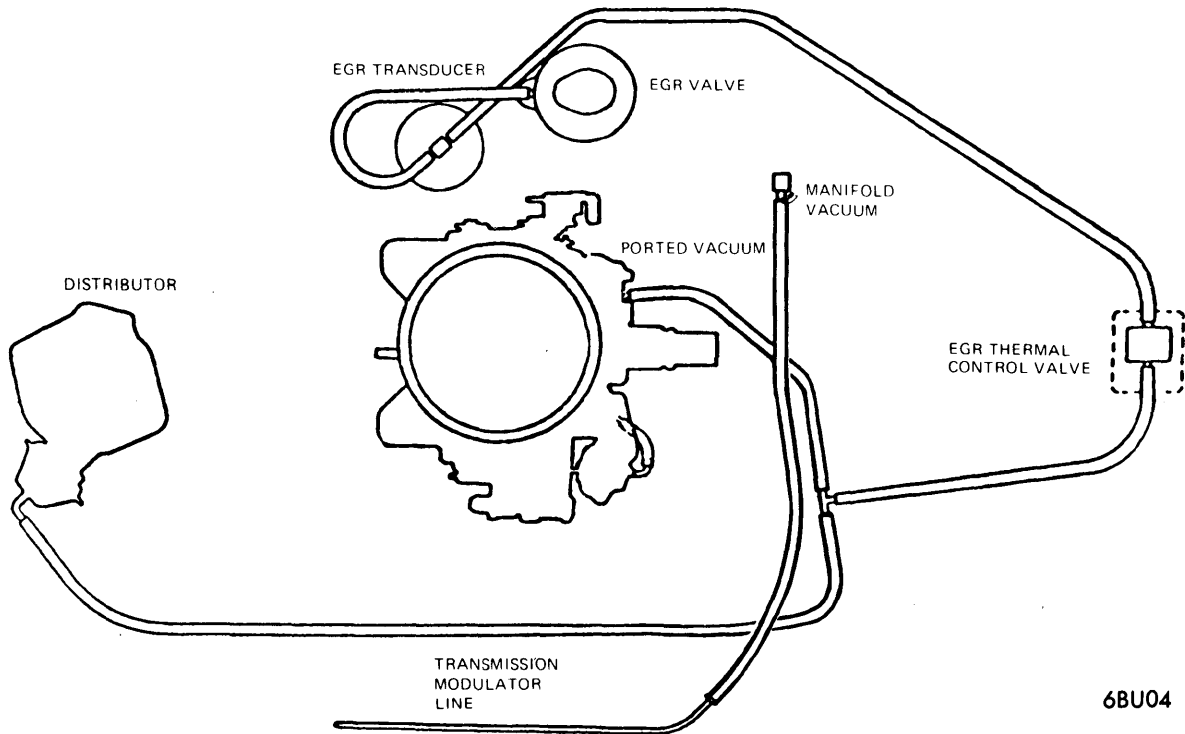
VACUUM HOSE ROUTING 260" V8 LATE PRODUCTION (CALIF.)
