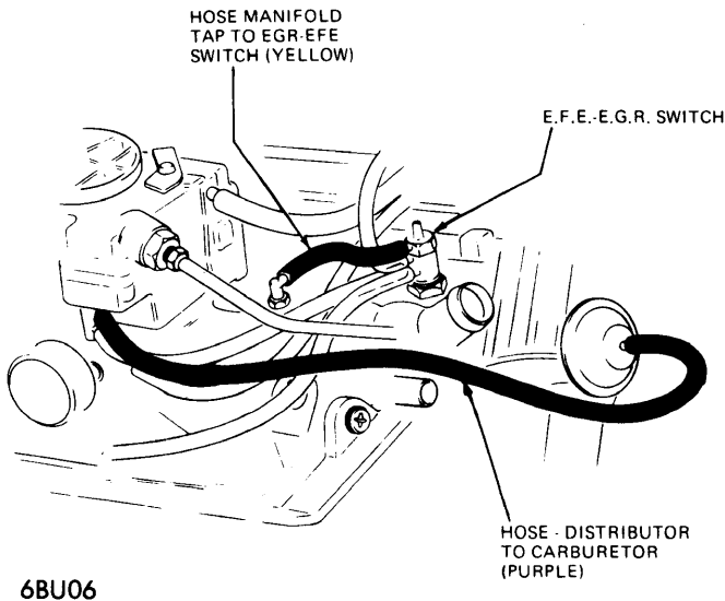
VACUUM HOSE ROUTING 350" 2-BBL. V8 WITHOUT AIR CONDITIONING
