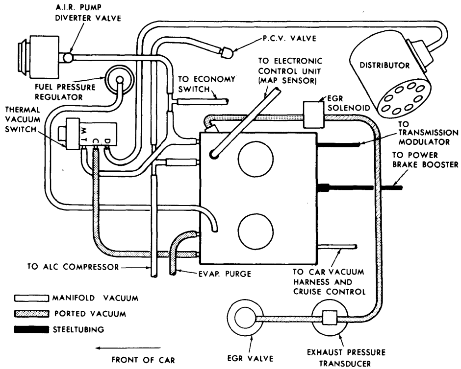
VACUUM HOSE ROUTING 350" V8 WITH FUEL INJECTION
