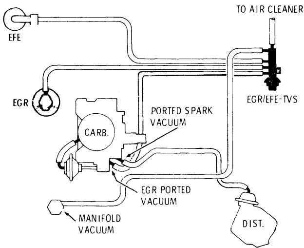
VACUUM HOSE ROUTING 231" V6
