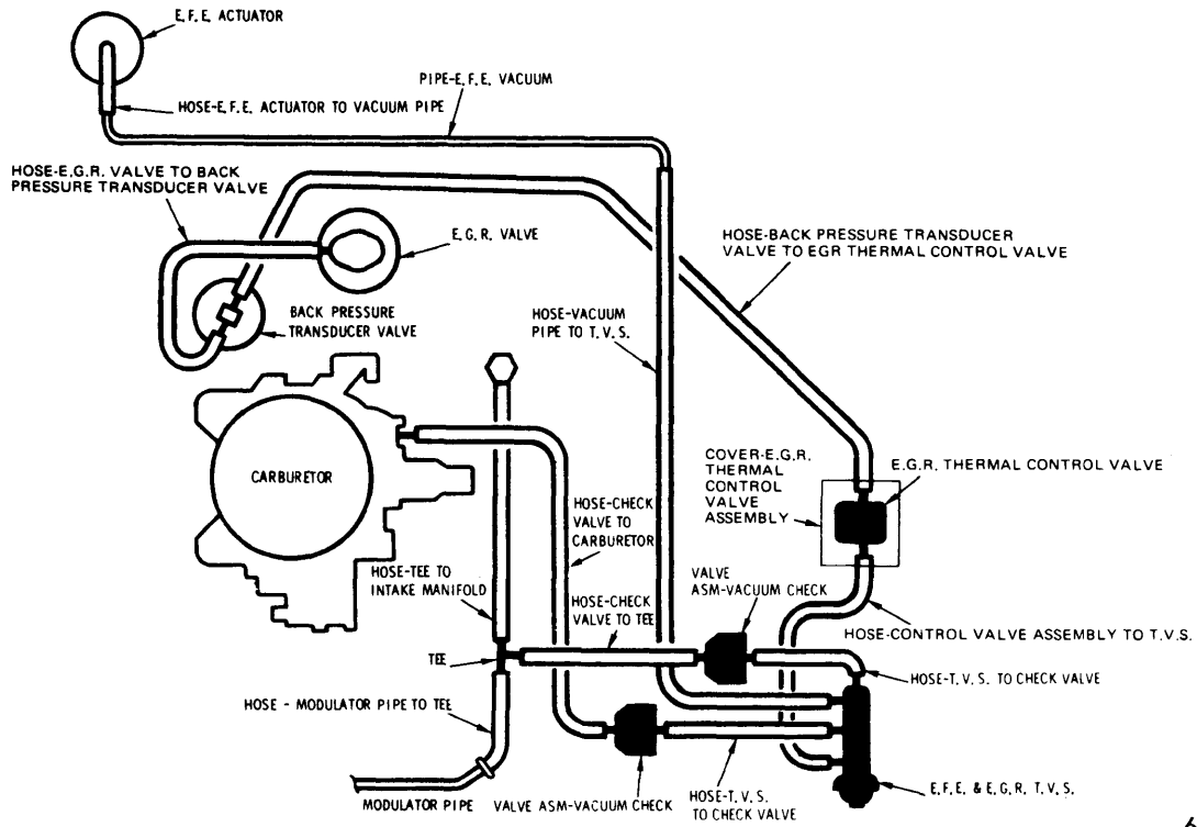
VACUUM HOSE ROUTING 260" V8 EARLY PRODUCTION (CALIF.)
