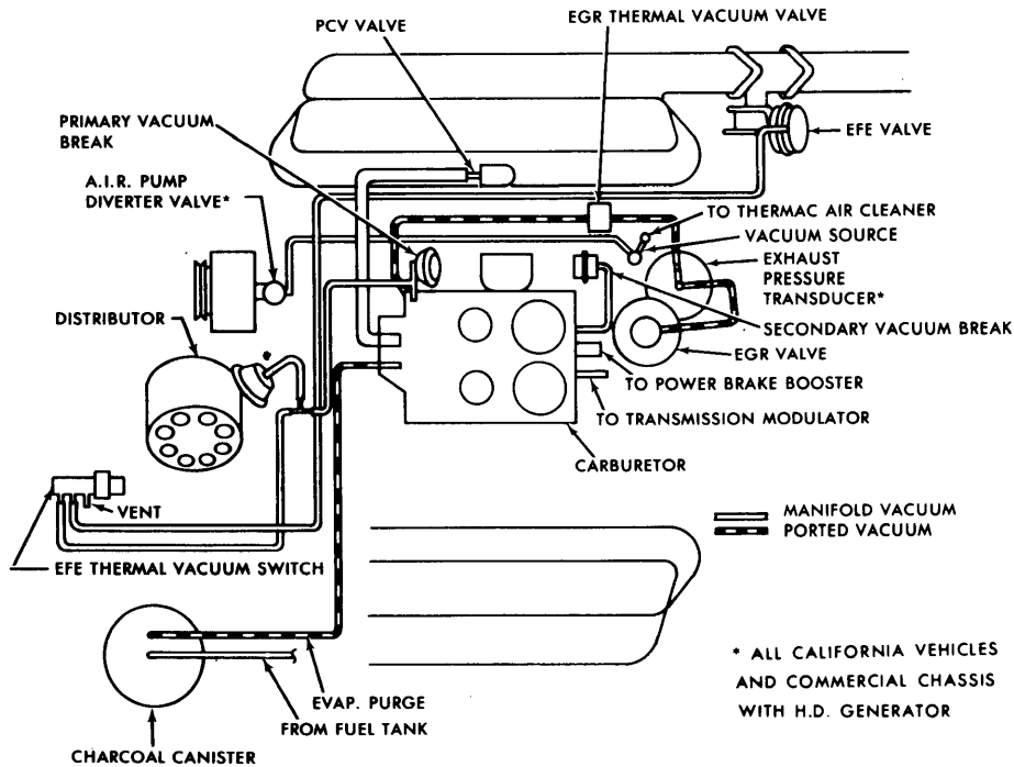
VACUUM HOSE ROUTING 500" V8 WITH CARBURETION
