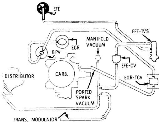
VACUUM HOSE ROUTING, OMEGA & CUTLASS 260" V8 2-Bbl. (FEDERAL-AUTO. TRANS.)
