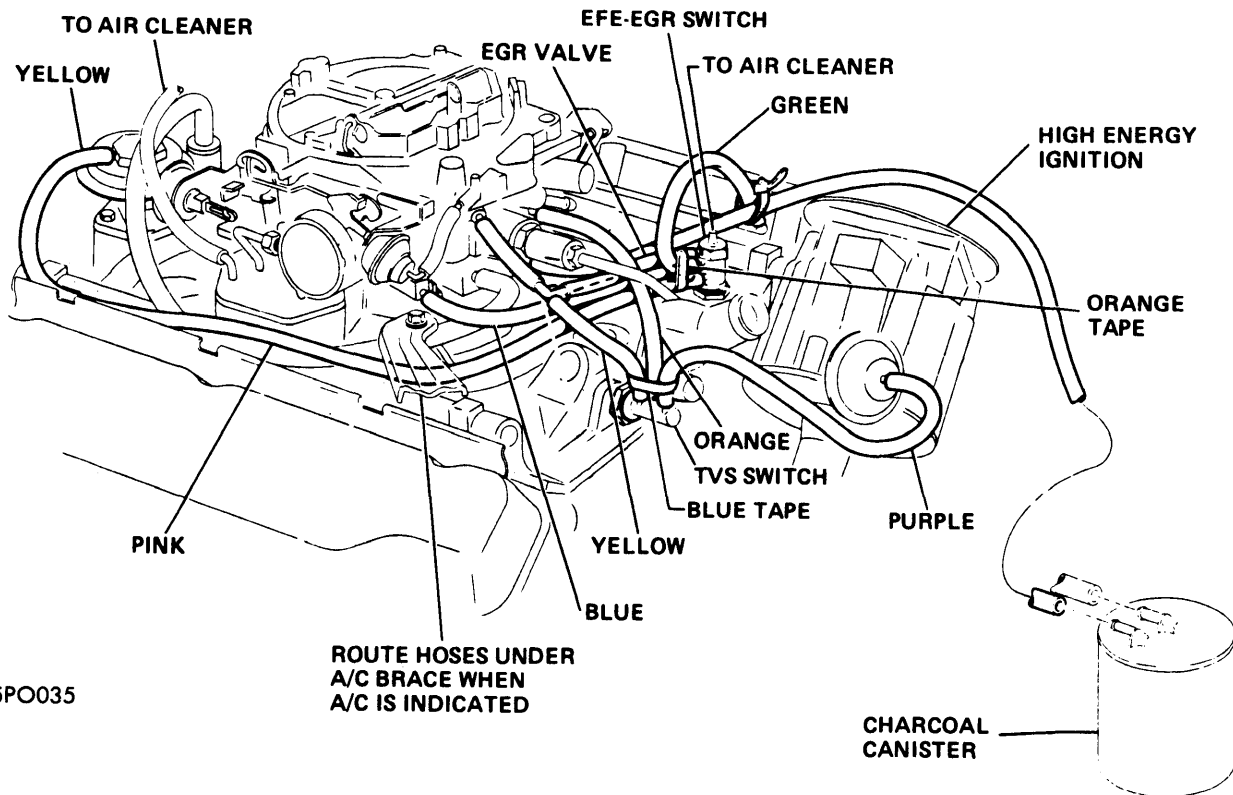
VACUUM HOSE ROUTING, 350" V8 4-Bbl. VENTURA (WITHOUT A.I.R.)
