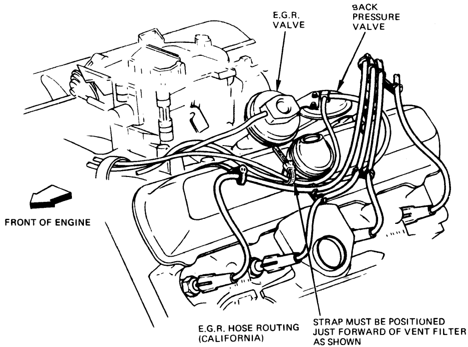
EGR VALVE STRAP, 260" V8
