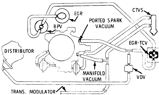
VACUUM HOSE ROUTING, CUTLASS & 88 350" V8 4-Bbl. (CALIF.)
