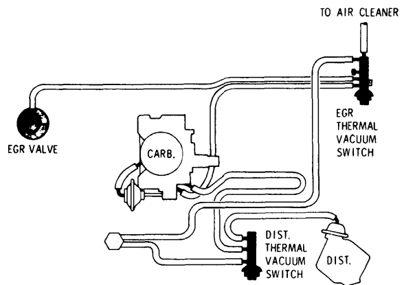
VACUUM HOSE ROUTING, OMEGA 350" V8 2-Bbl. (FEDERAL)
