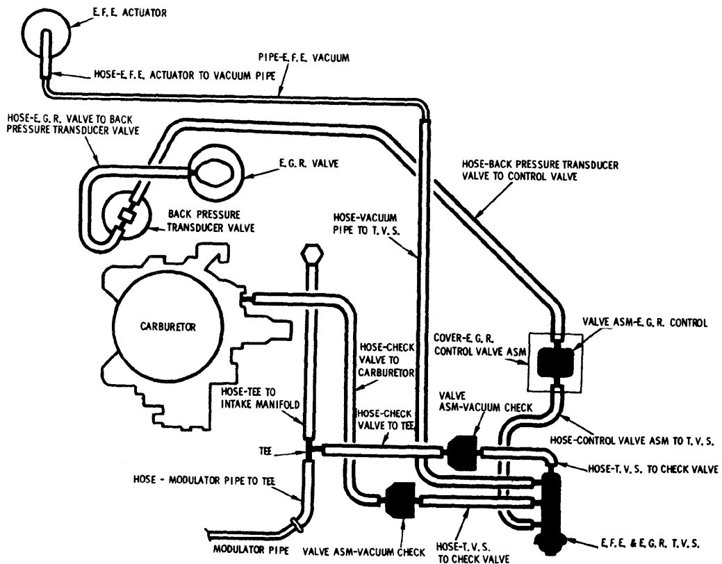
VACUUM HOSE ROUTING, 260" V8 (CALIF.)
