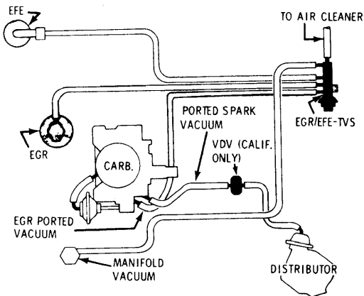
VACUUM HOSE ROUTING, STARFIRE 231" V6 2-Bbl.
