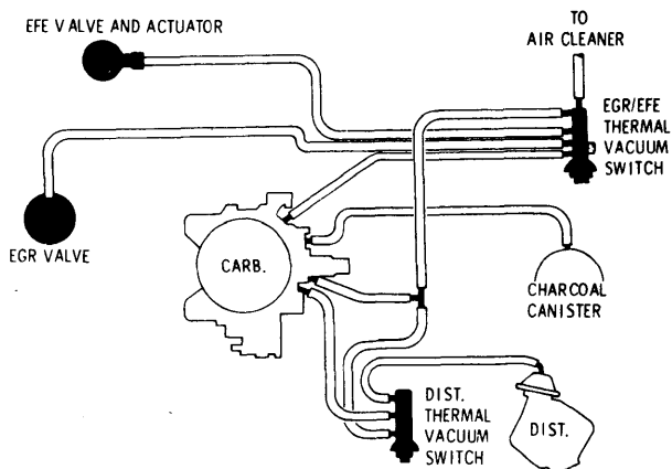
VACUUM HOSE ROUTING, OMEGA 350" V8 4-Bbl. (FEDERAL)
