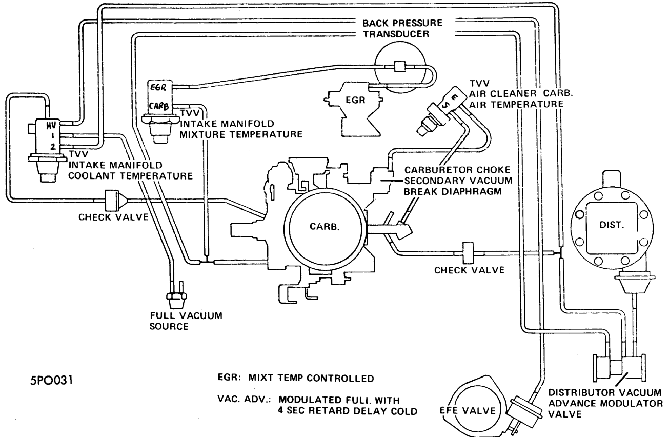
VACUUM HOSE ROUTING, 455" V8 4-Bbl. (FEDERAL)
