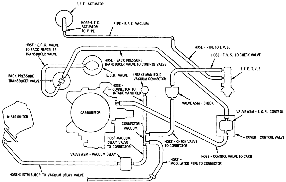
VACUUM HOSE ROUTING, 260" V8 (FEDERAL)
