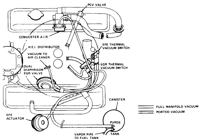
VACUUM HOSE ROUTING, 350" V8 (MONZA TOWN COUPE SHOWN)
