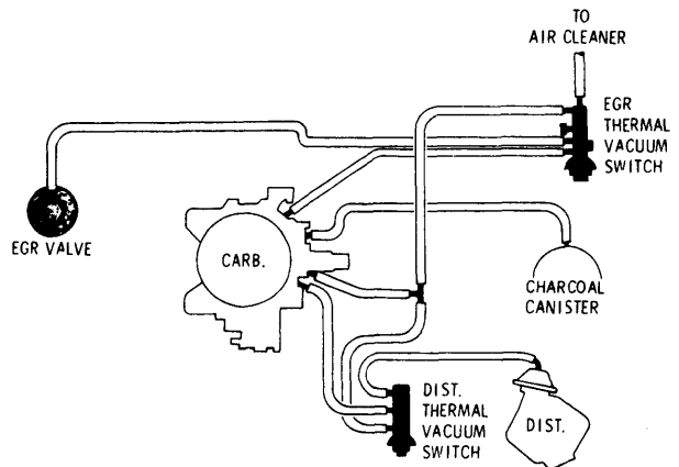
VACUUM HOSE ROUTING, OMEGA 350" V8 4-Bbl. (CALIF.)
