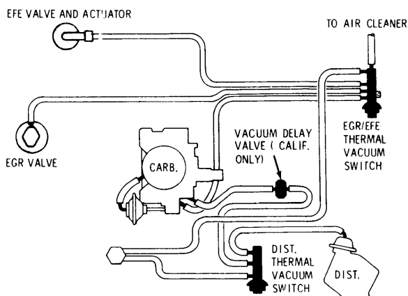
VACUUM HOSE ROUTING, STARFIRE 231" V6 2-Bbl. (ALL EARLY PRODUCTION)
