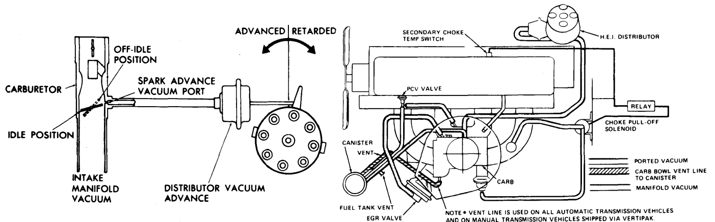
PORTED VACUUM ADVANCE (TYPICAL CHEVROLET SHOWN)
