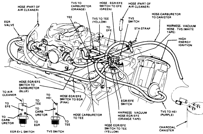
VACUUM HOSE ROUTING, 455" V8
