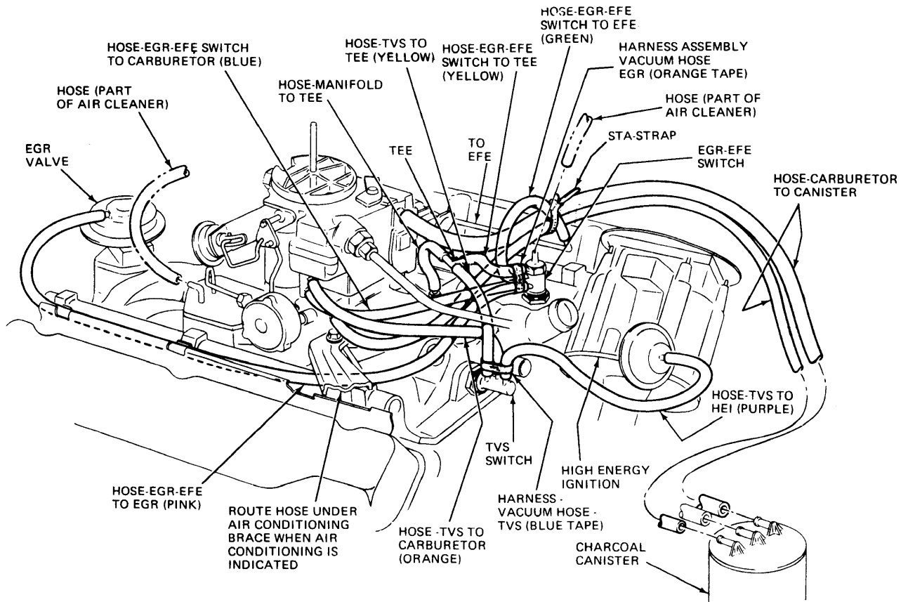
VACUUM HOSE ROUTING, 350" V8 (2-Bl.)
