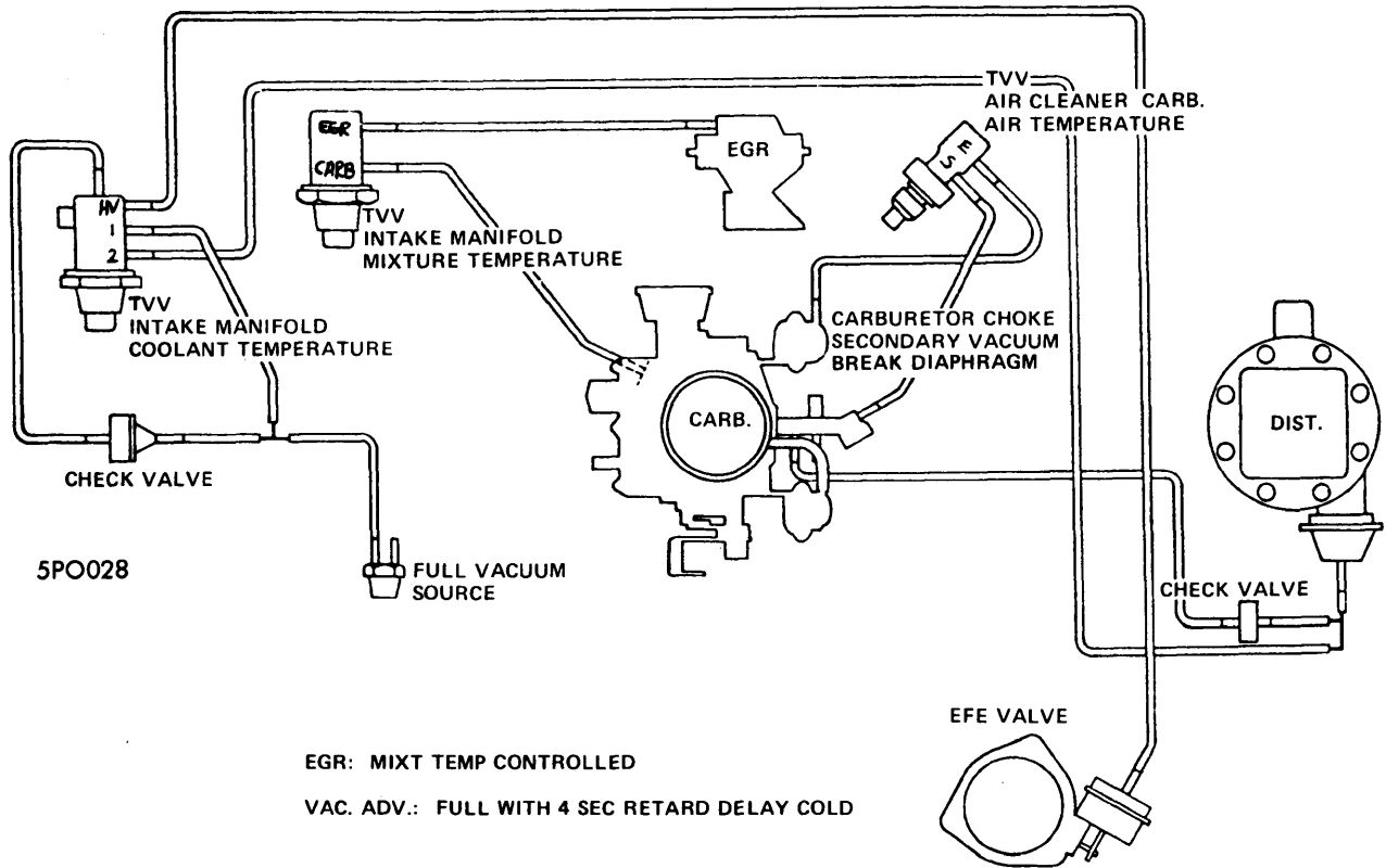
VACUUM HOSE ROUTING, 400" V8 2-Bbl. (FEDERAL)
