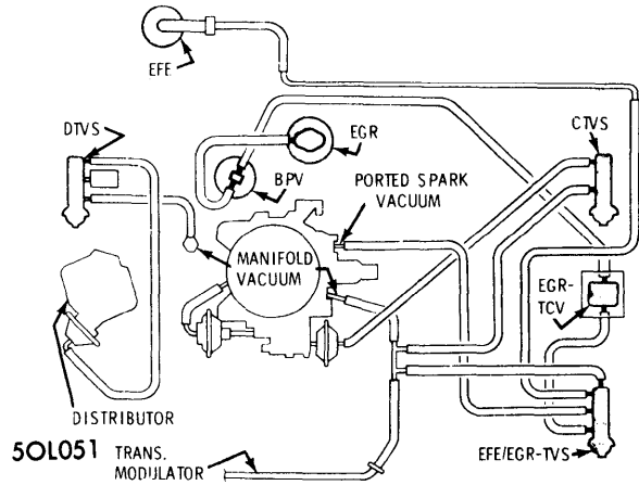
VACUUM HOSE ROUTING, TORONADO 455" V8 4-Bbl. (CALIF.)
