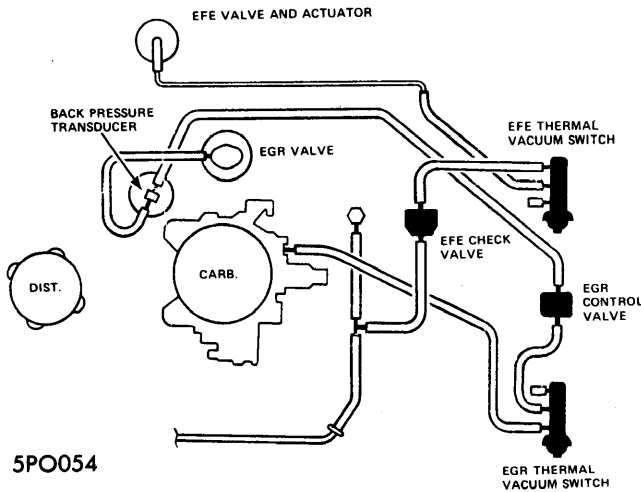
VACUUM HOSE ROUTING, 260" V8 VENTURA (AUTO. TRANS.-CALIF.)
