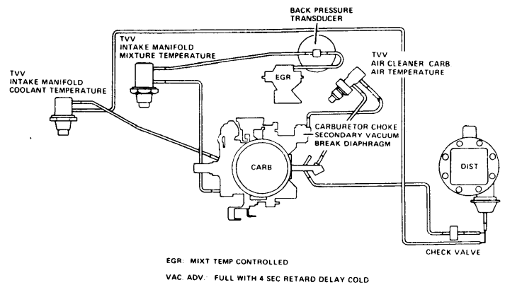
VACUUM HOSE ROUTING, 400" V8 (CALIF.)
