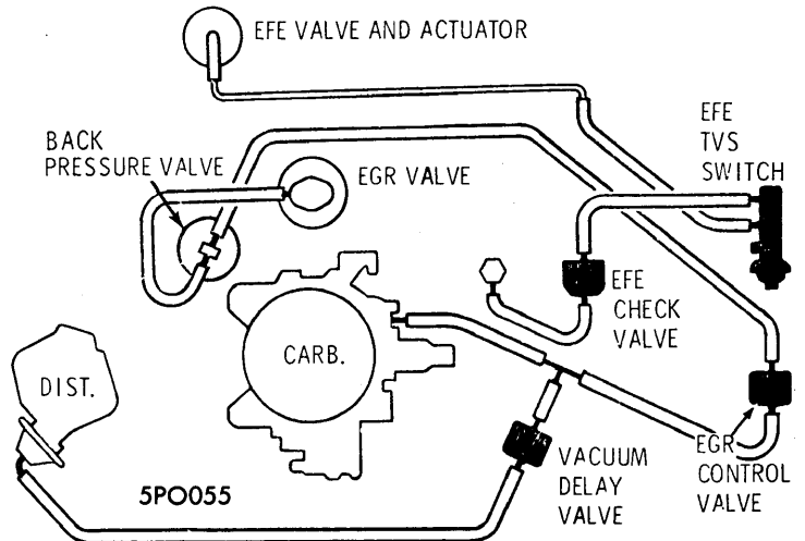
VACUUM HOSE ROUTING, 260" V8 VENTURA (MAN. TRANS.-FEDERAL)
