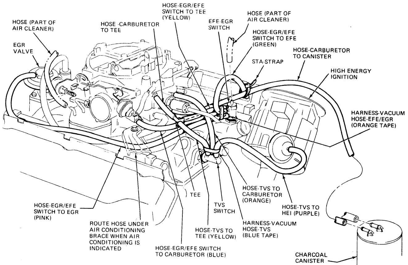
VACUUM HOSE ROUTING, 350" V8 W/4-Bbl. (WITHOUT A.I.R.)
