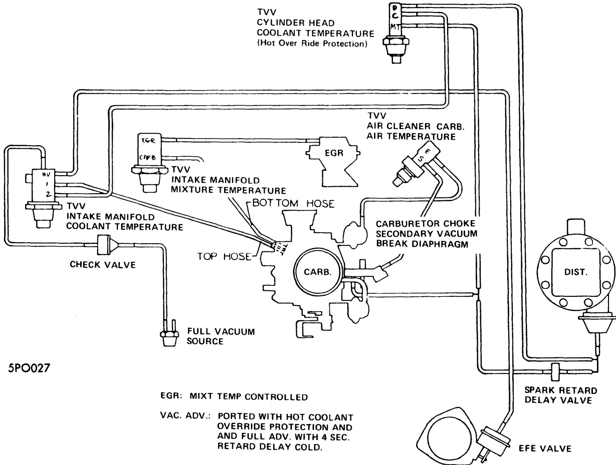
VACUUM HOSE ROUTING, 350" V8 2-Bbl., EXC. VENTURA (FEDERAL)
