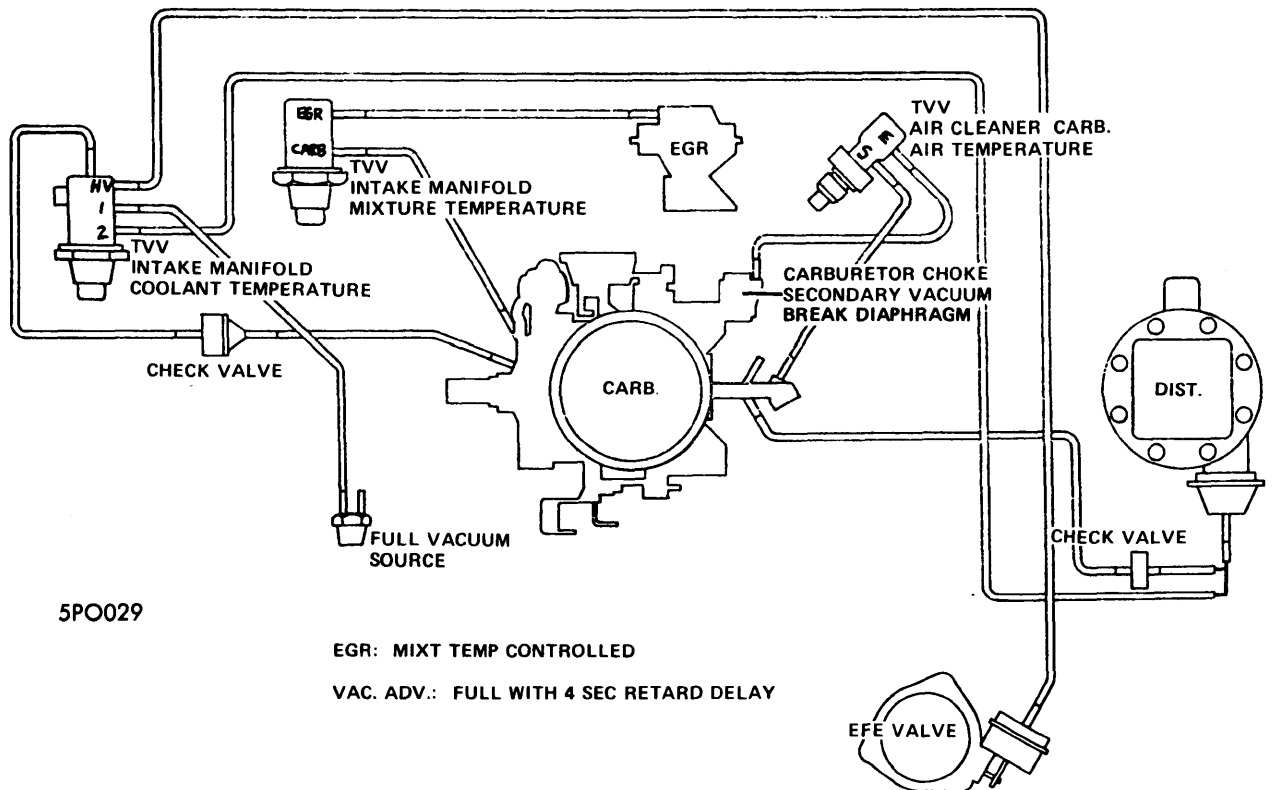
VACUUM HOSE ROUTING, 350"/400" V8 4-Bbl., EXC. VENTURA (FEDERAL-AUTO. TRANS.)
