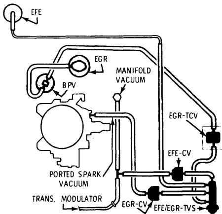
VACUUM HOSE ROUTING, OMEGA & CUTLASS 260" V8 2-Bbl. (CALIF.-AUTO. TRANS.)
