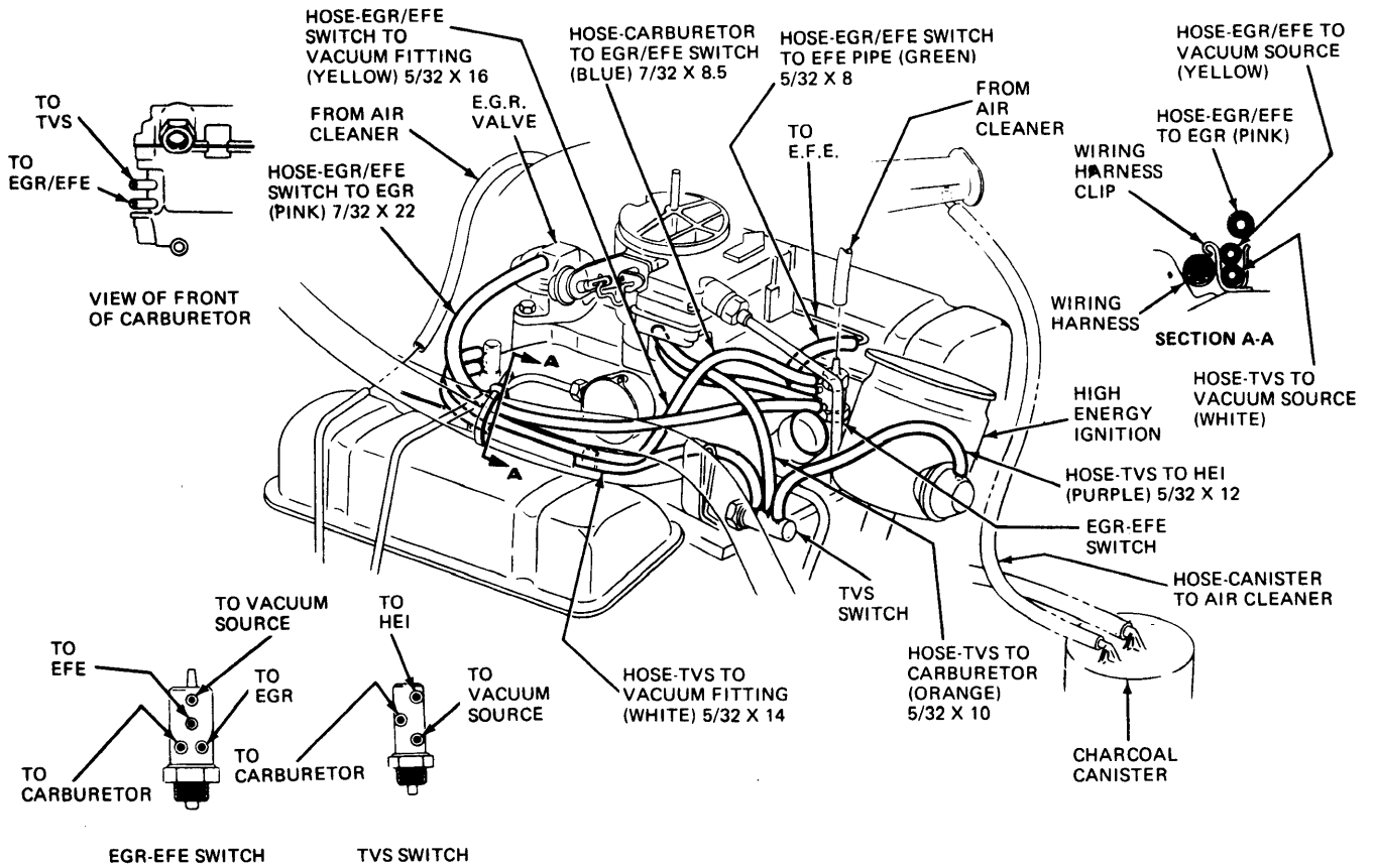
VACUUM HOSE ROUTING, 231" V6 (FEDERAL)
