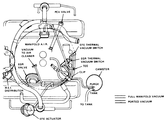
VACUUM HOSE ROUTING 260" V8 (MONZA TOWN COUPE SHOWN)
