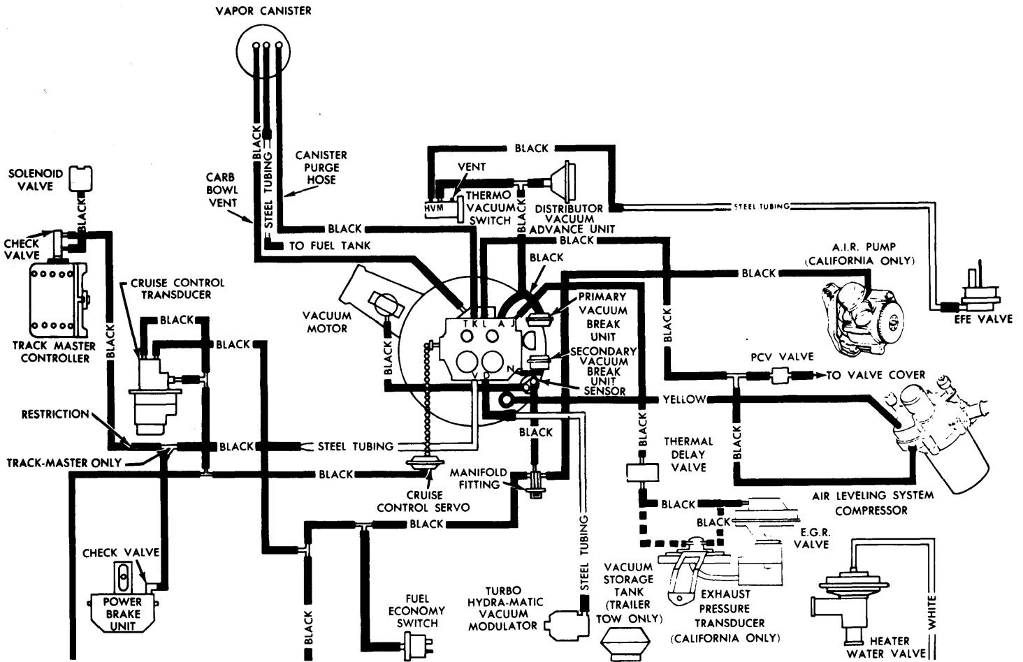
CADILLAC EMISSION CONTROL SYSTEMS
