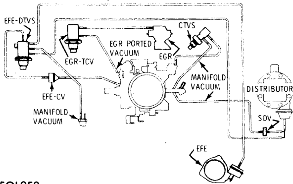
VACUUM HOSE ROUTING, ALL 88 STATION WAGON & 98 400" V8 4-Bbl. (FEDERAL)
