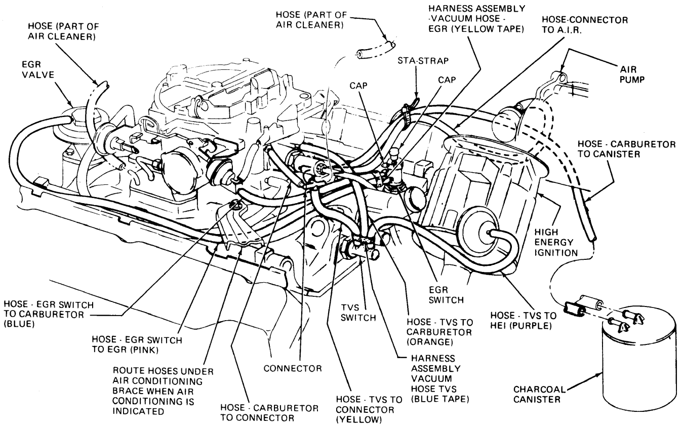
VACUUM HOSE ROUTING, 350" V8 W/4-Bbl. & A.I.R. (WITHOUT EFE)
