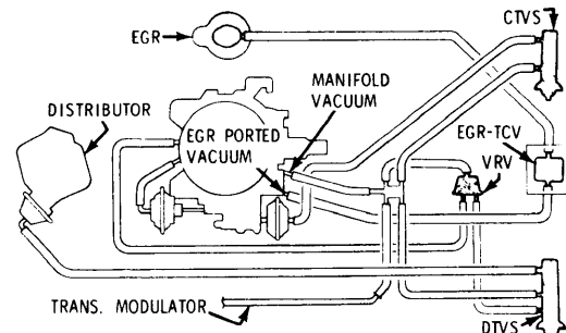
VACUUM HOSE ROUTING, CUTLASS, 88 & 98 455" V8 4-Bbl. (FEDERAL)
