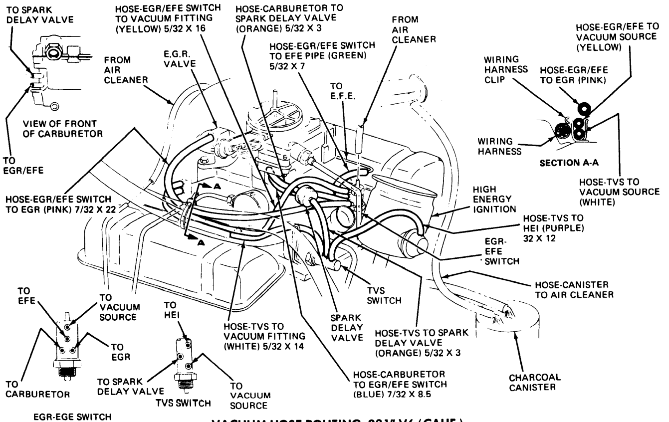
VACUUM HOSE ROUTING, 231" V6 (CALIF.)
