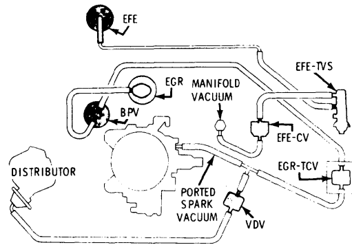
VACUUM HOSE ROUTING, OMEGA & CUTLASS 260" V8 2-Bbl. (FEDERAL-MAN. TRANS.)
