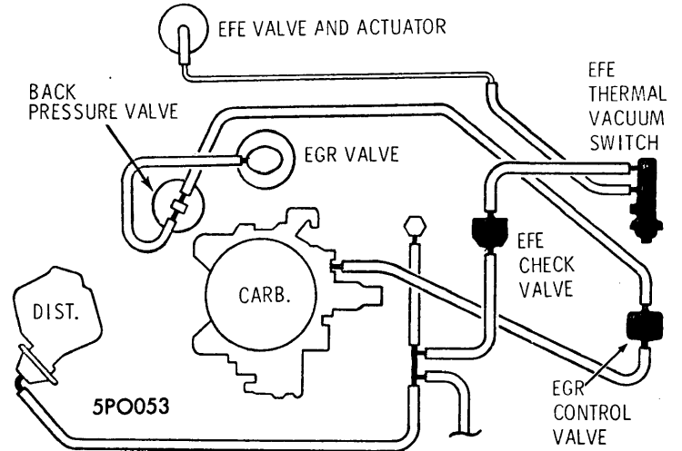
VACUUM HOSE ROUTING, 260" V8 VENTURA (AUTO. TRANS.-FEDERAL)
