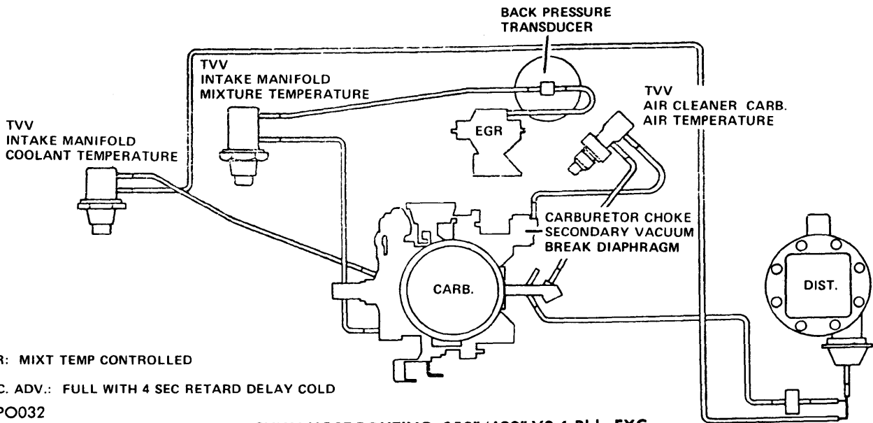
VACUUM HOSE ROUTING, 350"/400" V8 4-Bbl., EXC. VENTURA (CALIF.)
