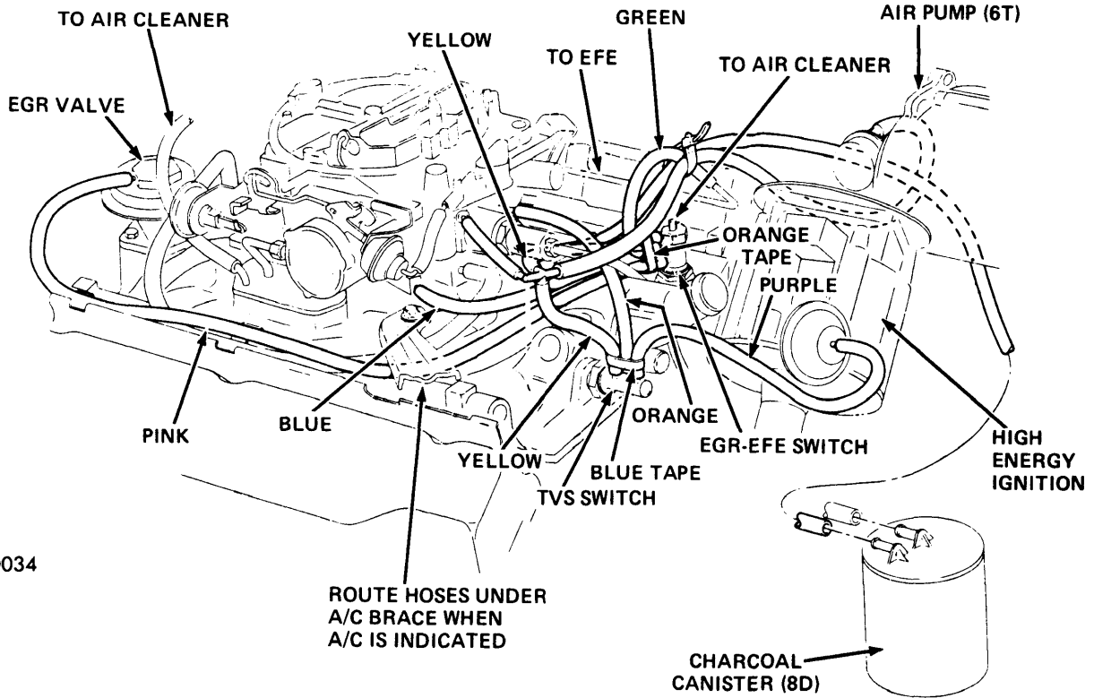
VACUUM HOSE ROUTING, 350" V8 4-Bbl. VENTURA (WITH A.I.R.)
