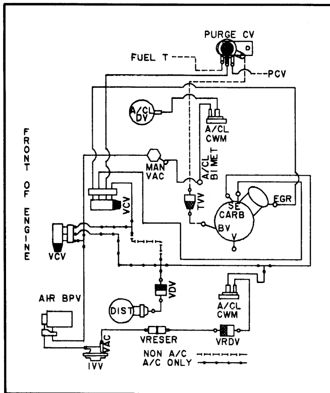
Fig. 39 Calibration 9-6A-R10; 200"; Federal
