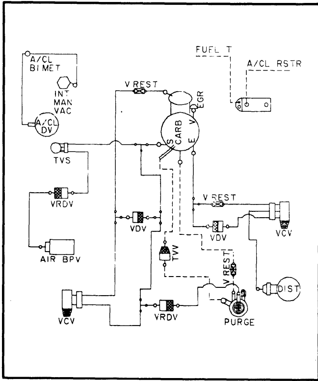
Fig. 85 Calibration 9-14E-R15; 351" M; Federal
