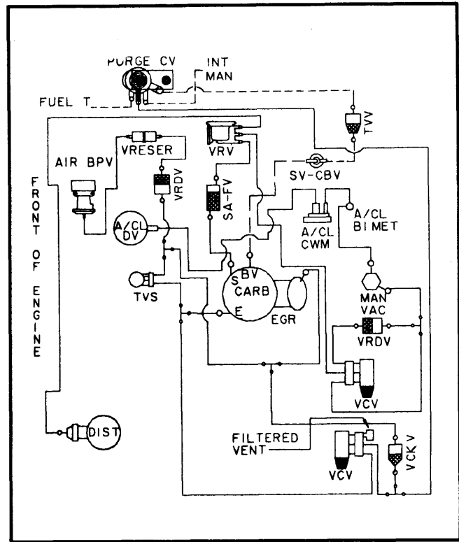
Fig. 58 Calibration 9-11A-R20; 302"; Federal
