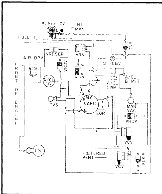
Fig. 79 Calibration 9-11X-R10; 302"; Federal
