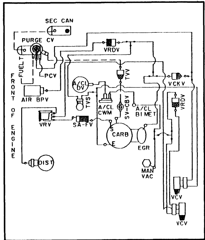
Fig. 68 Calibration 9-11J-R10 and 9-11J-R13 302"; Federal
