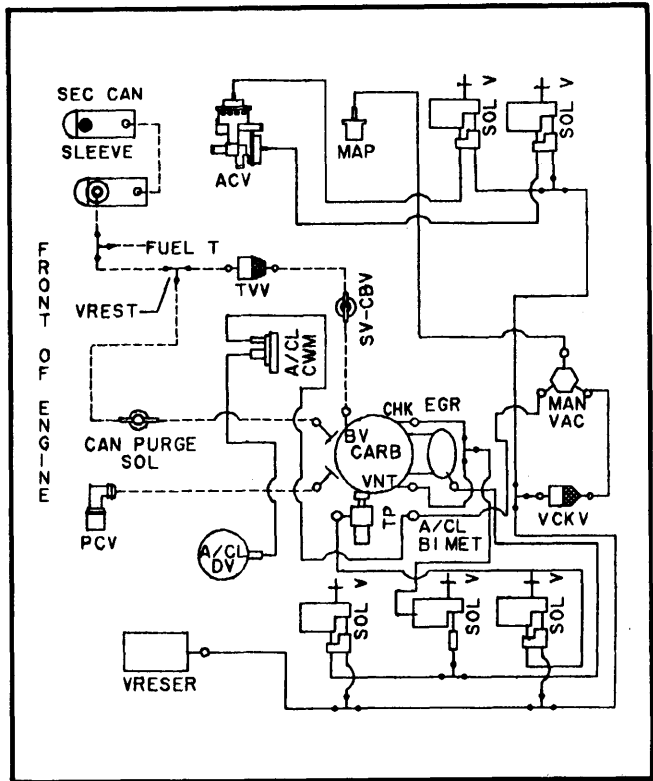
Fig. 90 Calibration 9-12A-R0; 351" W; Federal
