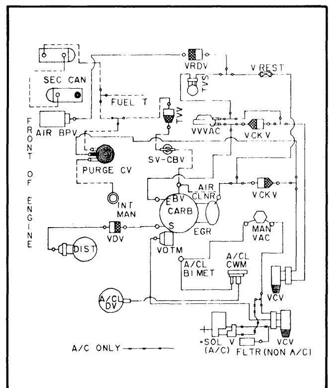
Fig. 64 Calibration 9-11E-R1; 302"; Calif.
