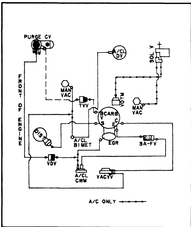
Fig. 31 Calibration 9-21B-R0; 2.3L; Federal
