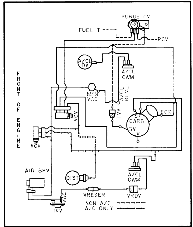
Fig. 38 Calibration 9-6A-R0; 200"; Federal
