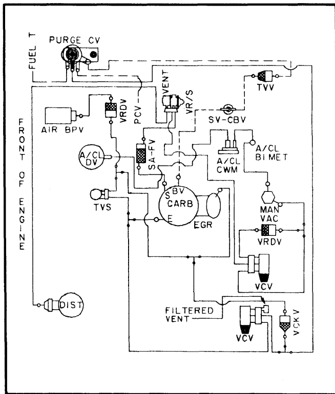
Fig. 59 Calibration 9-11B-R0; 302"; Federal
