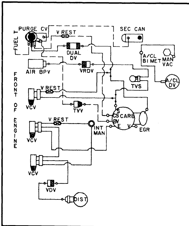
Fig. 87 Calibration 9-14Q-R0; 351" M; Federal
