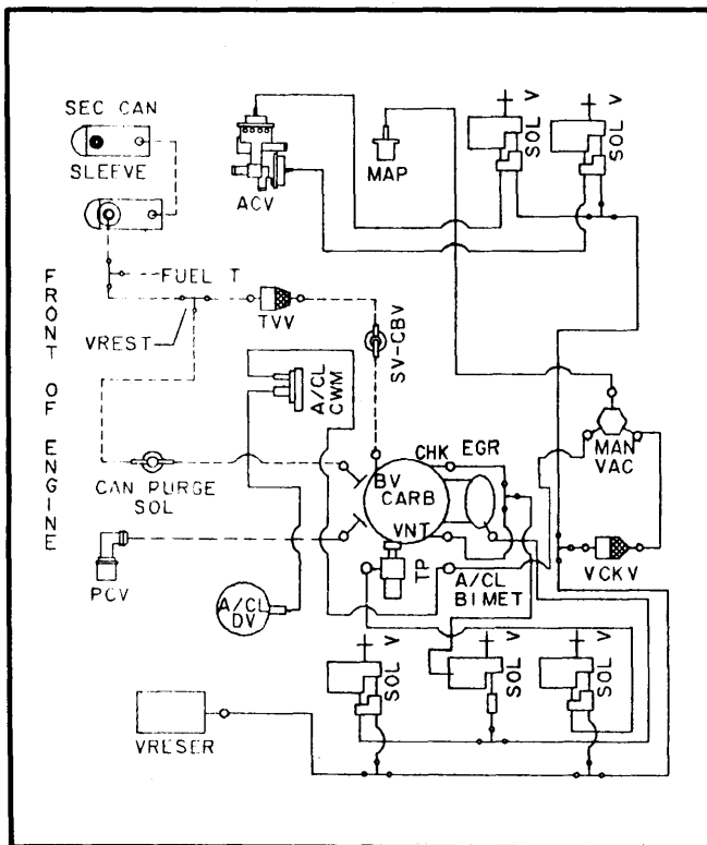
Fig. 91 Calibration 9-12B-R0; 351" W; Federal
