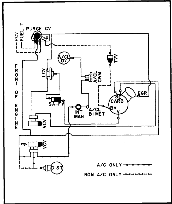
Fig. 42 Calibration 9-7A-R11, 9-7A-R12 and 9-7A-R13; 200"; Federal
