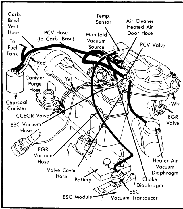
Fig. 1 1.7 Liter; Federal
