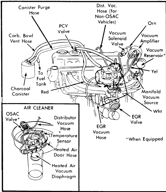
Fig. 5 225" 2-Barrel; Federal (Exc. Wagon) 3500#; Auto. Trans.
