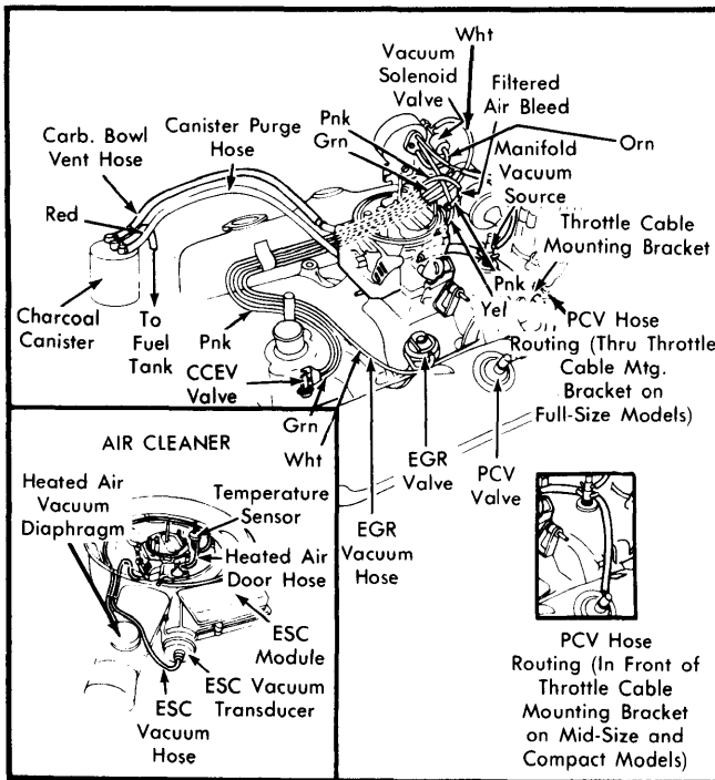
Fig. 9 360" 2-Barrel; Federal; Auto. Trans.
