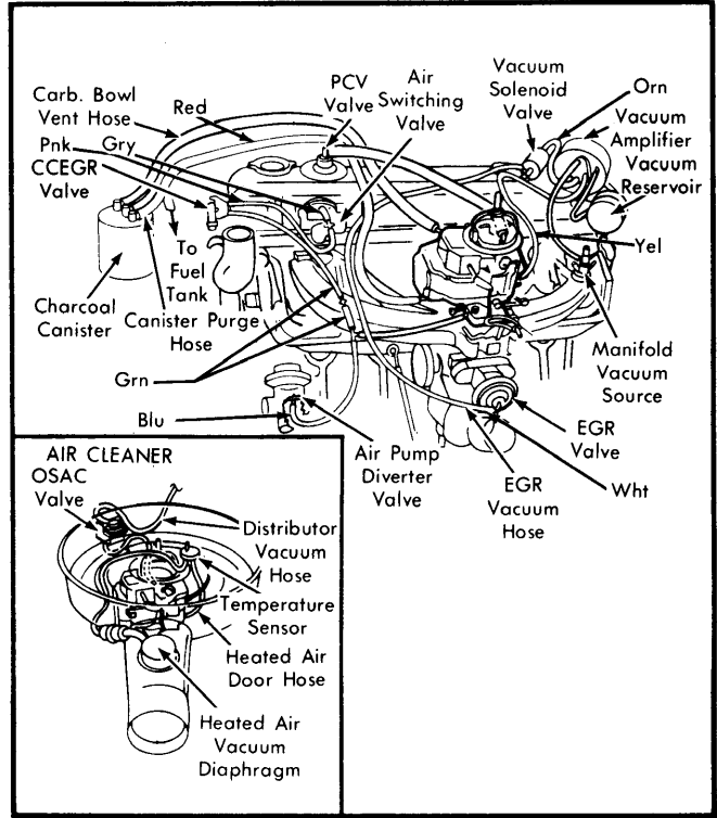
Fig. 6 225" 2-Barrel; Federal; 4000#; Auto. Trans.
