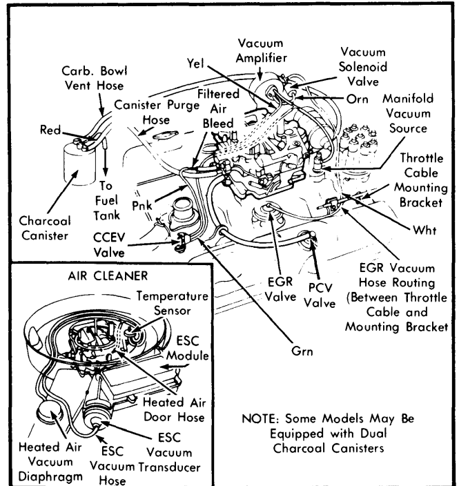
Fig. 10 360" 4-Barrel; Federal; Auto. Trans.
