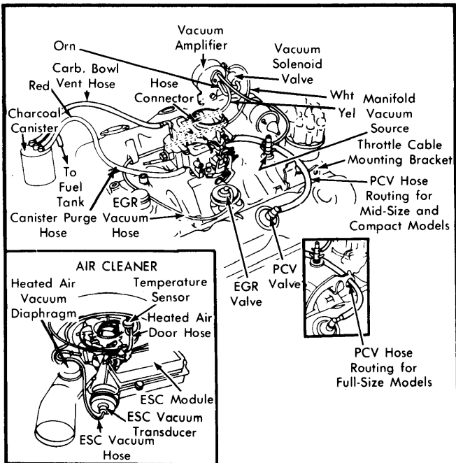
Fig. 7 318" 2-Barrel; Federal; Auto. Trans.
