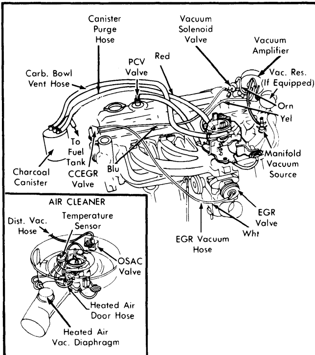
Fig. 3 225" 1-Barrel; Federal; All Trans.
