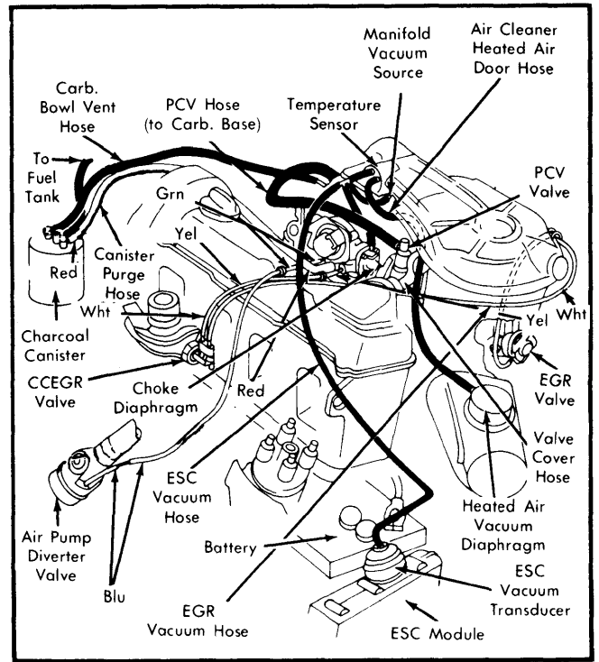
Fig. 2 1.7 Liter; California
