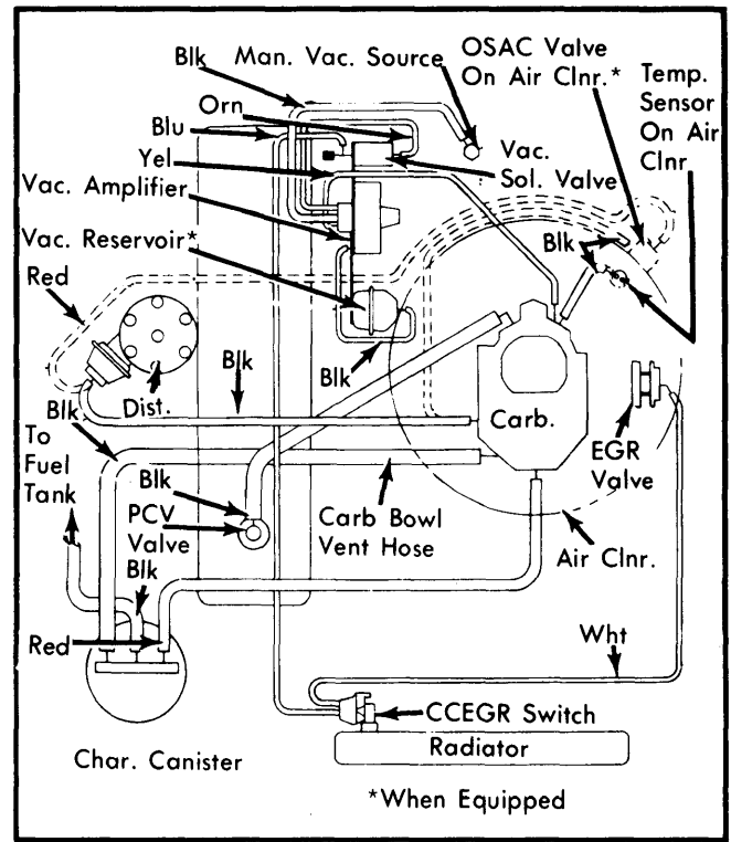
Fig. 6 225" 2-Bbl., Federal and Canada, Manual and Automatic Transmissions
