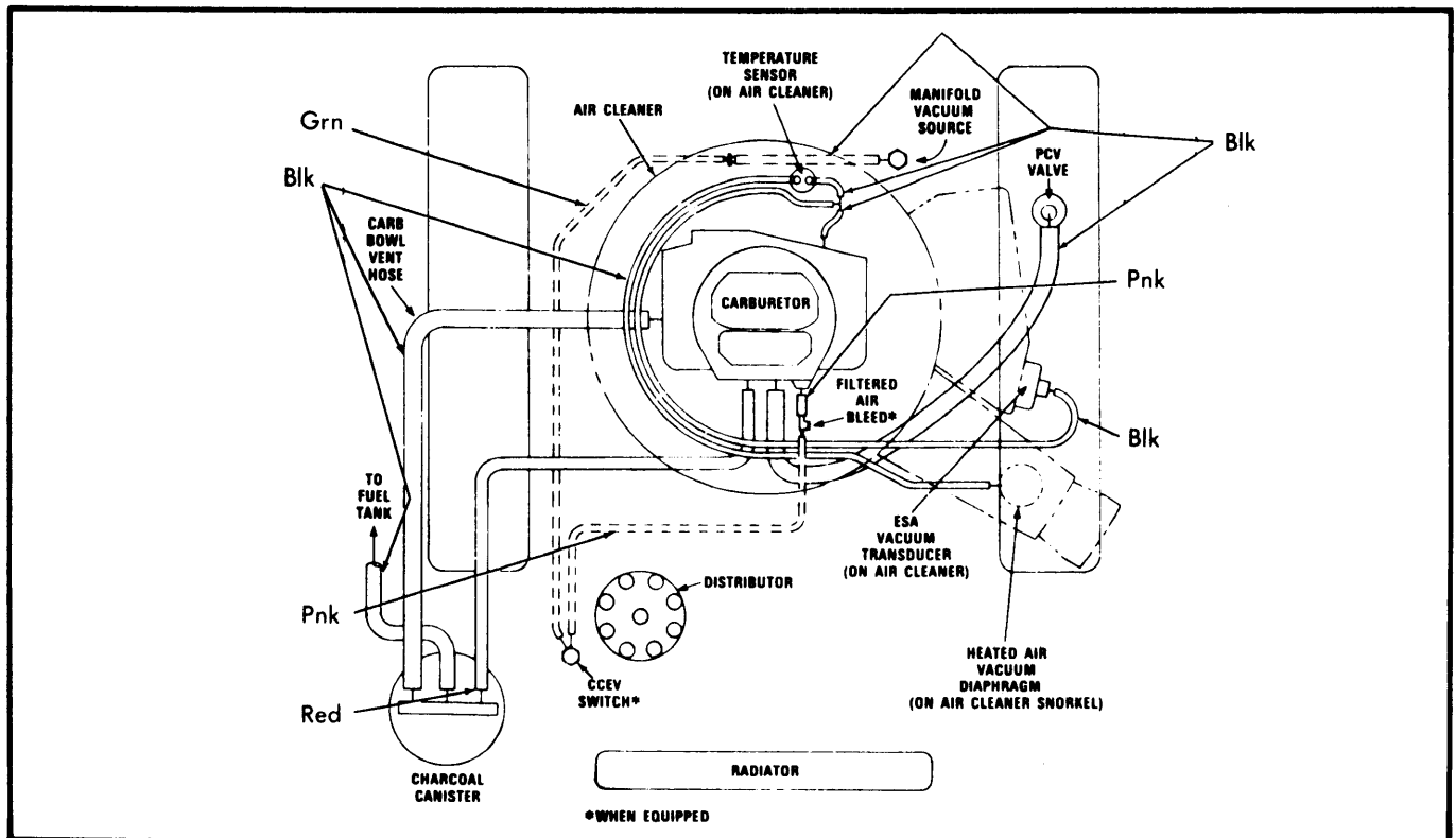
Fig. 16 400" and 440" 4-Bbl., Canada, with ELB, Auto. Trans.
