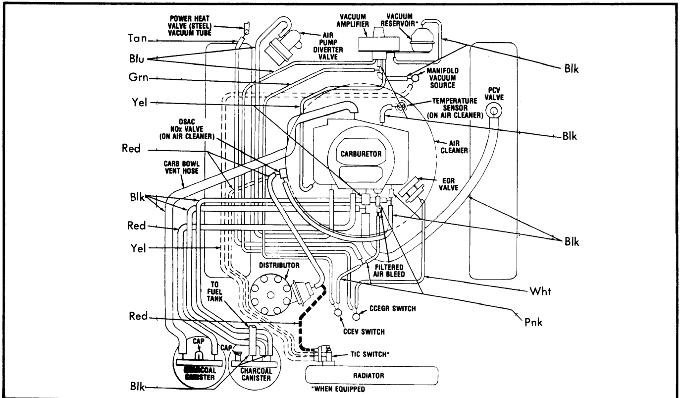
Fig. 20 440" 4-Bbl., Calif., with Catalyst and Air Pump, Auto. Trans.
