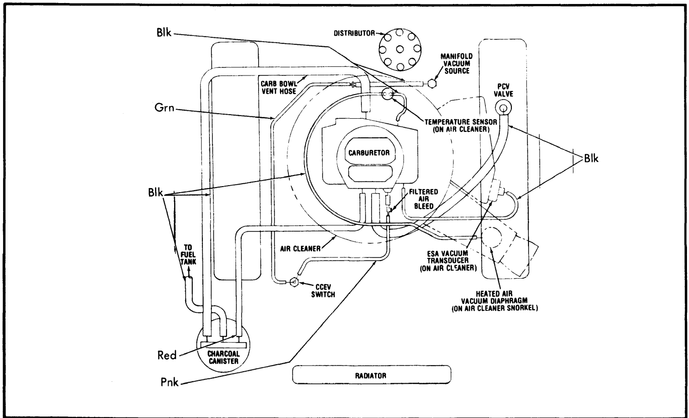
Fig. 11 360" 4-Bbl., Federal and Canada with ELB, Catalyst, Auto. Trans.
