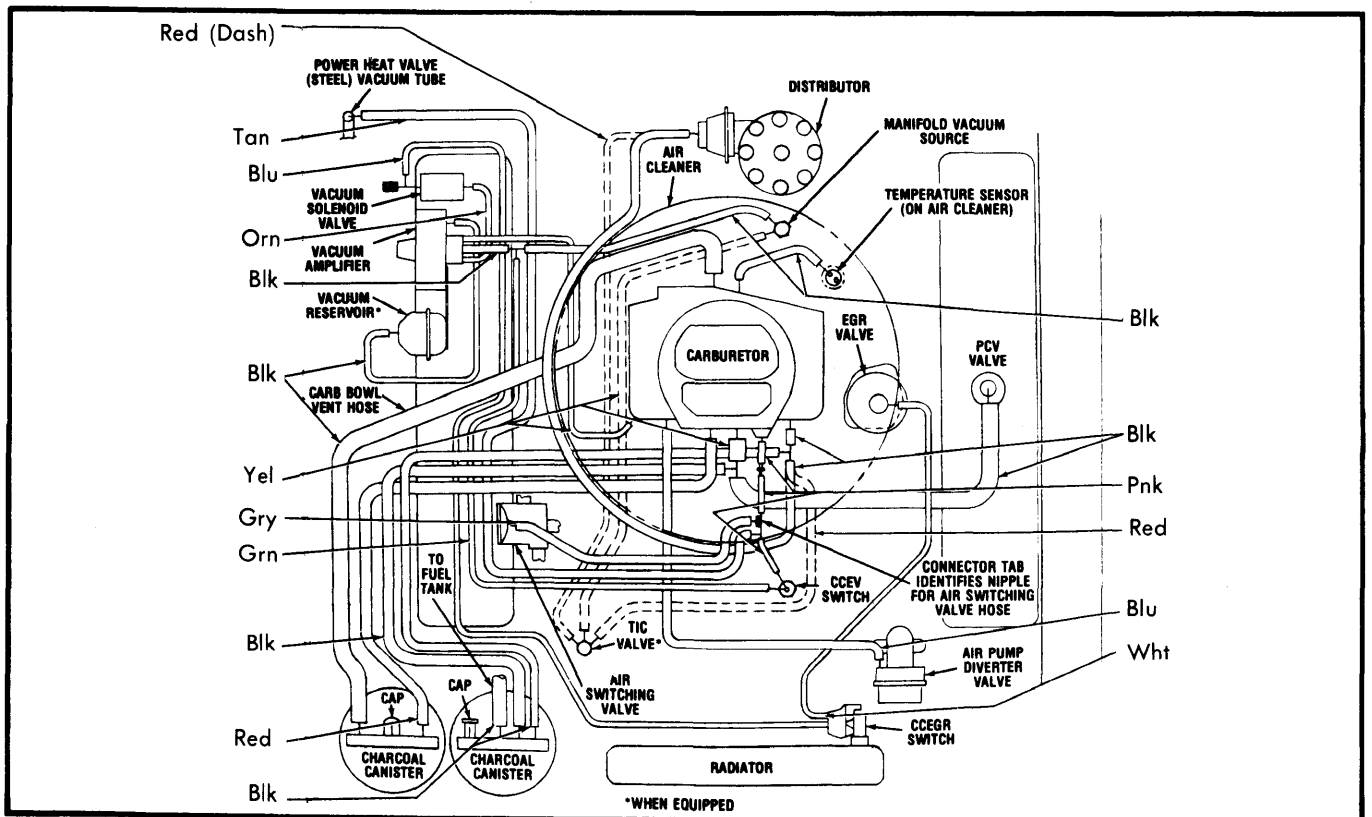
Fig. 12 360" 2-Bbl., Chrysler Only, High Altitude, Auto. Trans.
