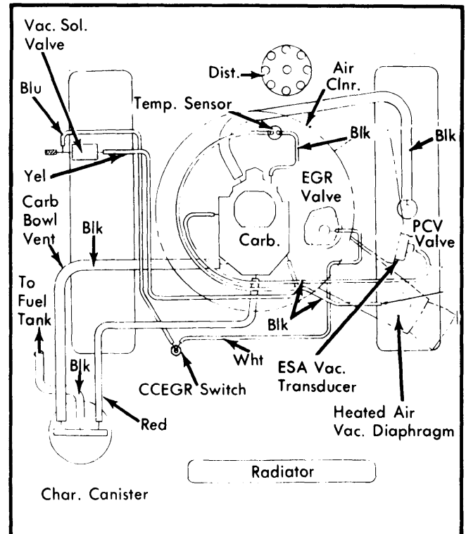
Fig. 8 318" 2-Bbl., Federal and Canada with ELB, All Trans.; High Alt., w/o ELB, Auto. Trans.
