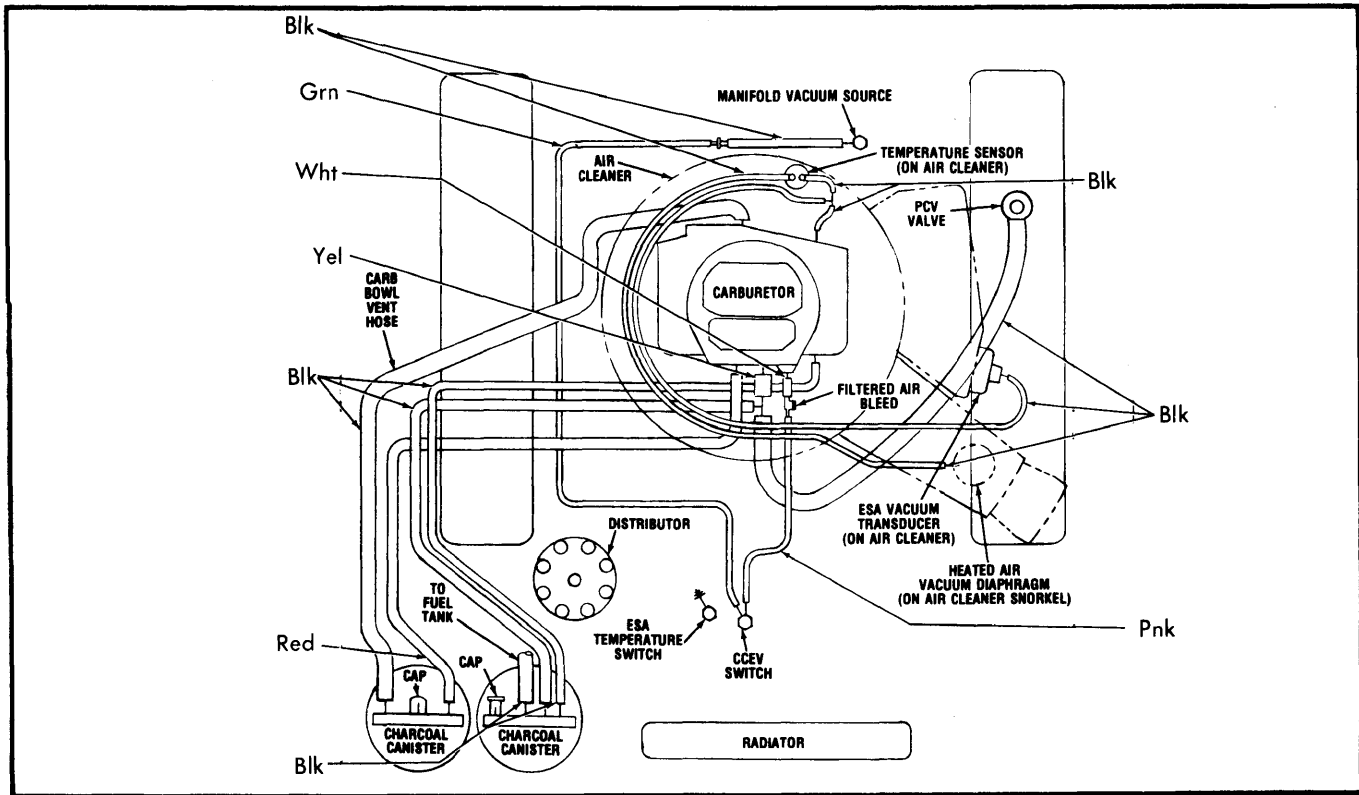
Fig. 17 400" 4-Bbl., Chrysler, Federal, with ELB and Catalyst, Auto. Trans.
