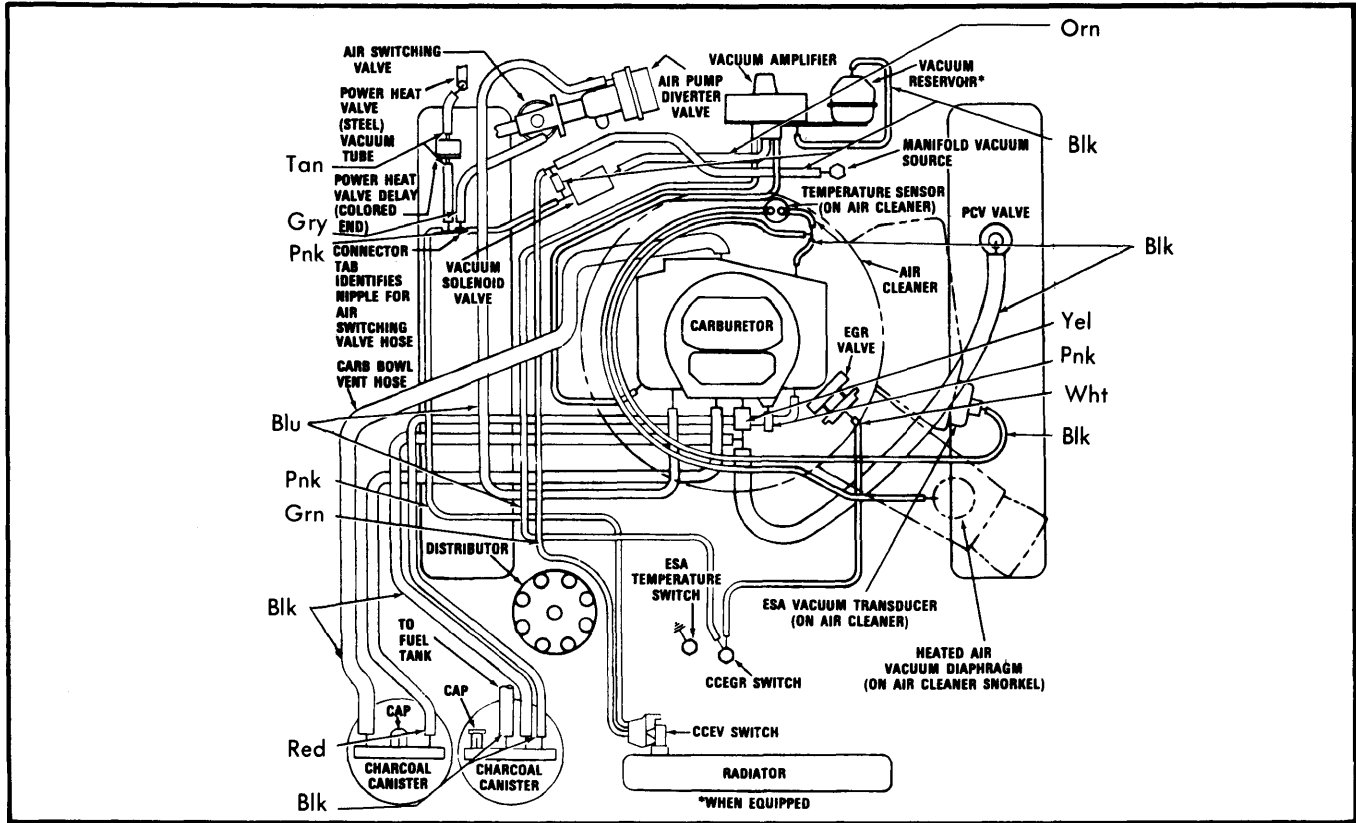
Fig. 21 440" 4-Bbl., Calif., with ELB, Catalyst and Air Pump, Auto. Trans.
