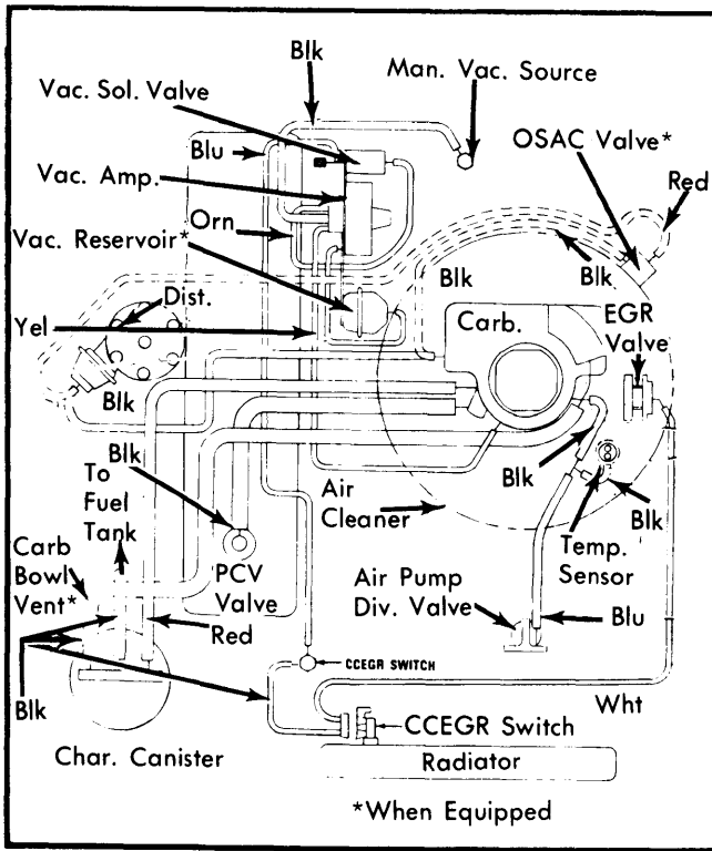
Fig. 5 225", Canada w/o Catalyst, Auto. Trans.
