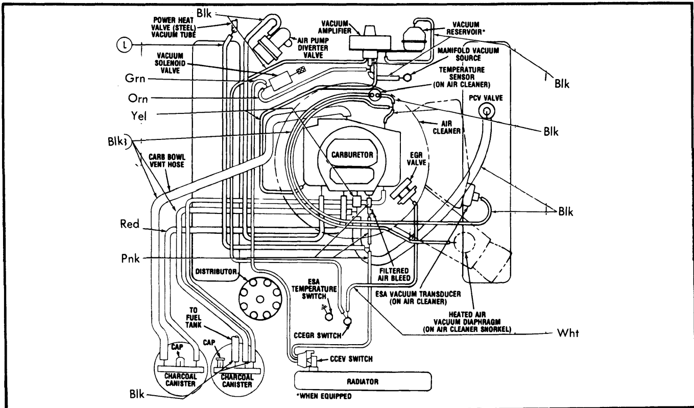
Fig. 18 440" 4-Bbl., Federal and Canada, with ELB and Catalyst, Auto. Trans.
