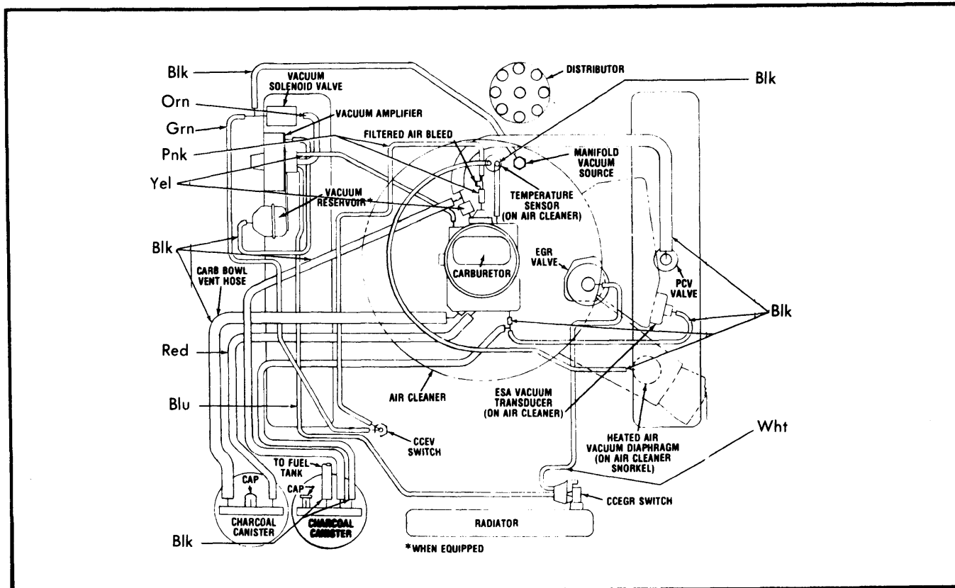
Fig. 14 360" 2-Bbl., Chrysler, Federal, with ELB and Catalyst, Auto. Trans.
