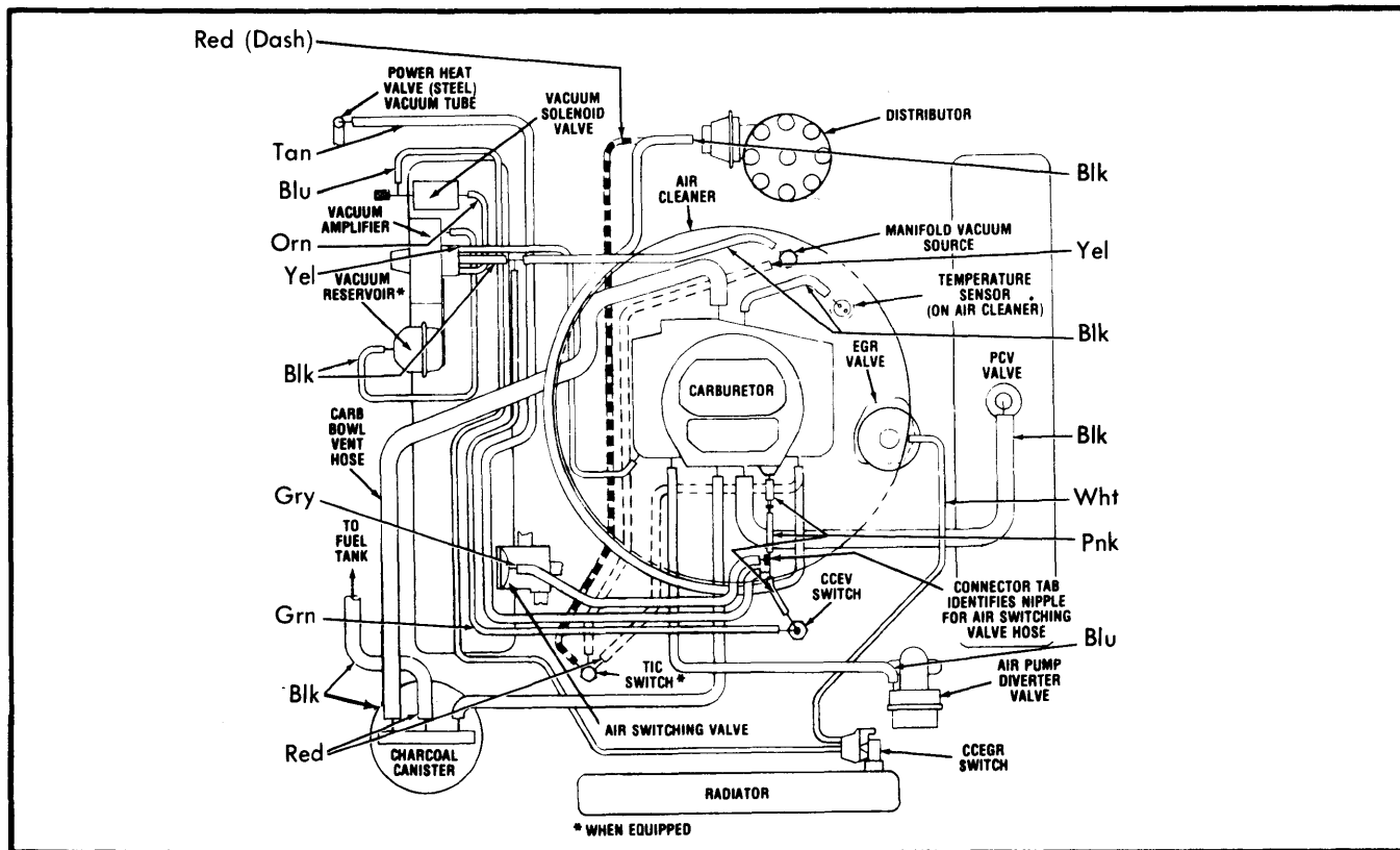
Fig. 13 360" 2-Bbl. and 4-Bbl., Exc Chrysler, High Altitude, and 360" 4-Bbl., Calirnia, Auto. Trans.
