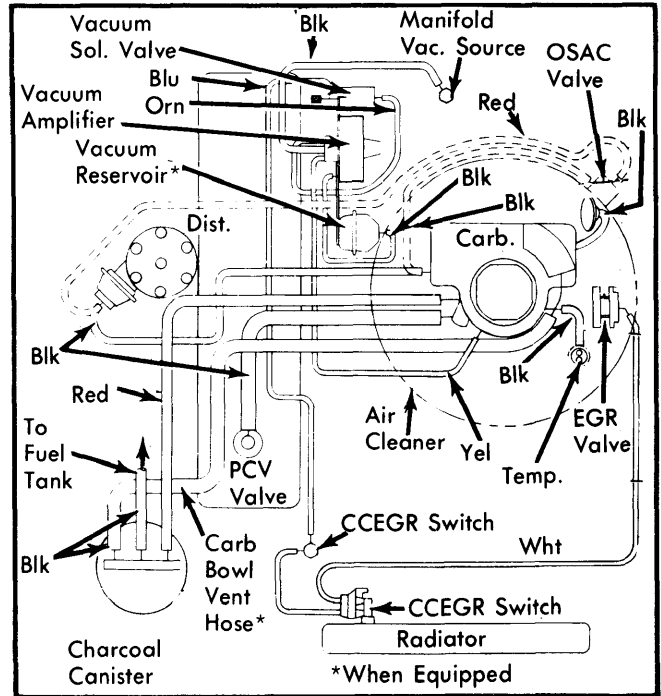
Fig. 2 225", Federal & Canada, All Trans.
