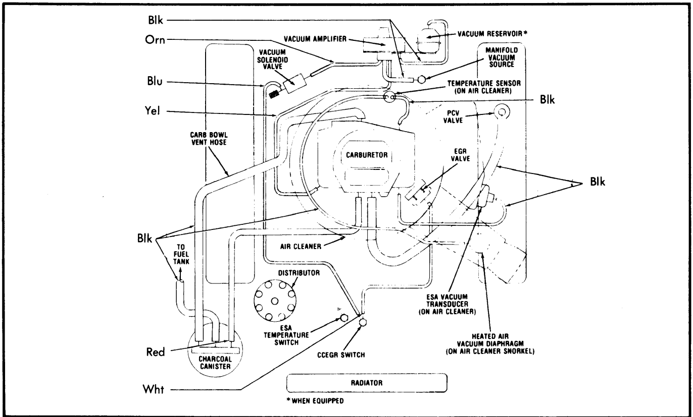
Fig. 15 400" 4-Bbl., Exc. Chrysler, Federal, with ELB and Catalyst, Auto. Trans.
