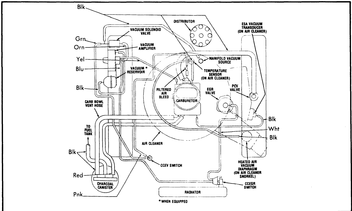
Fig. 10 360" 2-Bbl., Canada with ELB, Catalyst (Optional), Auto. Trans.
