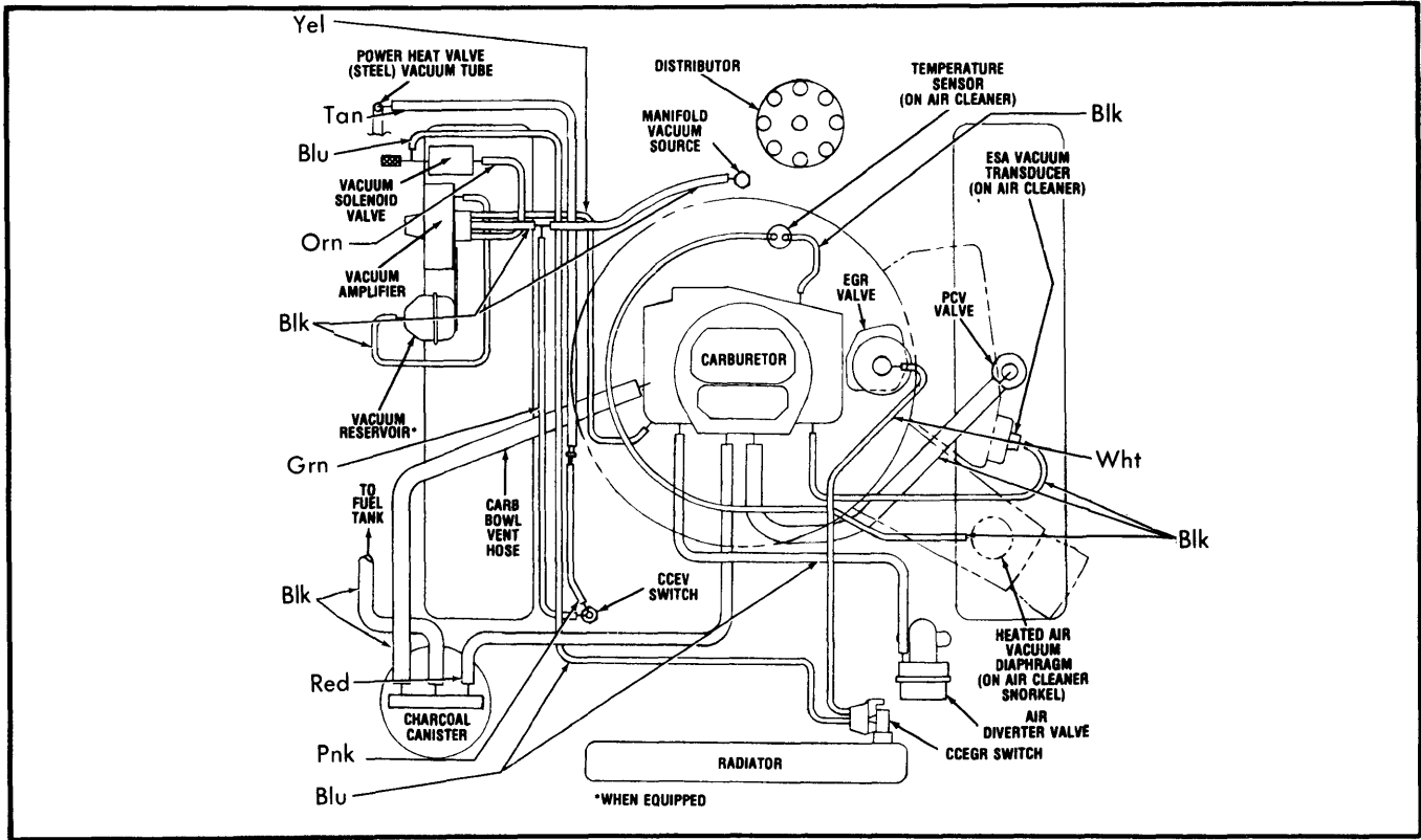
Fig. 9 318" 4-Bbl, Canada with ELB and Air Pump, Auto. Trans.
