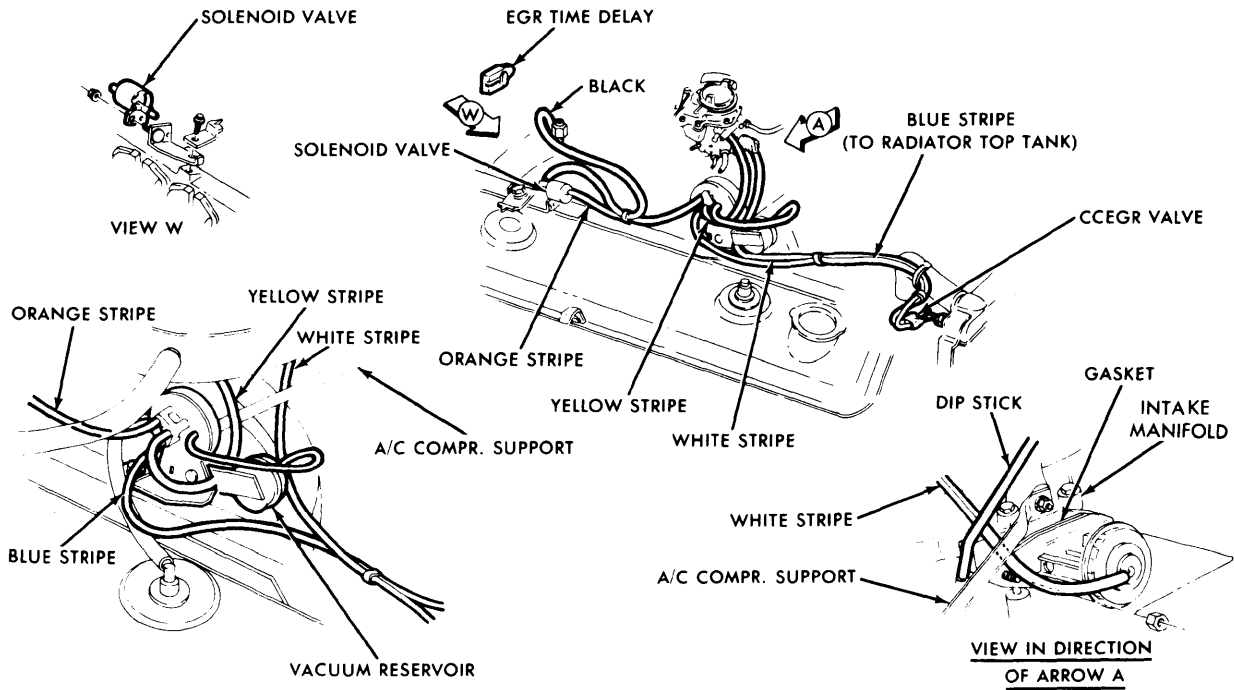
EGR SYSTEM 225" (CALIFORNIA)
