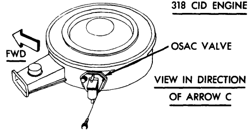
318 CID ENGINE
