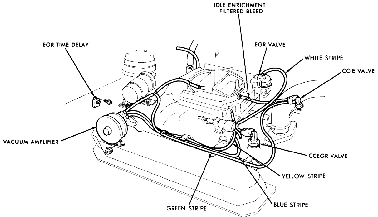
EGR SYSTEM 360" 4-BBL. AUTO TRANS. (CALIFORNIA)
