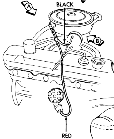
225 CID ENGINES
