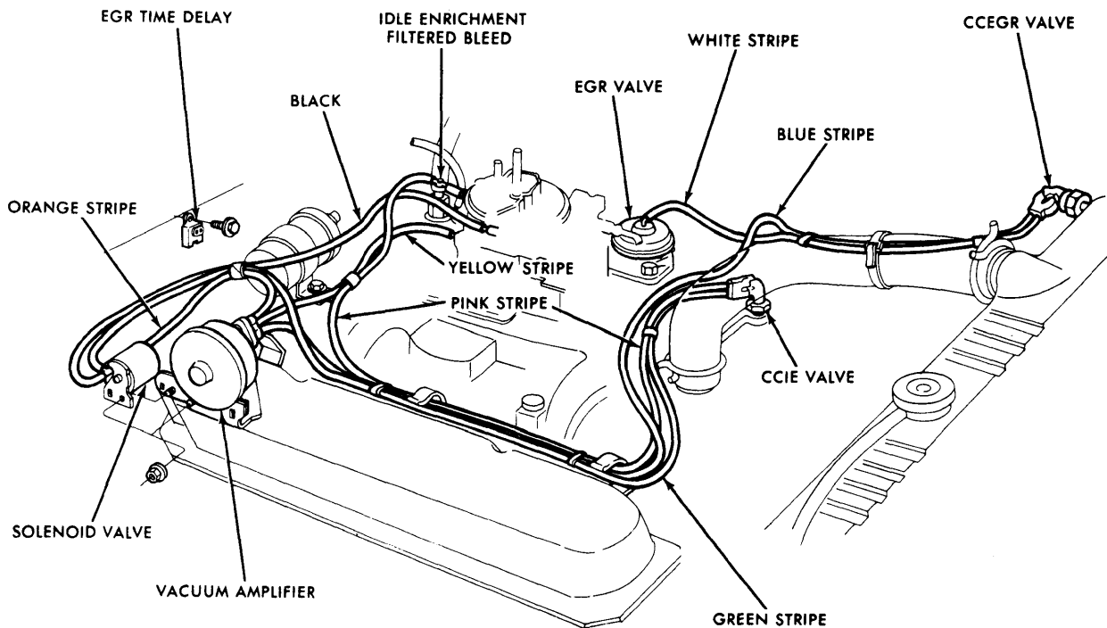
EGR SYSTEM 360" 2-BBL. AUTO. TRANS. (FEDERAL)
