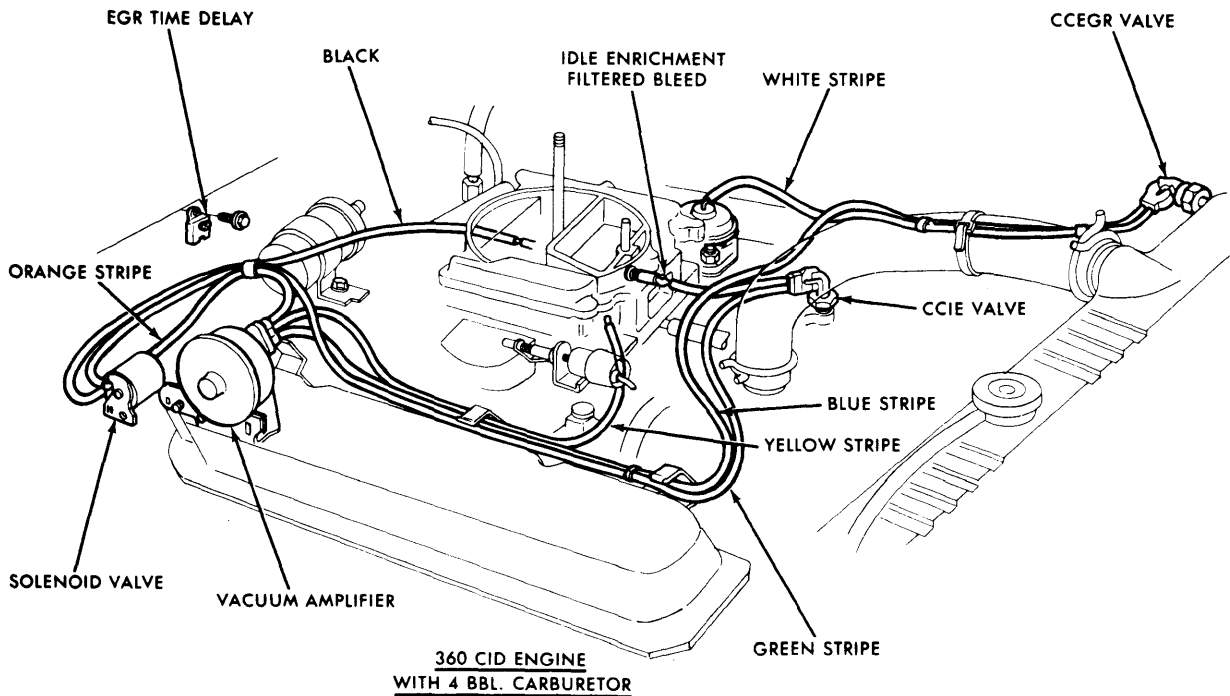
EGR SYSTEM 360" HI-PERFORMANCE (FEDERAL)
