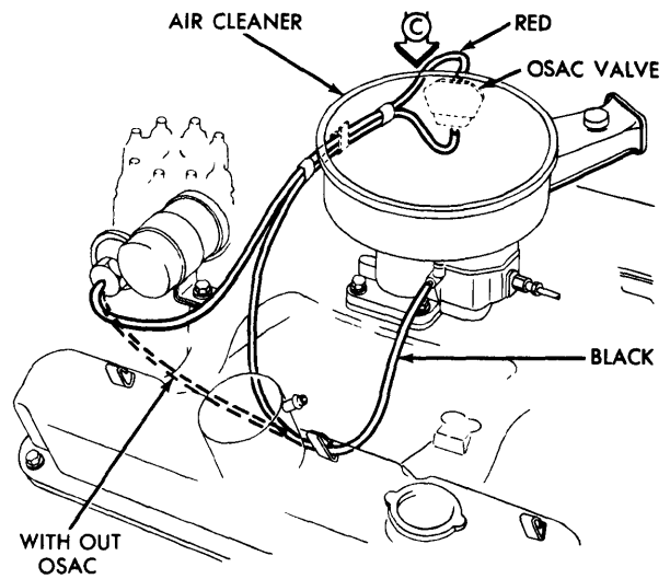
318 CID ENGINE
