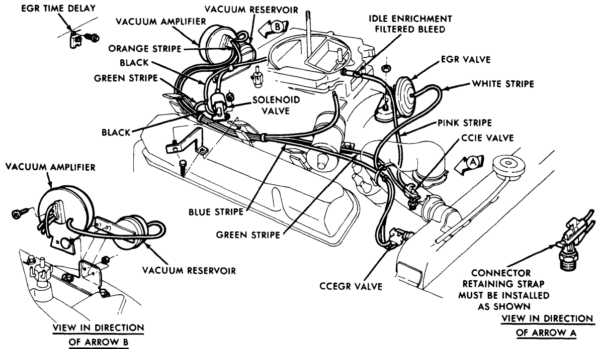
EGR SYSTEM 400" & 440" (CALIFORNIA)
