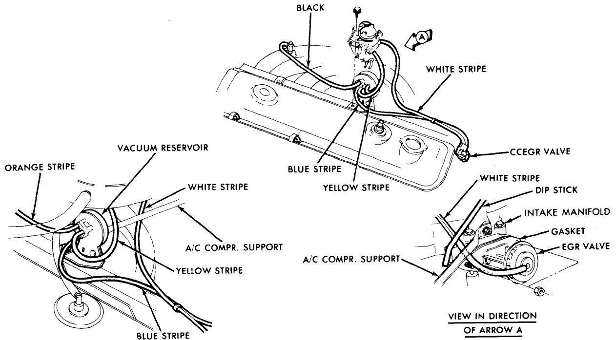
EGR SYSTEM 225" (FEDERAL)
