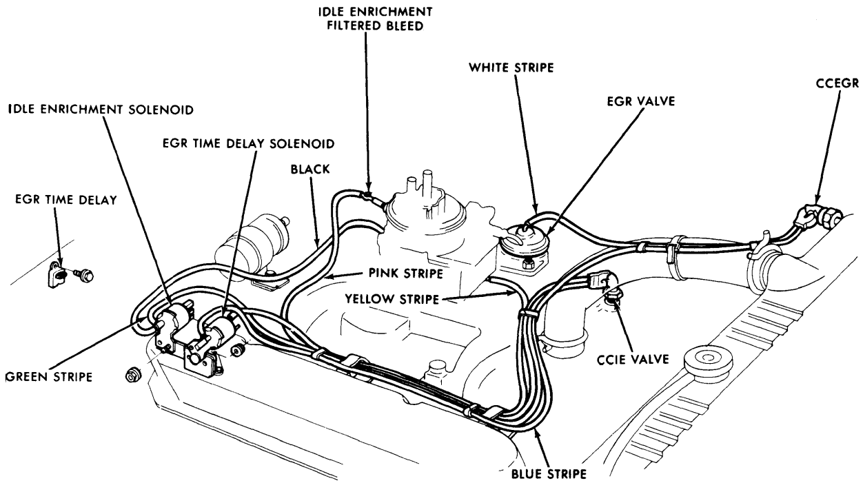
EGR SYSTEM 318" AUTO. TRANS. (FEDERAL)
