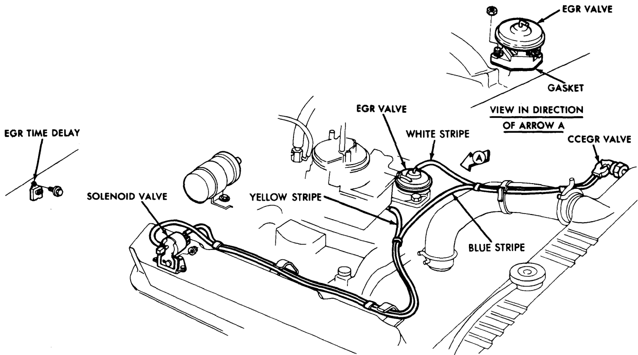
EGR SYSTEM 318" MAN. TRANS. (FEDERAL)
