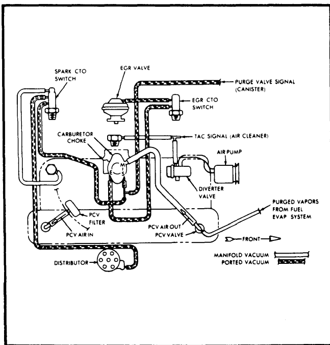
Fig. 3 232" 6-Cyl. 1-Bbl. Federal All Trans. (Pacer, Spirit, Concord)
