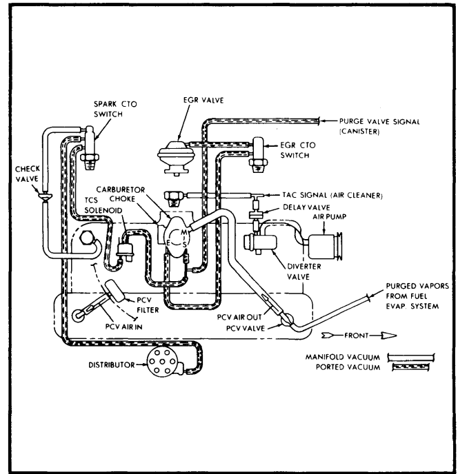
Fig. 6 258" 6-Cyl. 2-Bbl. Calif. Auto. Trans. (Pacer, Spirit, Concord)
