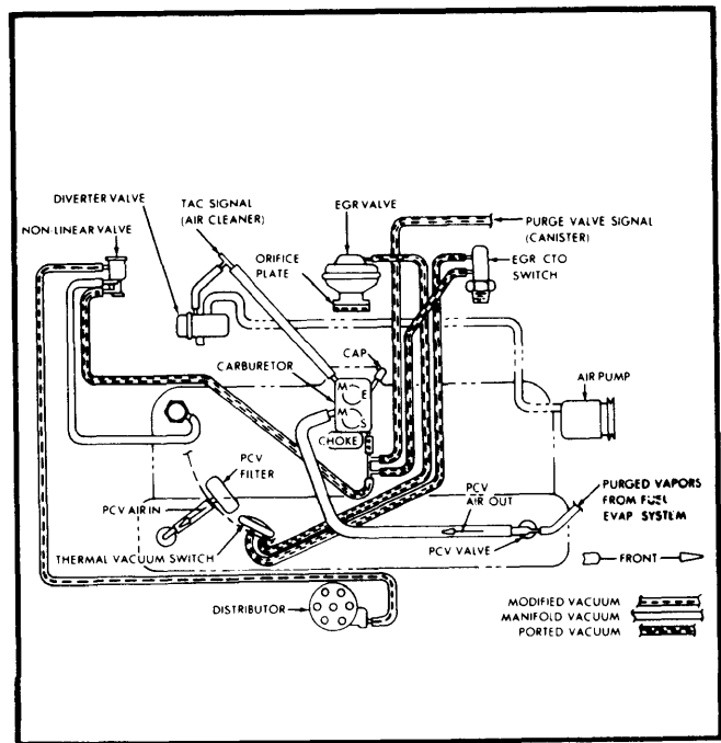
Fig. 4 258" 6-Cyl. 2-Bbl. Federal Man. Trans. (Pacer, Spirit, Concord)
