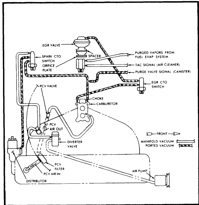
Fig. 2 121" 4-Cyl. 2-Bbl. Calif. Auto. Trans. (Spirit, Concord)
