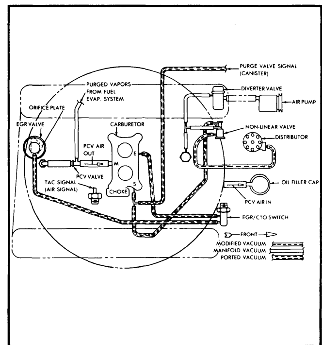
Fig. 8 304" V8 2-Bbl. Federal Auto. Trans. (Pacer, Spirit, Concord)
