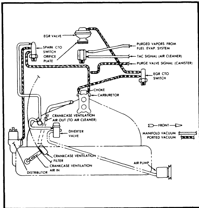
Fig. 1 121" 4-Cyl. 2-Bbl. Federal All Trans (Spirit, Concord)
