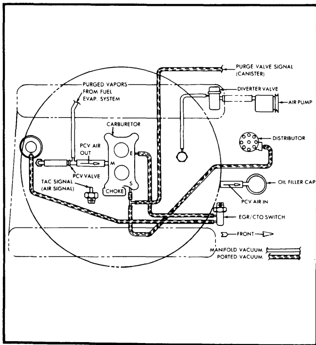
Fig. 7 304" V8 2-Bbl. Federal Man. Trans. (Spirit)
