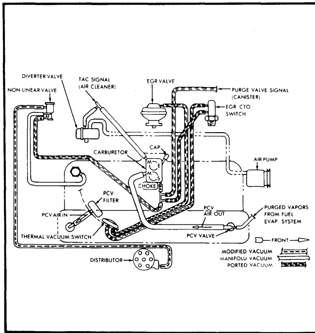
Fig. 5 258" 6-Cyl. 2-Bbl. Federal Auto. Trans. (Pacer, Spirit, Concord)
