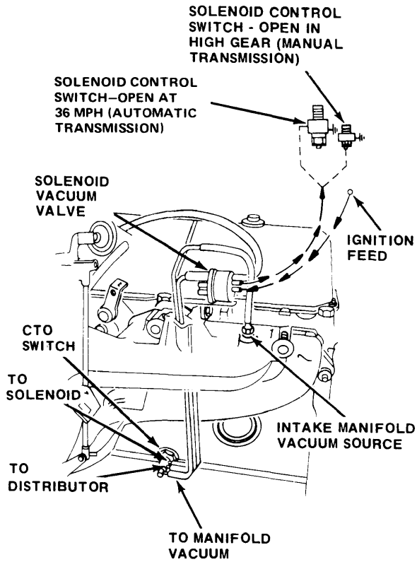
TCS SYSTEM (6-CYL.)
