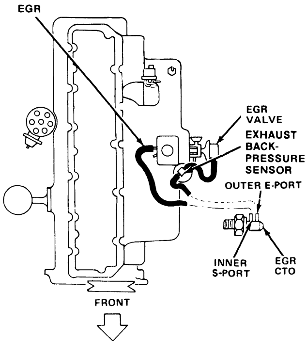
EGR SYSTEM (6 CYL.)
