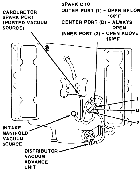
TCS SYSTEM (6-CYL.)
