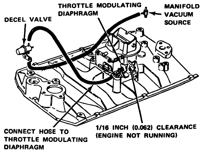
THROTTLE MODULATING SYSTEM (DECAL VALVE)
