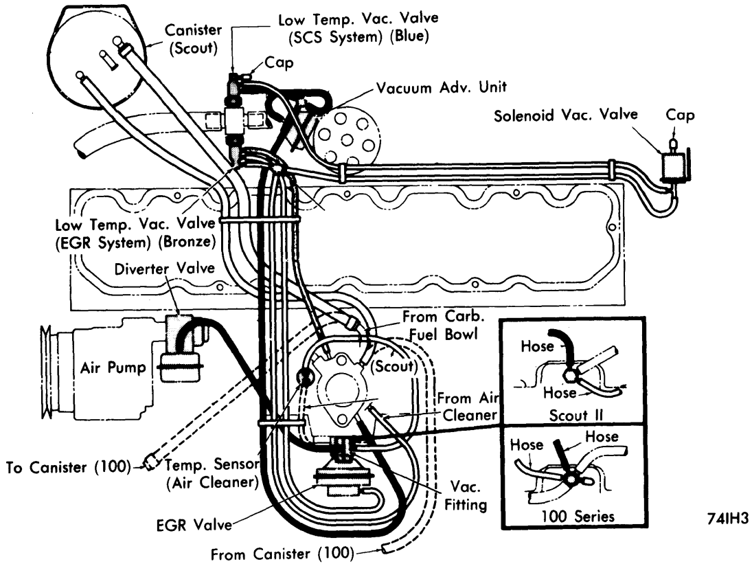
1974 IHC 258" 6-CYL. (EXCEPT CALIF.)
