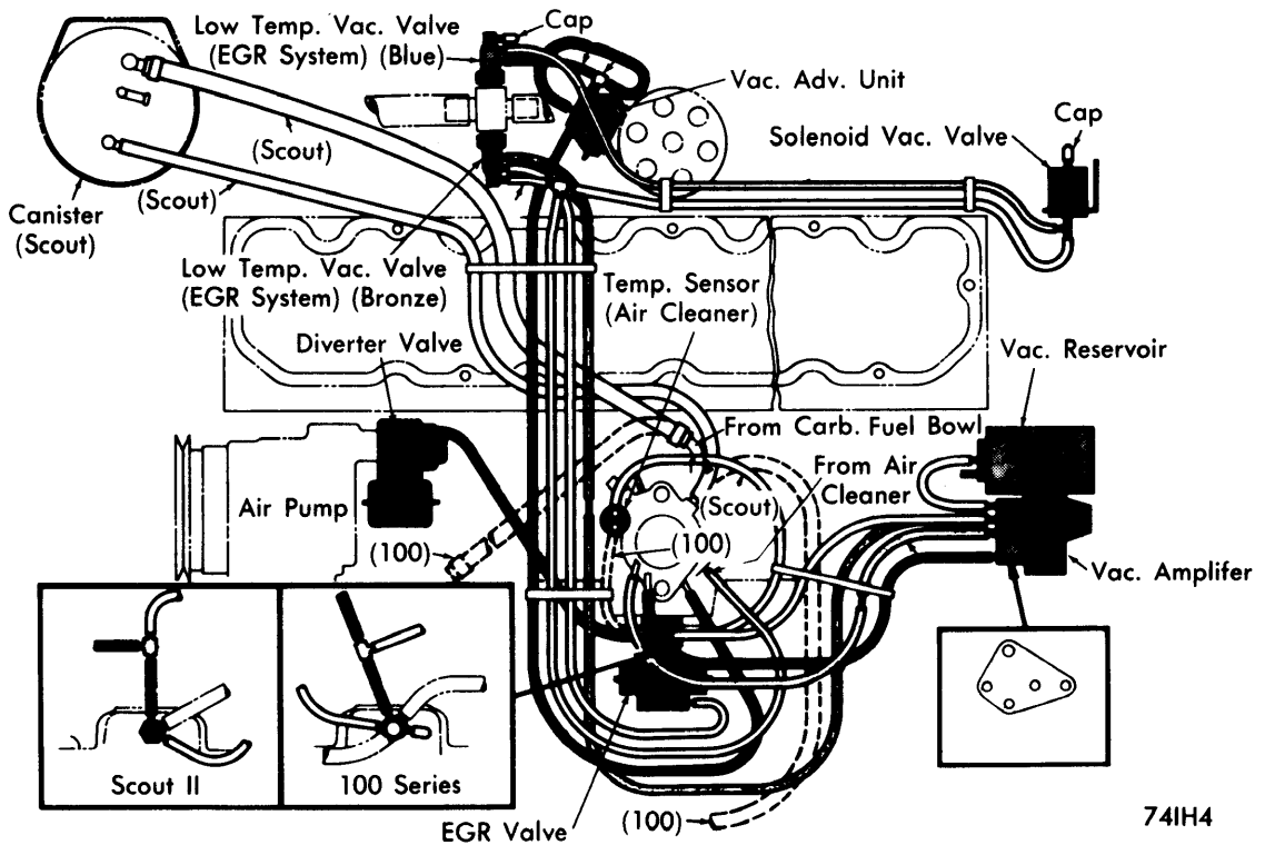
1974 IHC 258" 6-CYL. (CALIF. ONLY)
