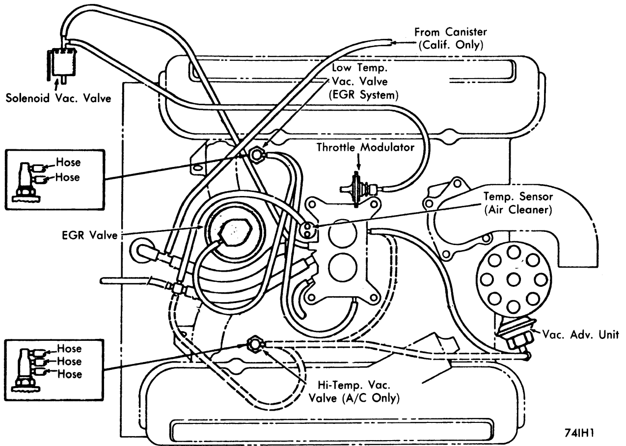
1974 IHC 304" & 345" V8 (200 & MHC MODELS WITH 2210 CARBURETOR)
