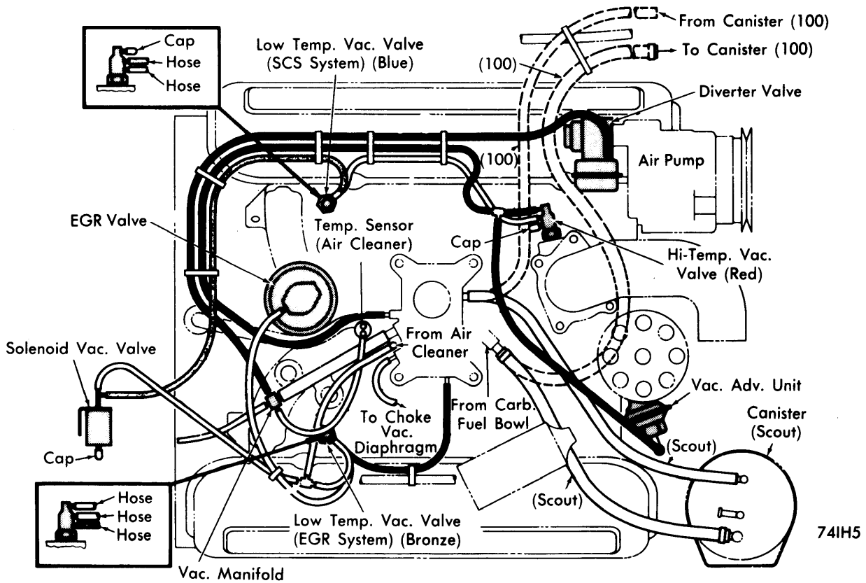
1974 IHC 304" & 345" V8 (EXCEPT CALIF.)
