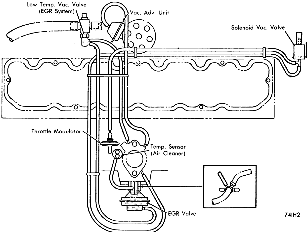
1974 IHC 258" 6-CYL. (200 MODELS)
