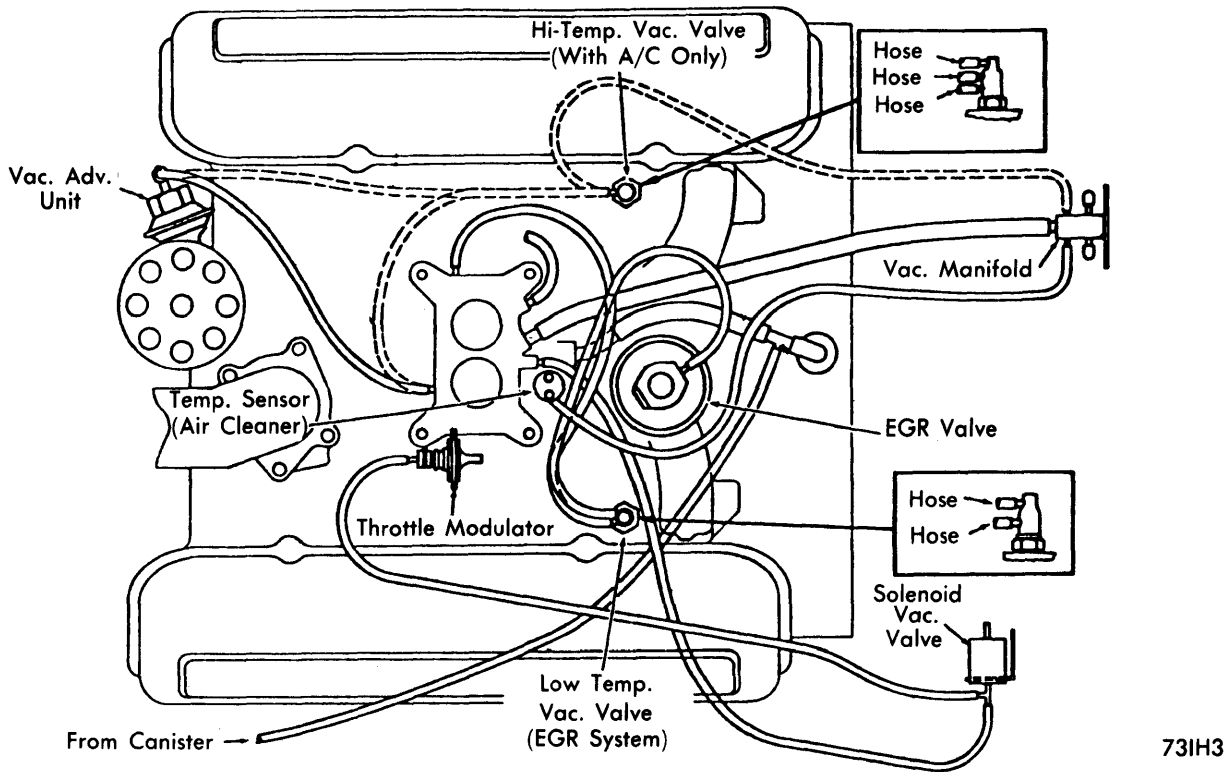
1972-73 IHC 304" & 345" V8 (WITH THROTTLE MODULATOR)
