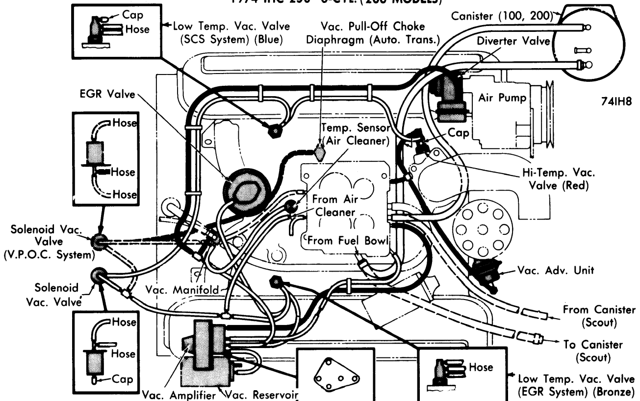
1974 IHC 345" & 392" V8 (CALIF. ONLY)
