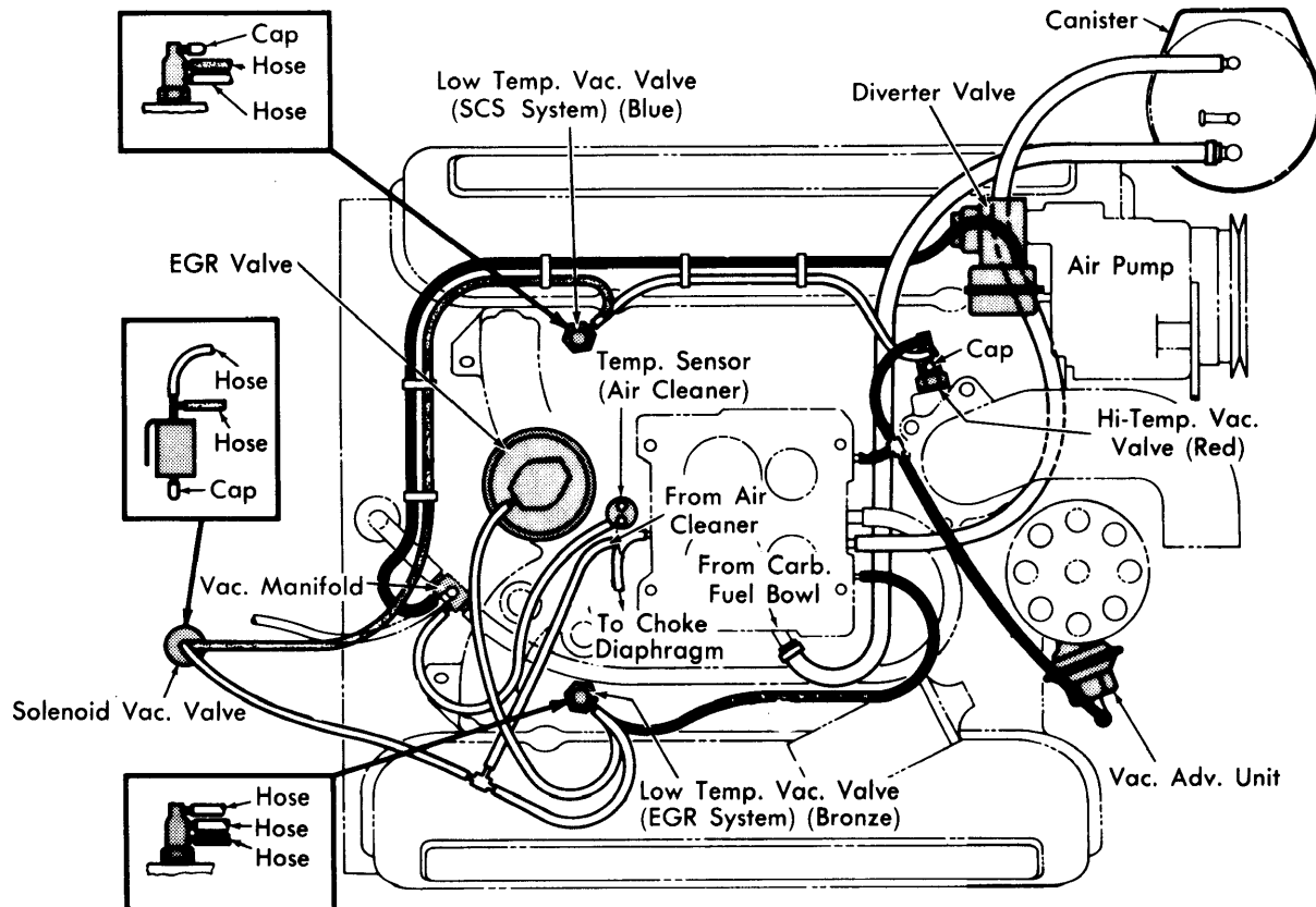
1974 IHC 392" V8 (EXCEPT CALIF.)
