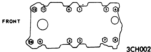
307" & 350" INTAKE MANIFOLD TIGHTENING SEQUENCE
