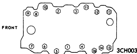
454" INTAKE MANIFOLD TIGHTENING SEQUENCE
