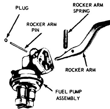
SEALED FUEL PUMP (TYPICAL)
