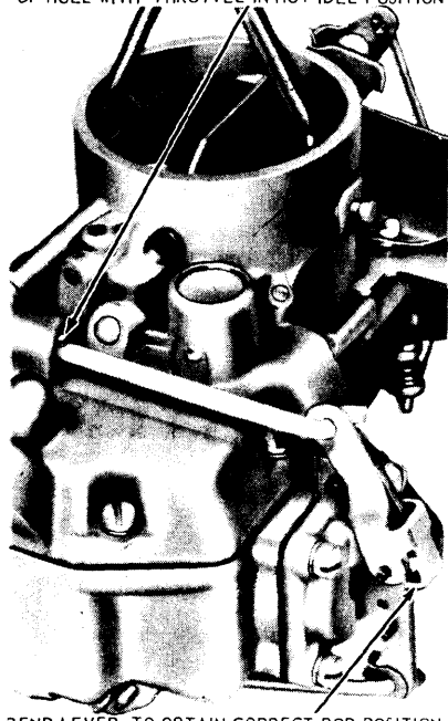
BEND LEVER TO OBTAIN CORRECT ROD POSITION
