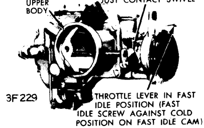
3F229 THROTTLE LEVER IN FAST IDLE POSITION (FAST IDLE SCREW AGAINST COLD POSITION ON FAST IDLE CAM) CHOKE VALVE PULL-DOWN ADJUSTMENT (MODEL 1100 CARBURETORS)
