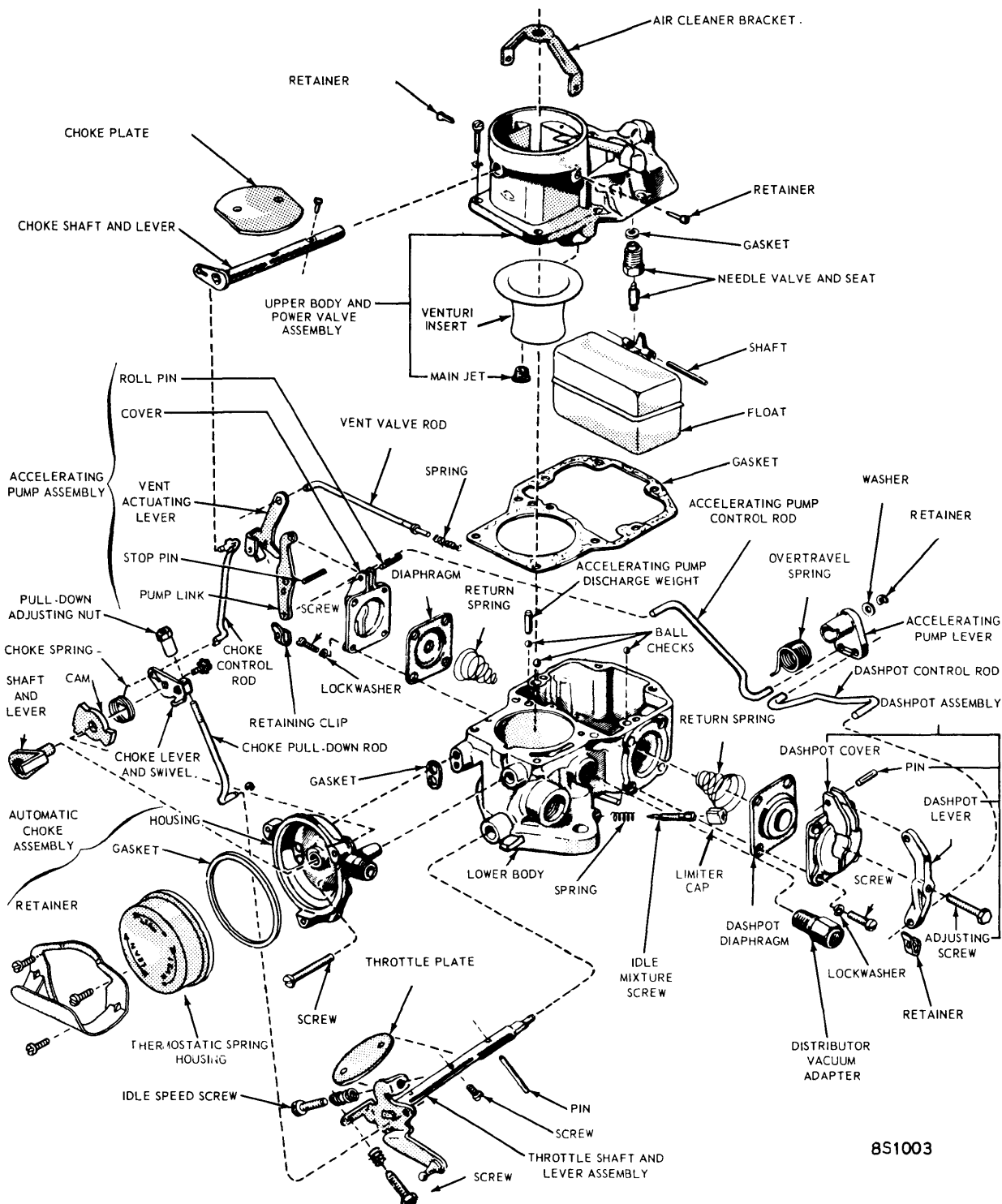
FORD SINGLE BARREL CARBURETOR ASSEMBLY (SPRING TYPE AUTOMATIC CHOKE) MODEL 1100 (COMET, FALCON, FAIRLANE, MUSTANG)
