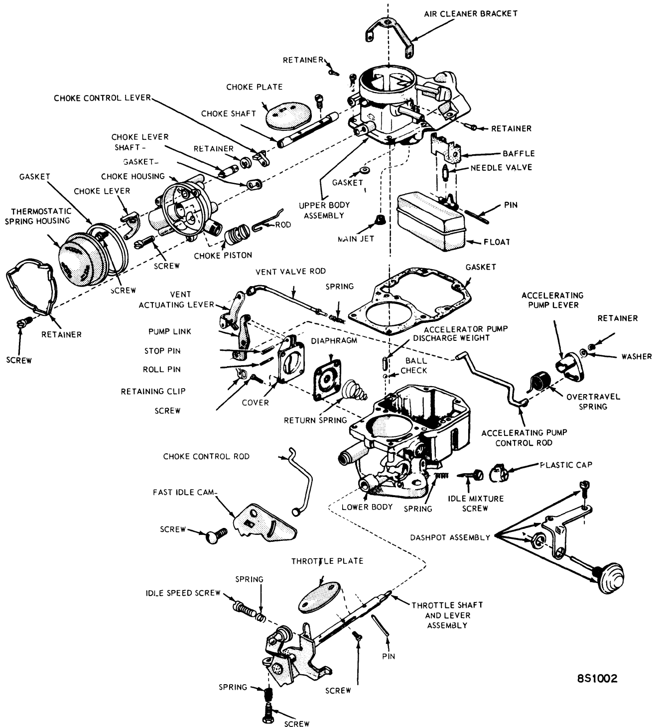
FORD SINGLE BARREL CARBURETOR ASSEMBLY (PISTON TYPE AUTOMATIC CHOKE) MODEL 1101 (FORD CUSTOM & GALAXIE)
