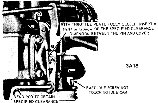
ACCELERATING PUMP ADJUSTMENT
