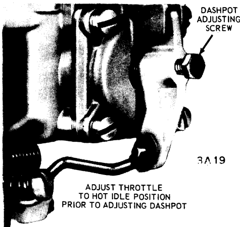
ANTI-STALL DASHPOT ADJUSTMENT (INTERNAL TYPE)
