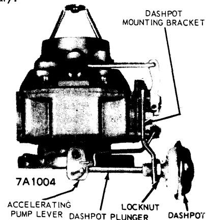
ANTI-STALL DASHPOT ADJUSTMENT (EXTERNAL TYPE)
