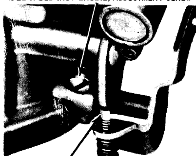
FAST IDLE (COLD ENGINE) ADJUSTMENT SCREW
