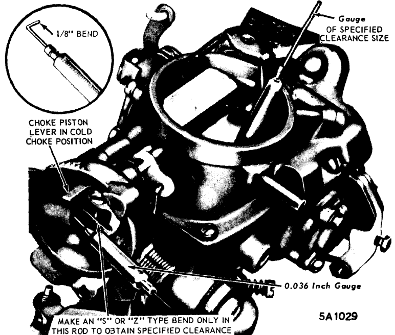
CHOKE VALVE PULL-DOWN ADJUSTMENT (MODEL 1101 CARBURETORS)
