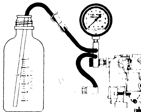
CHECKING FUEL PUMP VOLUME
