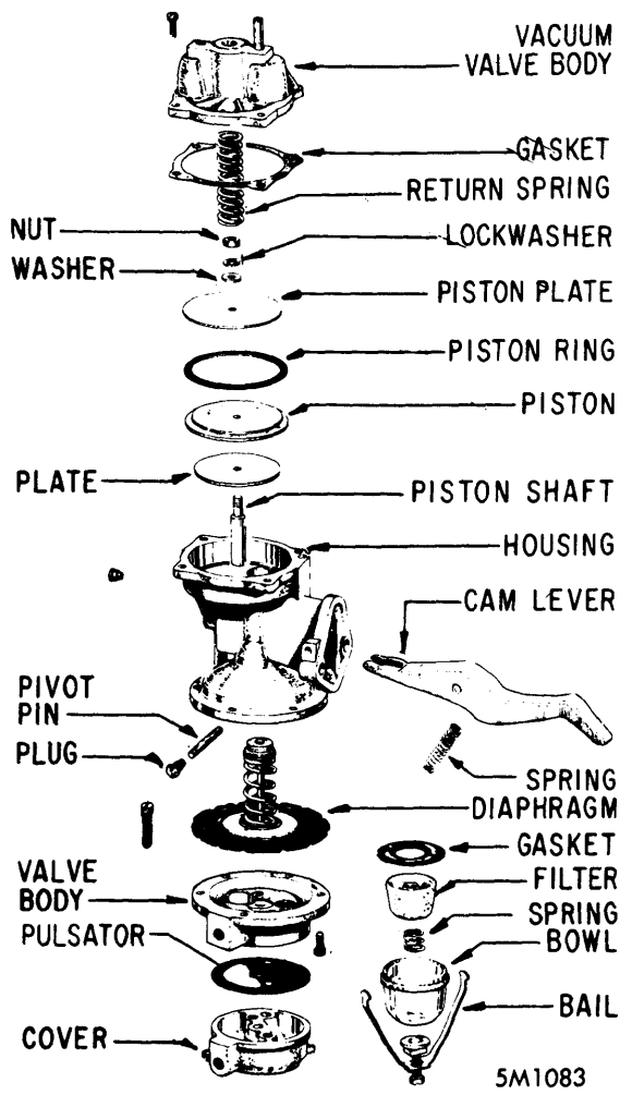
FUEL & VACUUM PUMP (TYPICAL) (CARTER SHOWN)
