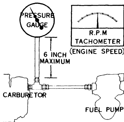
CHECKING FUEL PUMP PRESSURE
