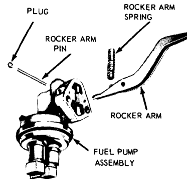
SEALED FUEL PUMP (TYPICAL)
