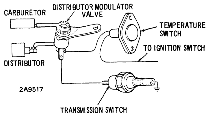
TRANSMISSION REGULATED SPARK CONTROL SYSTEM (TRS)
