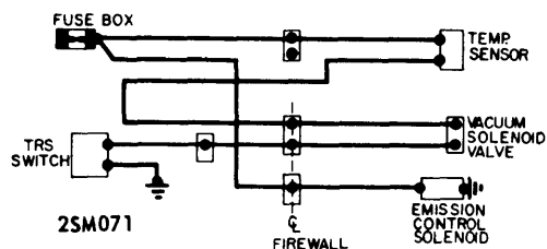
TRANSMISSION REGULATED SPARK CONTROL ELECTRICAL SCHEMATIC
