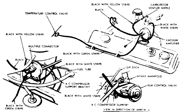
EGR VENTURI SYSTEM (6 CYL.)
