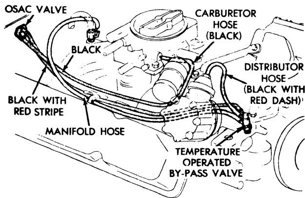
BY-PASS VALVE (ALL ENGINES)
