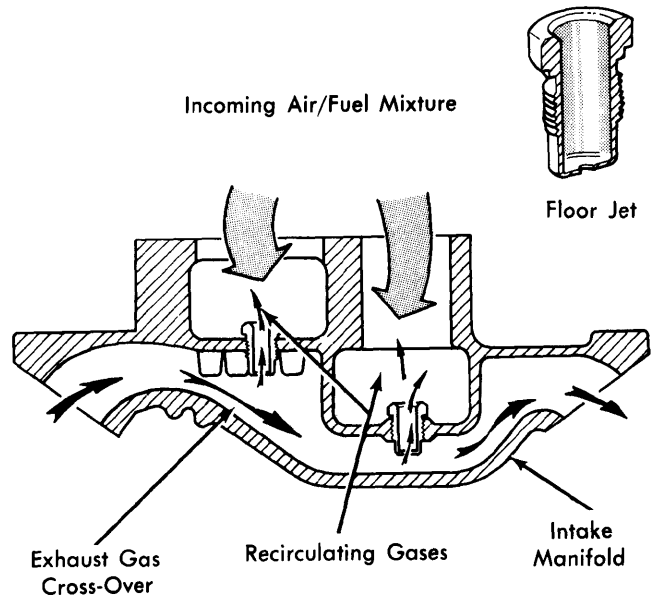
EGR FLOOR JET SYSTEM (1972-73) 340" & 400" 4-BARREL ONLY
