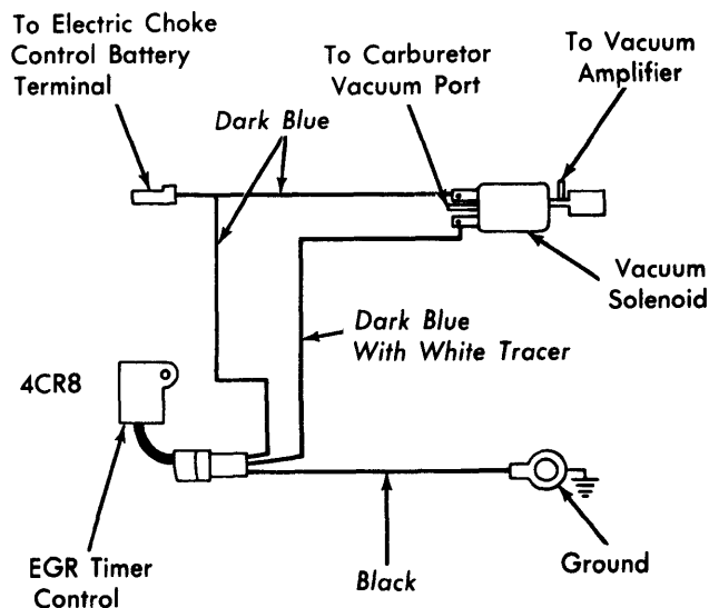
EGR TIME DELAY SYSTEM
