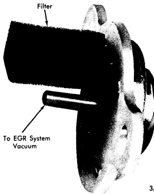
TEMPERATURE CONTROL VALVE (PRIOR TO MARCH 15, 1973)
