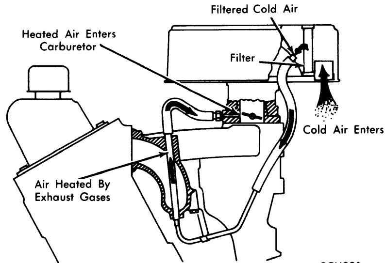
ANTI-ICING DEVICE (1969 ONLY)
