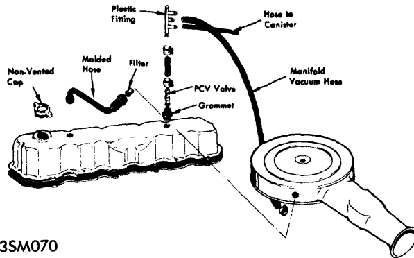
1973 PCV SYSTEM (6 CYL.)
