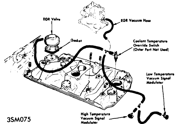
1973 EGR SYSTEM (V-8)
