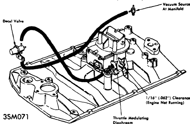
1973 VACUUM THROTTLE MODULATING SYSTEM
