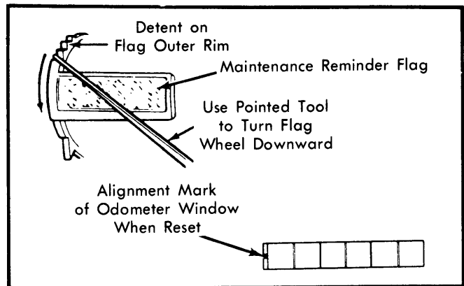
Fig. 2 General Motors Maintenance Reminder Flag Resetting Procedure
