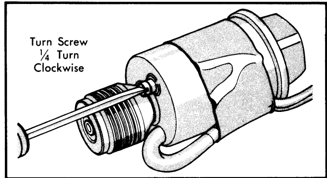
Fig. 1 Resetting Maintenance Reminder Switch American Motors
