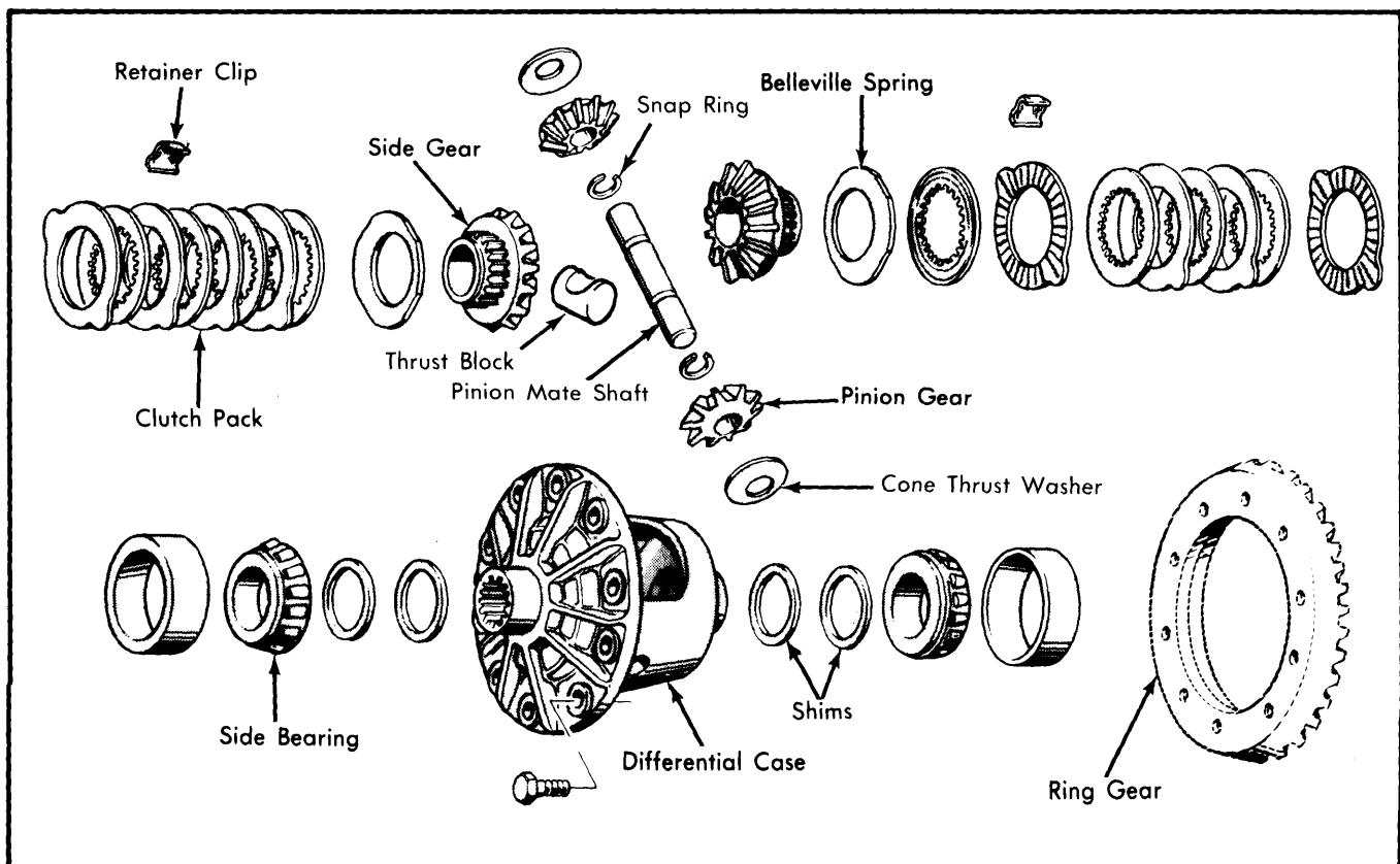
Fig. 1 Exploded View of Spicer (Dana) Trac-Lok Differential Assembly
