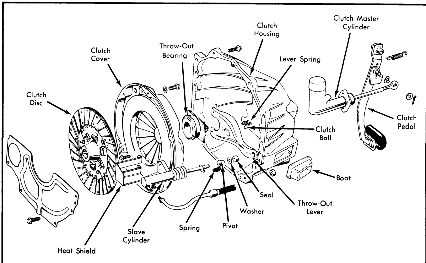
Fig. 1 Exploded View of Hydraulic Clutch Assembly ("CJ" & Scrambler With 4-Cylinder Engine)
