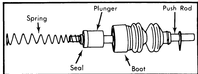
Fig. 3 Exploded View of Clutch Slave Cylinder
