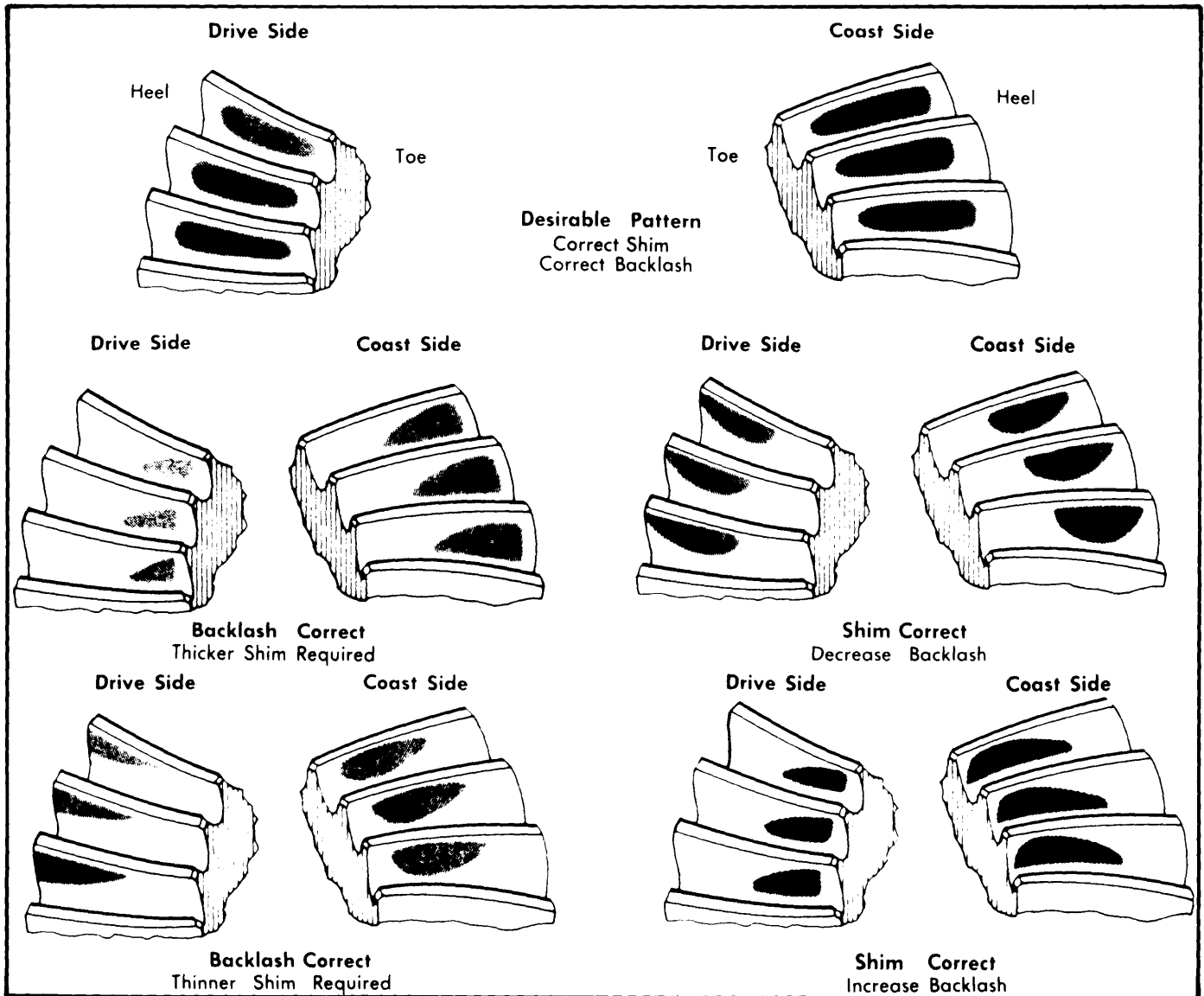
Fig. 1 Drive Axle Gear Tooth Pattern
