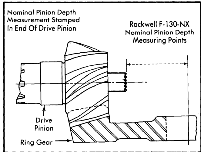
Fig. 6 Nominal Pinion Depth Measuring Points for Rockwell F-130-NX Single Speed Drive Axle
