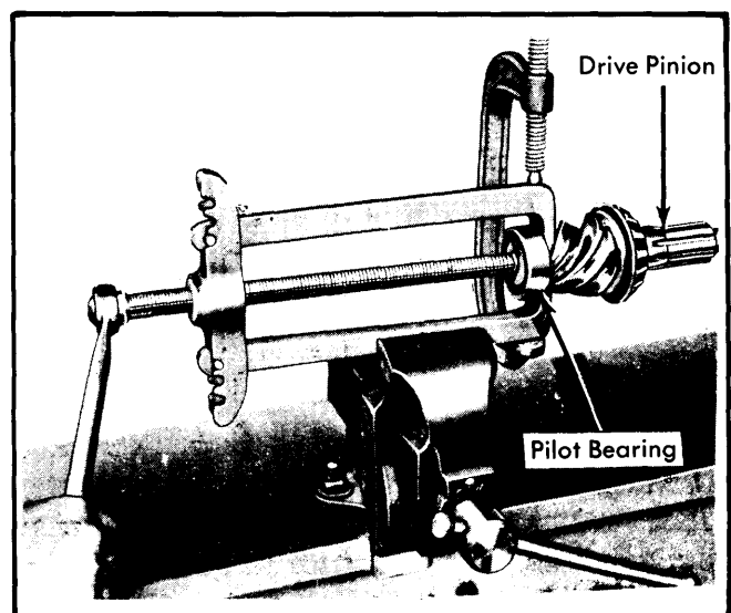
Fig. 2 Drive Pinion Pilot Bearing Removal
