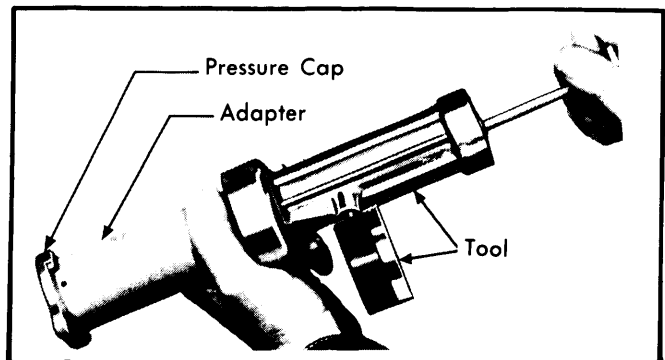
Fig. 2 Correct Procedure to Test Radiator Pressure Cap
