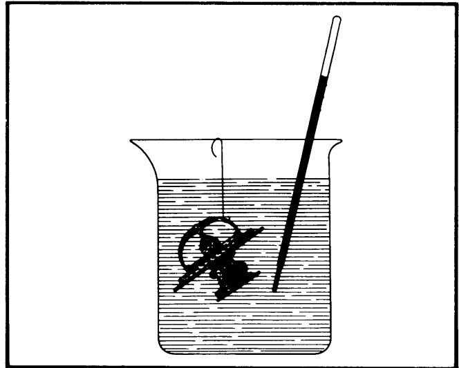
Fig. 1 Correct Procedure to Test Thermostat
