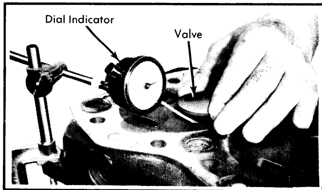
Fig. 4 Measuring Valve Stem to Guide Clearance
