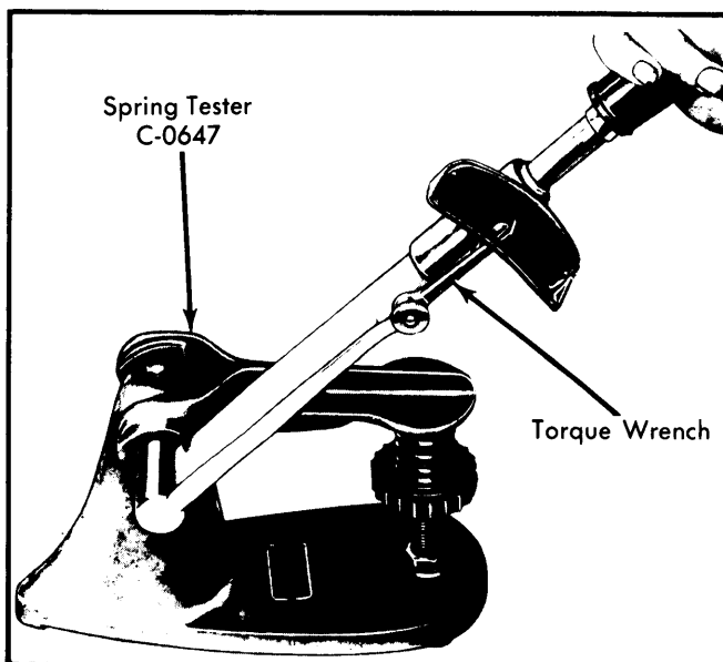
Fig. 5 Testing Valve Spring
