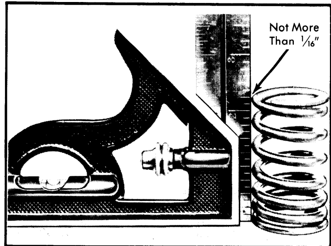
Fig. 6 Valve Spring Squareness Test
