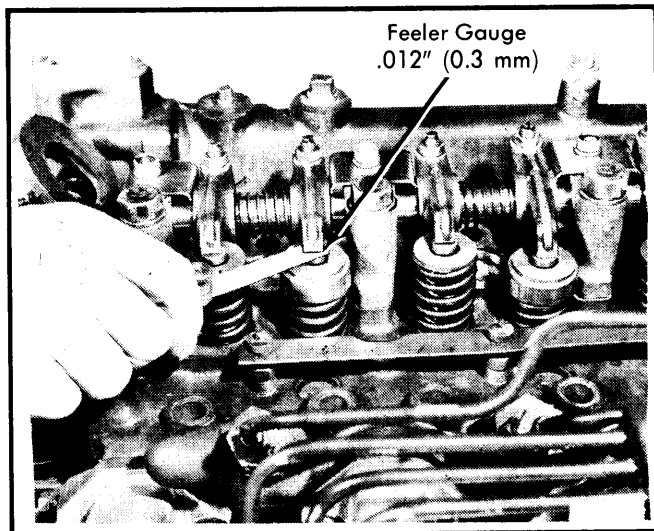
Fig. 8 Valve Adjustment
