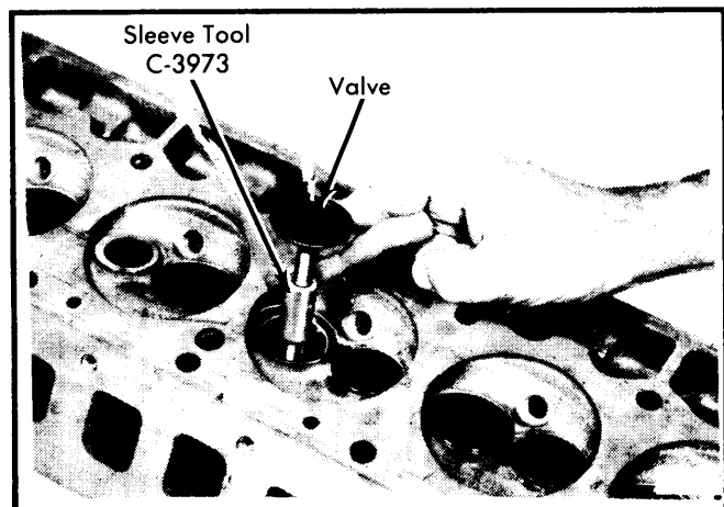
Fig. 3 Installation of Sleeve Tool C-3973
