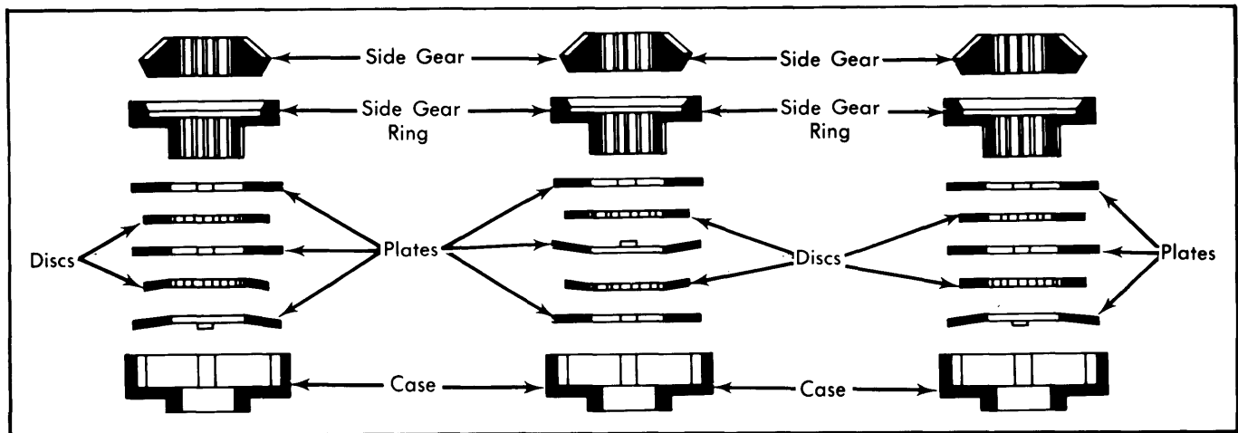
Fig. 2 Three Views Showing Typical Clutch Pack Arrangements (Not All Combinations are Shown)
