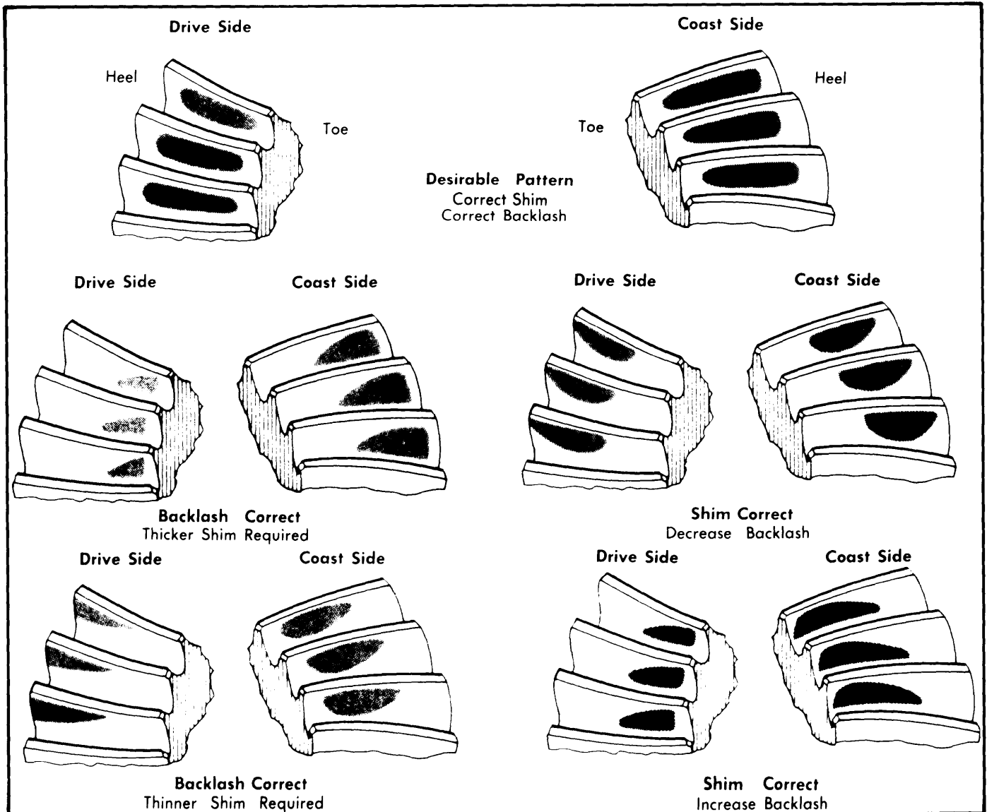
Fig. 1 Drive Axle Gear Tooth Patterns
