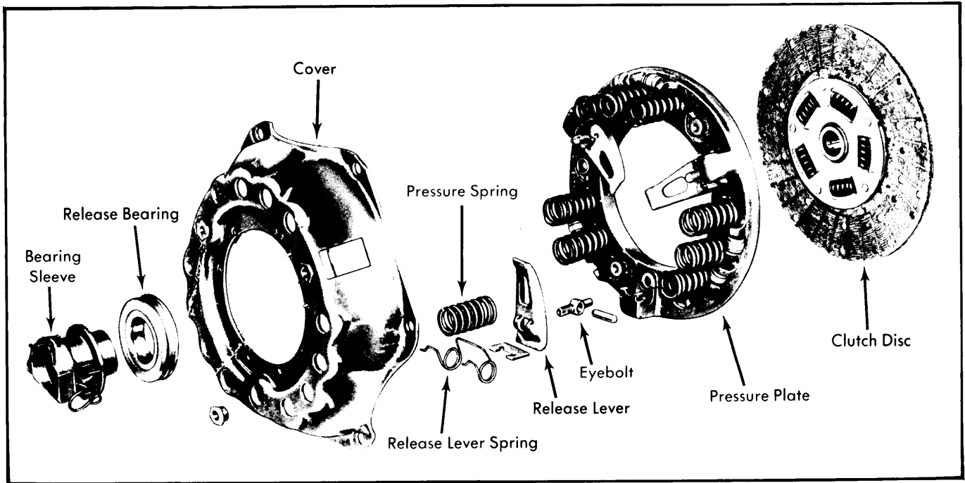
Fig. 2 Exploded View of Borg & Beck Type Clutch Assembly
