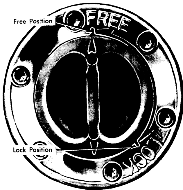
Fig. 1 Front View of Dana/Spicer Locking Hub
