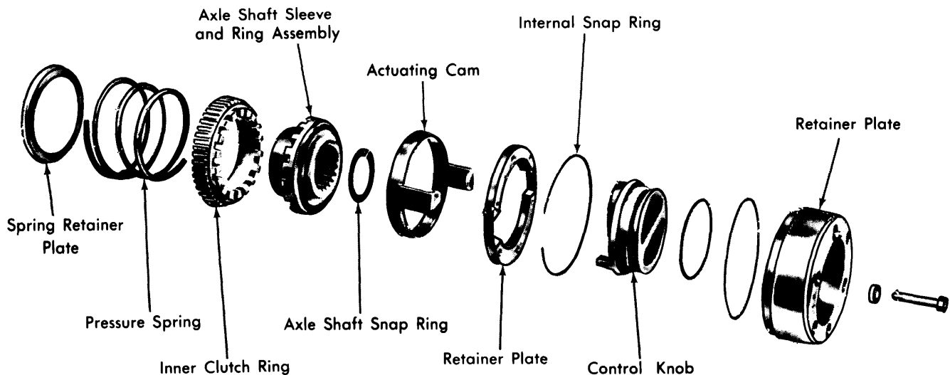
Fig. 2 Exploded View of Dana/Spicer 6 Bolt Locking Hub
