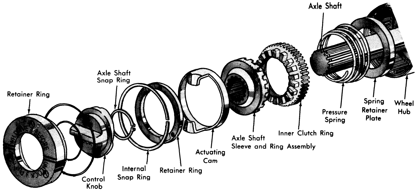
Fig. 3 Exploded View of Dana/Spicer 3 Bolt Locking Hub
