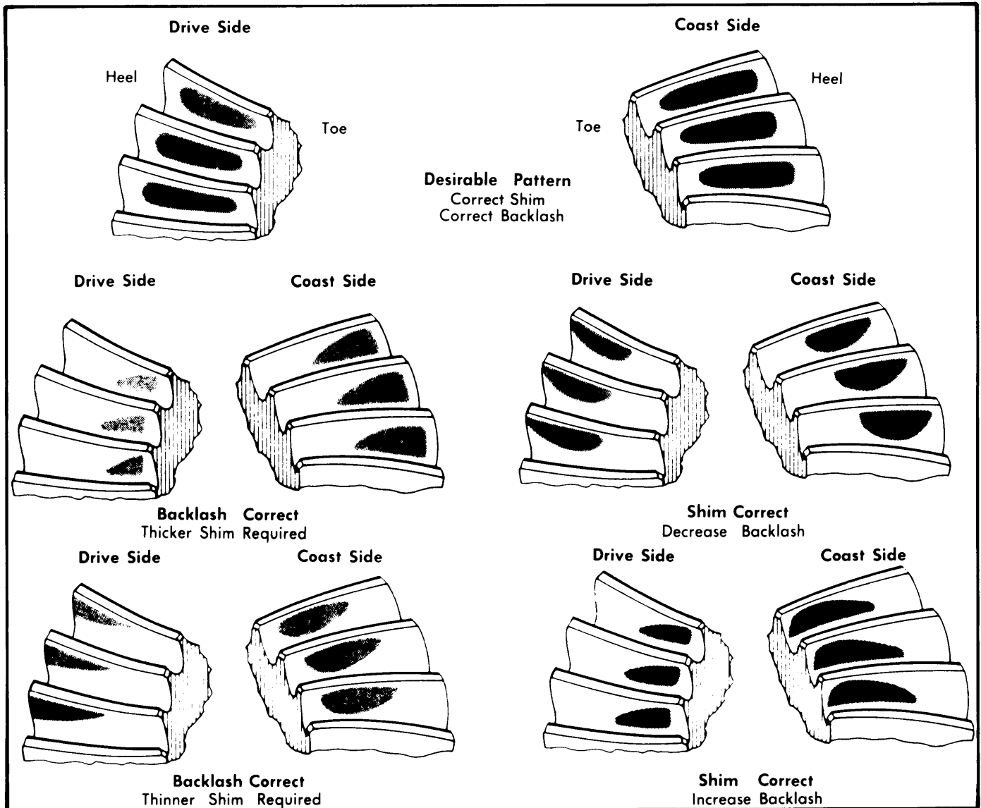
Fig. 1 Drive Axle Gear Tooth Patterns
