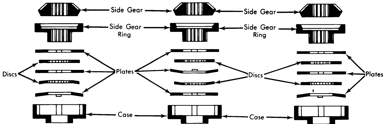
TYPICAL CLUTCH PACK ARRANGEMENTS (NOT ALL COMBINATIONS ARE SHOWN)
