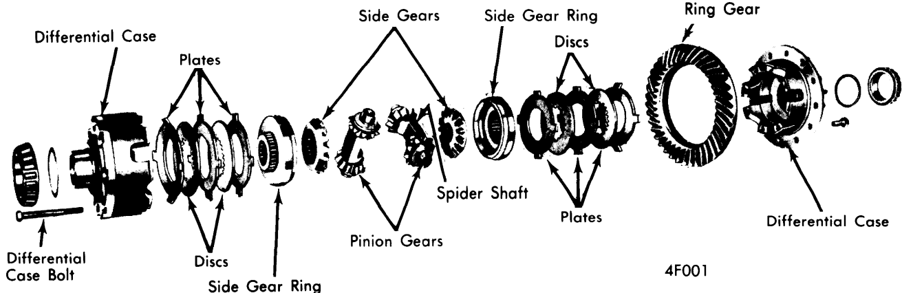
POWER-LOK DIFFERENTIAL ASSEMBLY
